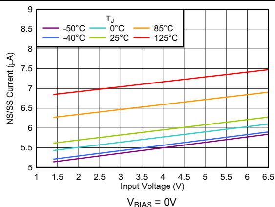
5-32. NR/SS Current vs Input Voltage
