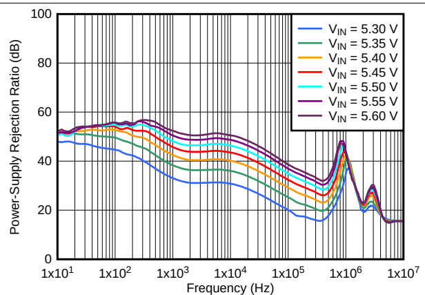
FIG 49. PSRR vs Frequency and V_{IN} for V_{OUT} = 5.0 V at I_{OUT} = 3.0 A
