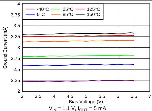
FIG 28. Quiescent Current vs Bias Voltage
