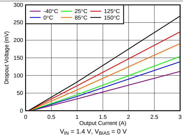
FIG 22. Dropout Voltage vs Output Current Without Bias
