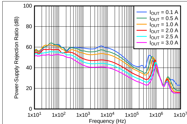
FIG 48. PSRR vs Frequency and I_{OUT} for V_{OUT} = 5.0 V
