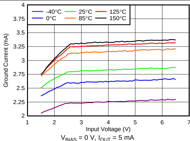
FIG 27. Quiescent Current vs Input Voltage
