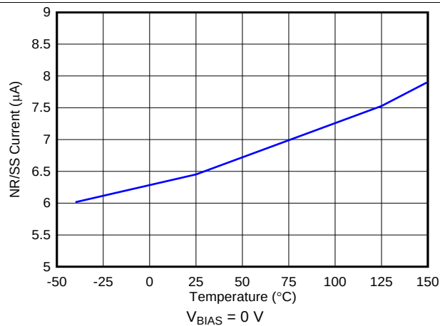
FIG 31. NR/SS Current vs Temperature
