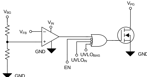
☒ 42. Simplified PG Circuit
