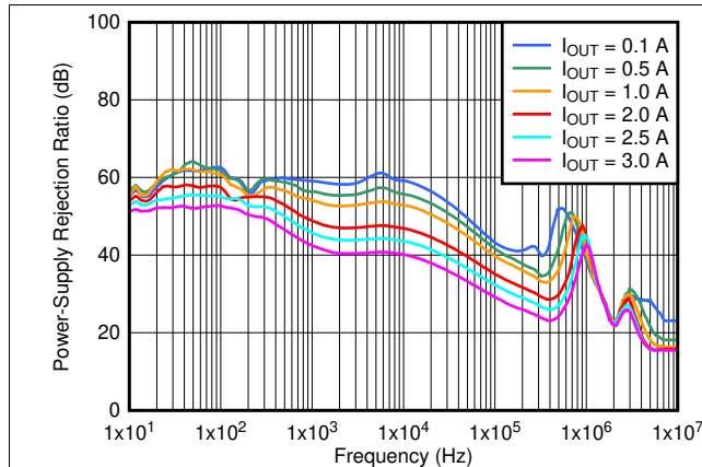
FIG 10. PSRR vs Frequency and I_{OUT} for V_{OUT} = 5.0 V
