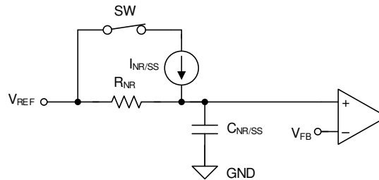
Figure 2. Simplified Soft-Start Circuit
