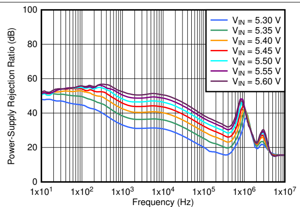
FIG 11. PSRR vs Frequency and V_{IN} for V_{OUT} = 5.0 V at I_{OUT} = 4.0 A
