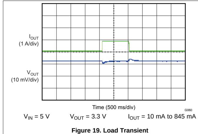
Figure 19. Load Transient
