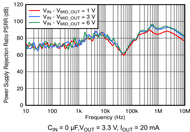
FIG 6-33. OUT PSRR vs Frequency and V_{\text{IN}}
