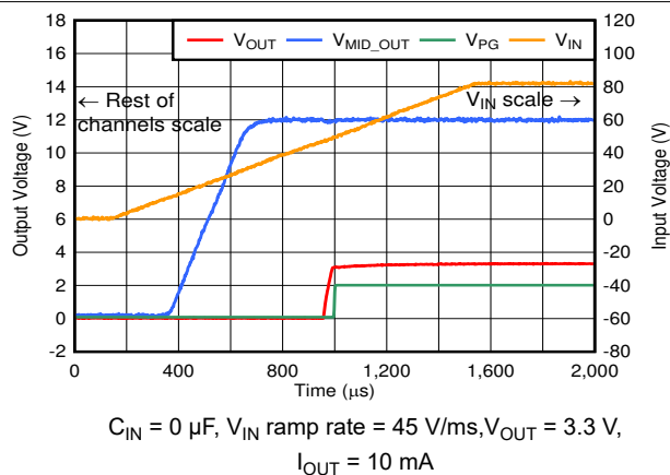
FIG 6-13. Slow Start-Up
