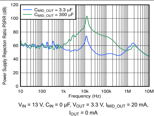
FIG 6-37. MID_OUT PSRR vs Frequency and C_{\text{MID\_OUT}}
