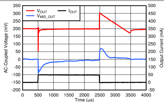
FIG 6-22. Load Transient
