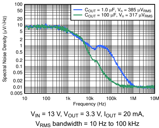
FIG 6-31. Spectral Noise Density vs Frequency and C_{\text{OUT}}
