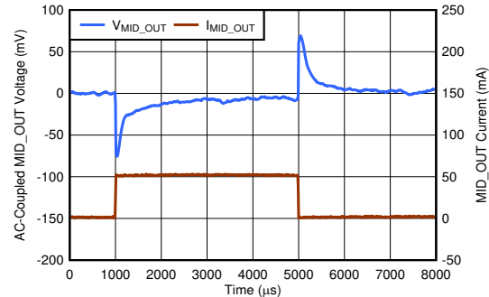
FIG 6-26. Load Transient (MID_OUT)
