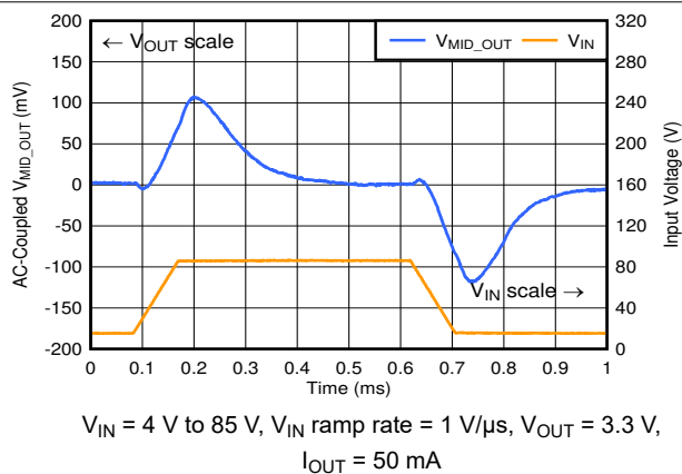
FIG 6-18. Line Transient ( V_{MID\_OUT} in Dropout)
