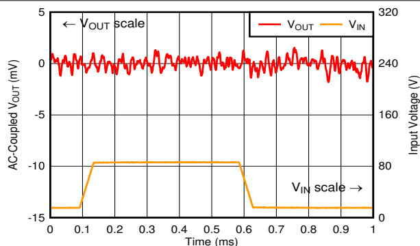
FIG 6-19. Line Transient ( V_{\text{MID\_OUT}} in Dropout)
