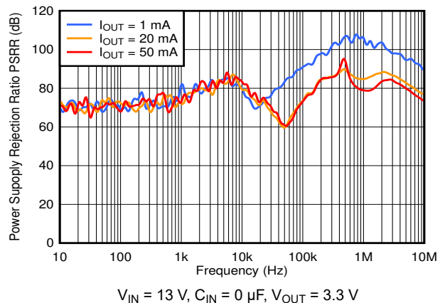
FIG 6-32. OUT PSRR vs Frequency and I_{\text{OUT}}
