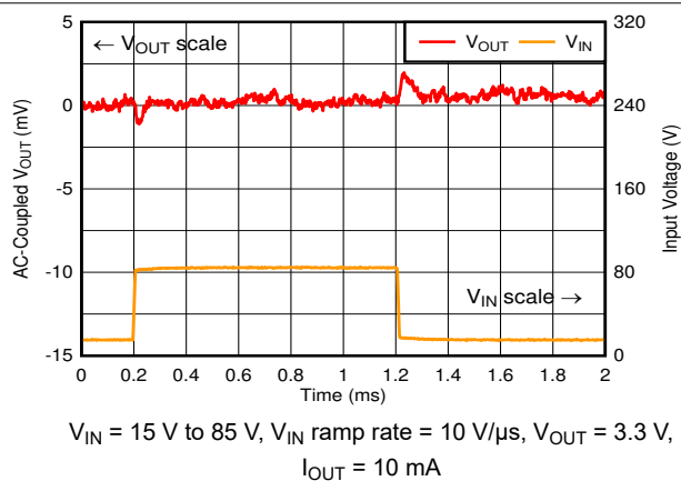
FIG 6-15. Line Transient
