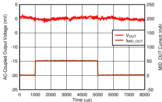
FIG 6-27. Load Transient (MID_OUT)
