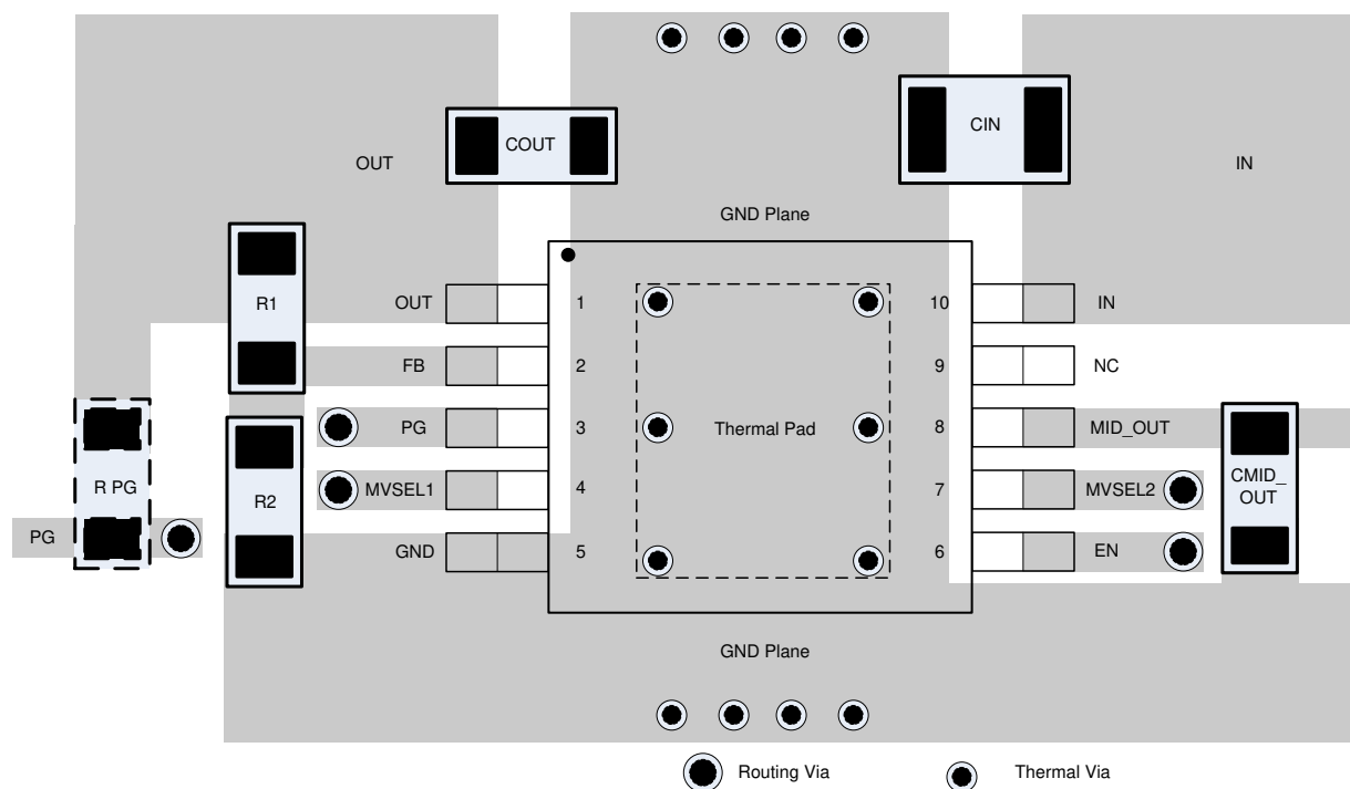
8-4. Adjustable Version Layout Example
