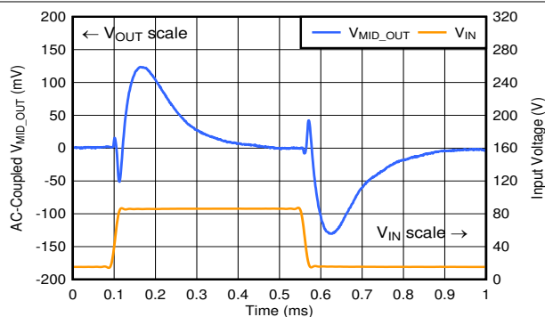
图 8-2. TPS7A43 Line Transient: 15 V to 85 V
