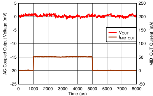
FIG 6-25. Load Transient (Rising Edge)
