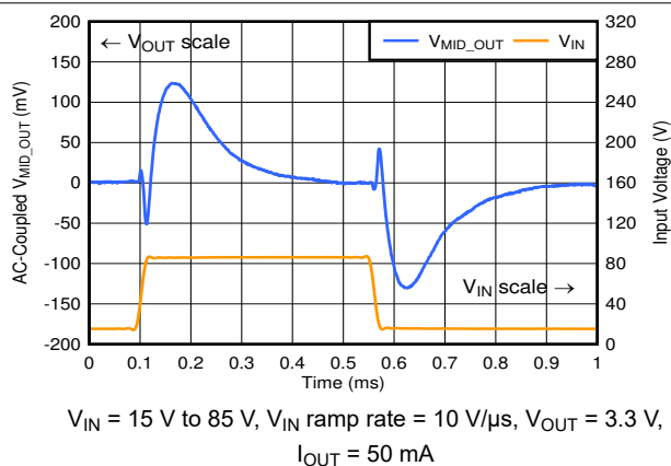
FIG 6-16. Line Transient
