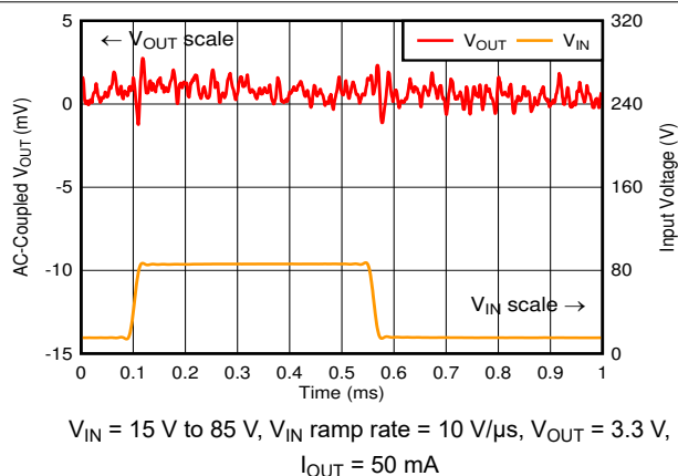
FIG 6-17. Line Transient
