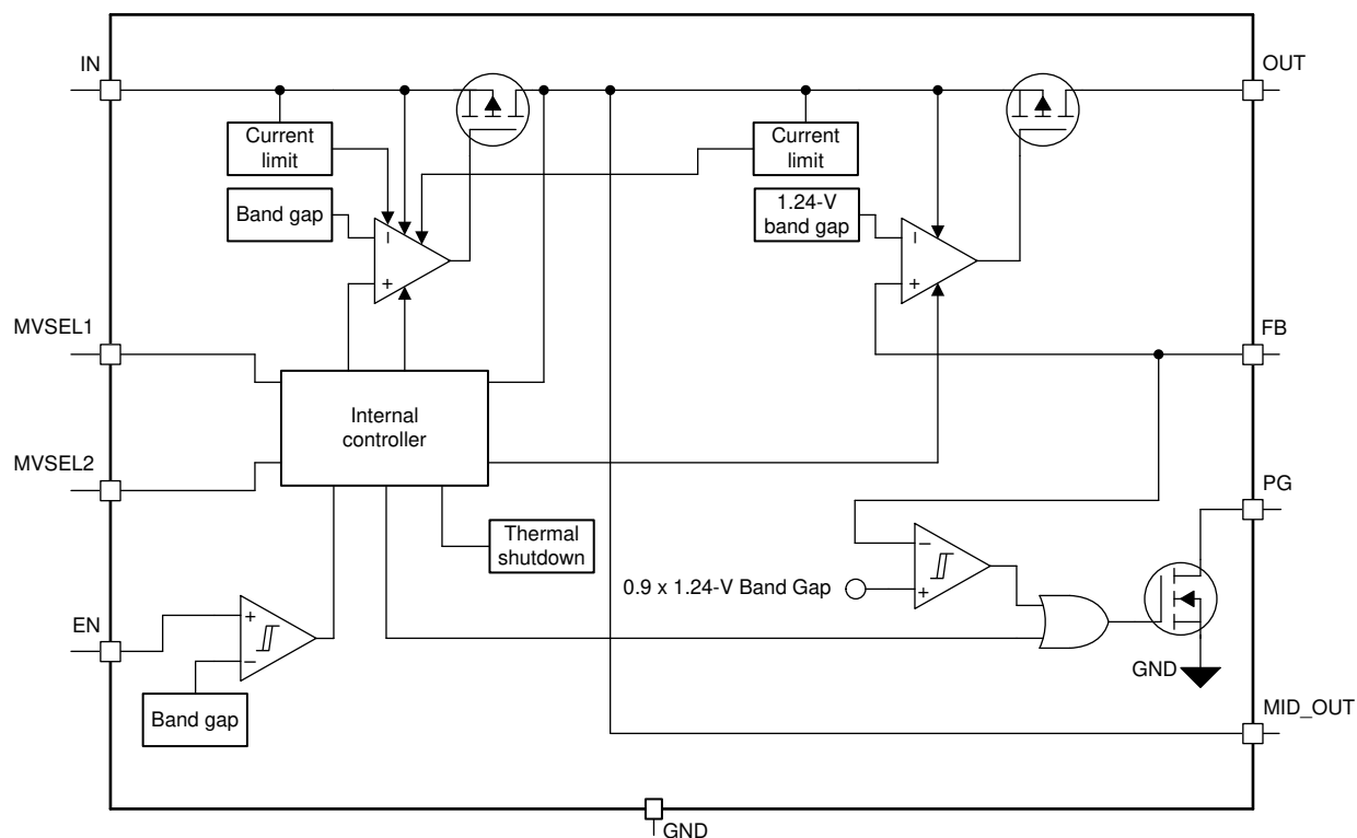
7-1. Adjustable Version
