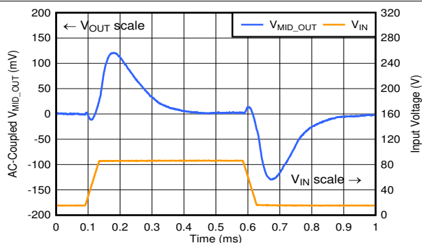
FIG 6-20. Line Transient ( V_{\text{MID\_OUT}} in Dropout)
