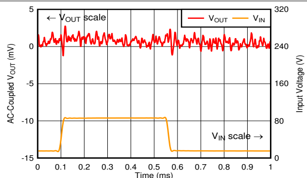
图 8-3. TPS7A43 Line Transient: 15 V to 85 V (Zoom on V OUT )
