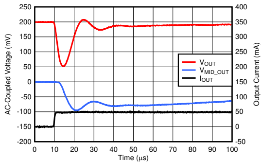
FIG 6-25. Load Transient (Rising Edge)
