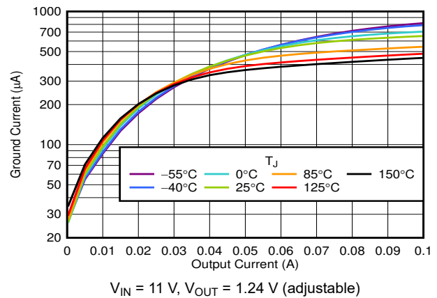
图 6-6. I_{GND} vs I_{OUT} ( MID\_OUT in Dropout)
