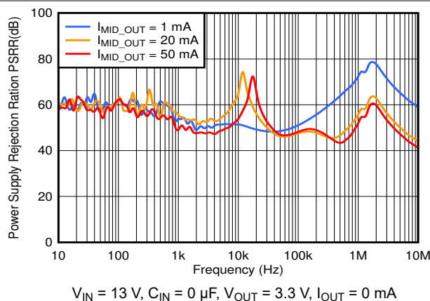
FIG 6-35. MID_OUT PSRR vs Frequency and I_{\text{MID\_OUT}}
