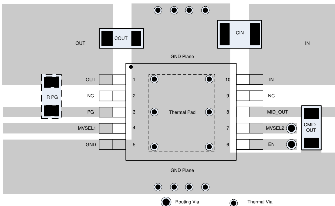
8-5. Fixed Version Layout Example
