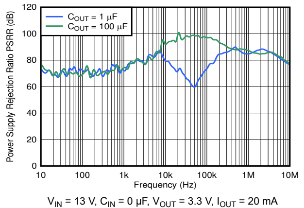
FIG 6-34. OUT PSRR vs Frequency and C_{\text{OUT}}
