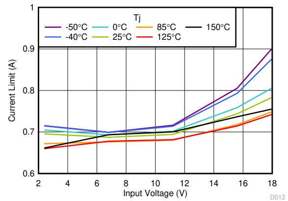
FIG 7-8. Current Limit vs V_{IN}
