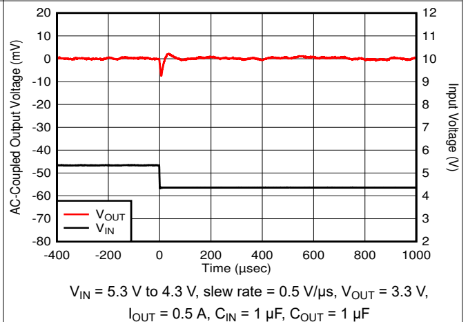
FIG 7-30. Line Transient
