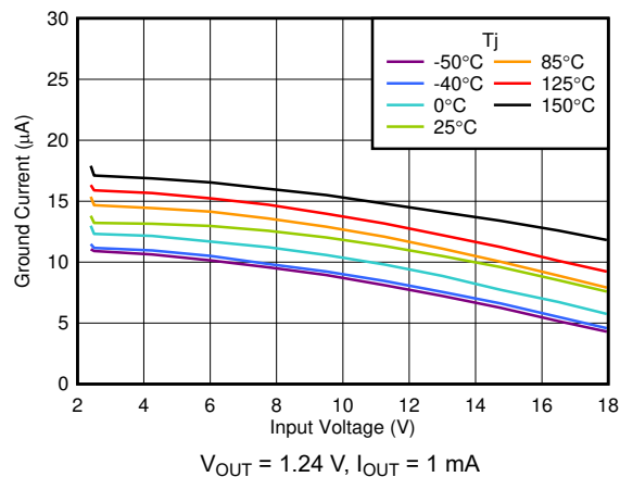
FIG 7-9. I_{GND} vs V_{IN}
