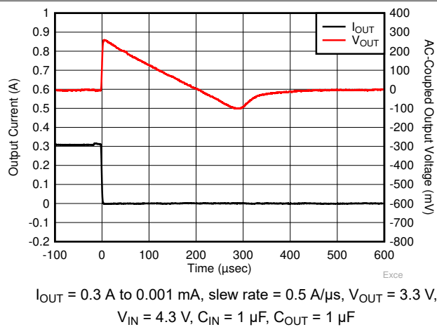
FIG 7-29. Load Transient
