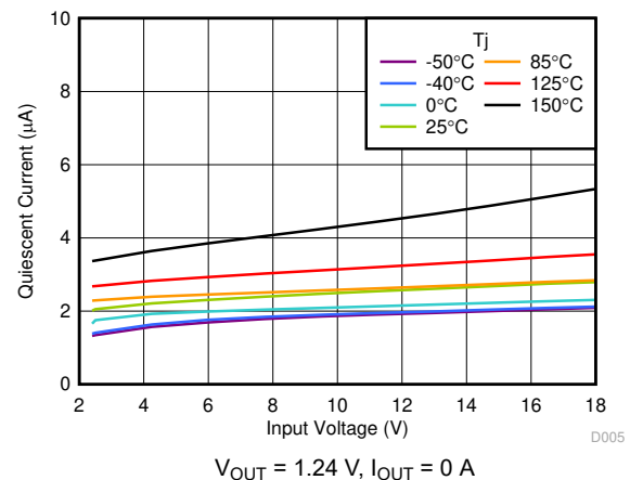
FIG 7-10. I_Q vs V_{IN}
