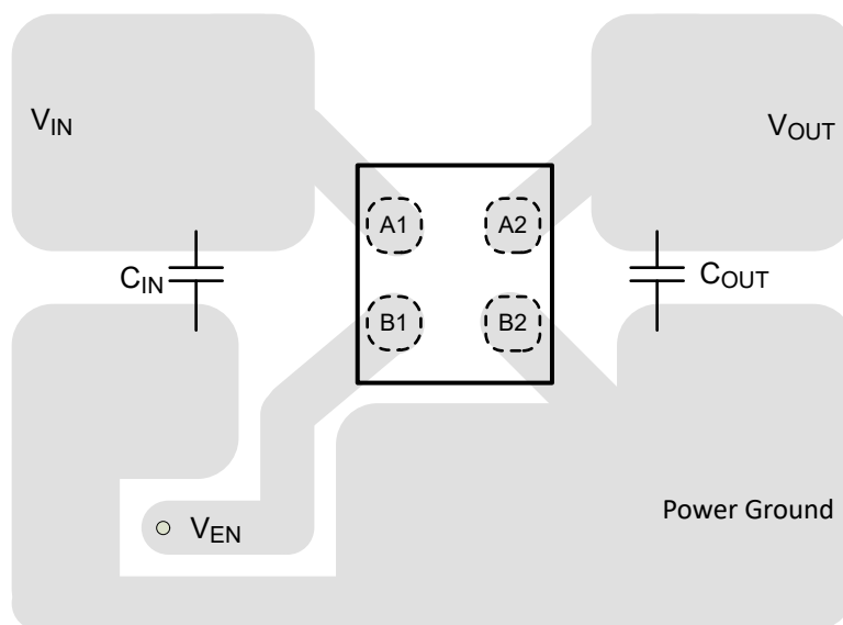
8-7. Typical DSBGA Layout
