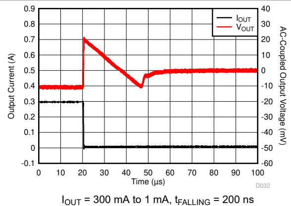
5-54. Load Transient
