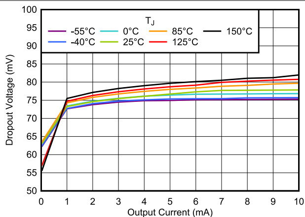
図 5-32. Dropout Voltage vs I_{OUT}
