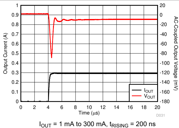
5-53. Load Transient
