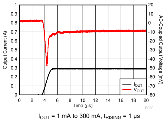
5-51. Load Transient
