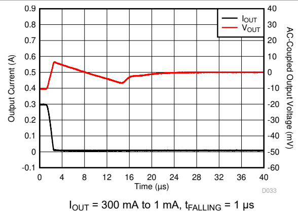
5-52. Load Transient
