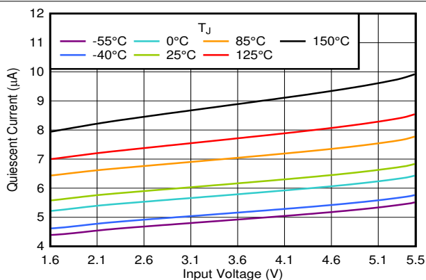
図 5-36. I_{GND} vs V_{IN} in the Dropout Region
