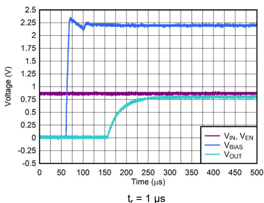
6-17. Start-Up With V_{\text{IN}} and V_{\text{EN}} Before V_{\text{BIAS}}
