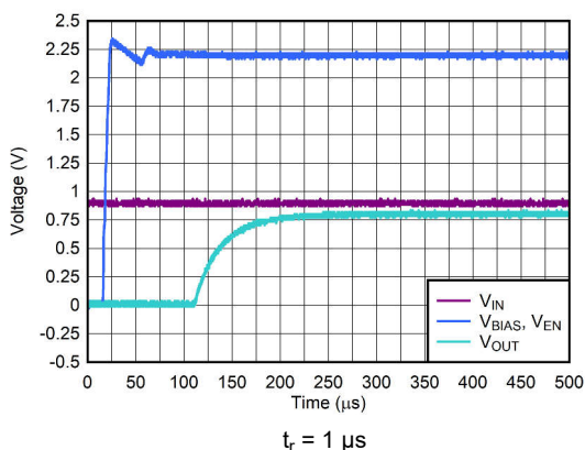
6-15. Start-Up With V_{\text{IN}} Before V_{\text{BIAS}} and V_{\text{EN}}
