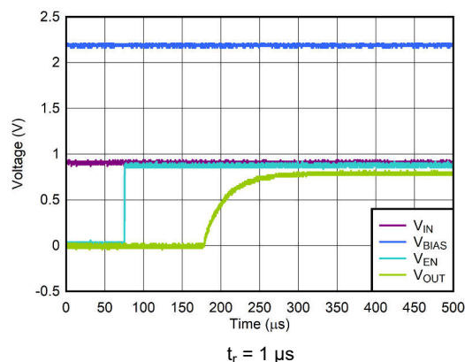
6-16. Start-Up With V_{\text{IN}} and V_{\text{BIAS}} Before V_{\text{EN}}
