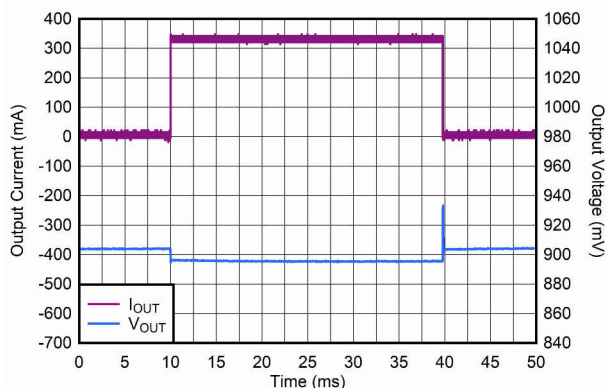
FIG 6-20. Load Transient From 100 \mu\text{A} to 320 mA
