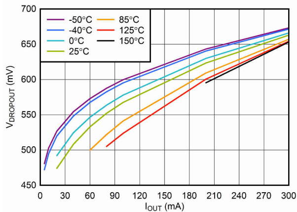
FIG 6-5. V_{\text{BIAS}} Dropout Voltage vs I_{\text{OUT}}
