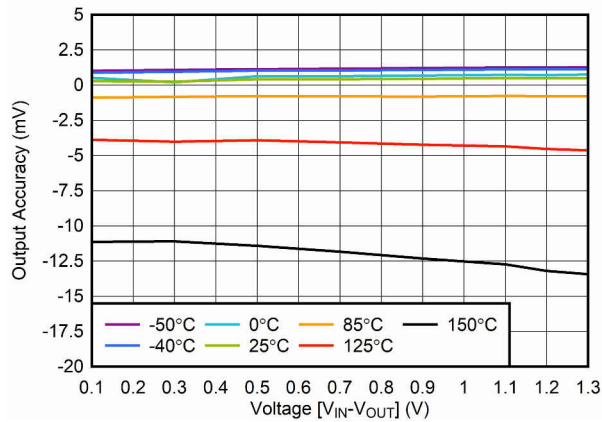
FIG 6-1. Output Voltage Accuracy vs V_{\text{IN}}
