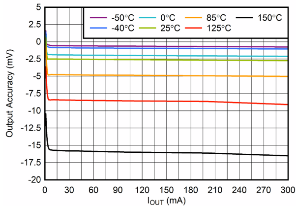
FIG 6-3. Output Voltage Accuracy vs I_{\text{OUT}}
