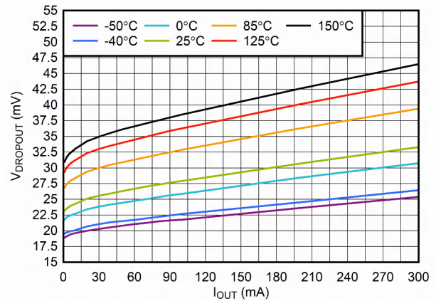
FIG 6-4. V_{\text{IN}} Dropout Voltage vs I_{\text{OUT}}
