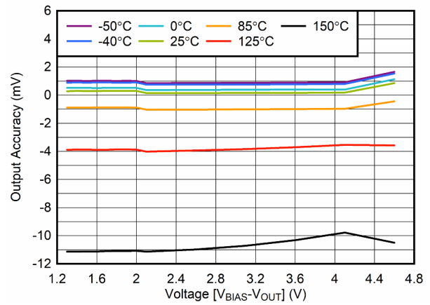
FIG 6-2. Output Voltage Accuracy vs V_{\text{BIAS}}
