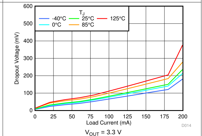
FIG 22. Dropout vs I_{OUT} and Temperature
