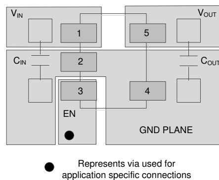
✎ 56. Layout Example for the DBV Package
