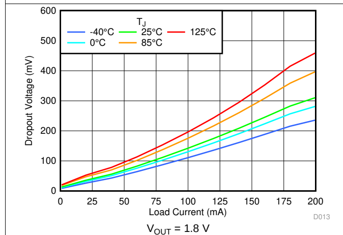
FIG 21. Dropout vs I_{OUT} and Temperature
