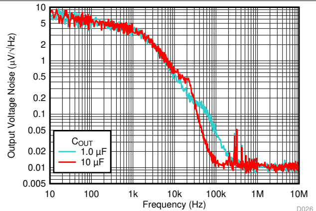
FIG 44. Output Noise vs Frequency and C_{OUT}
