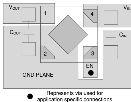
✎ 57. Layout Example for the DQN Package
