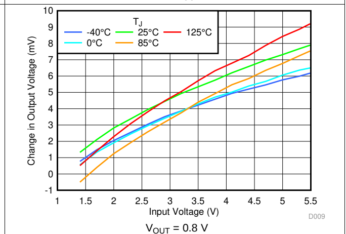
FIG 24. Line Regulation V_{IN} and Temperature
