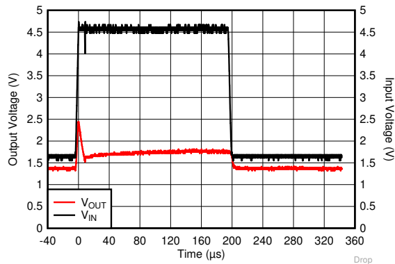
FIG 6-25. V_{IN} Transient From 1.5 V to 4.5 V
