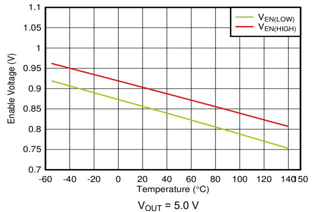
FIG 6-40. EN High and Low Threshold vs Temperature
