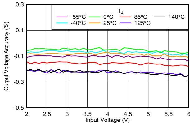
FIG 6-27. Output Accuracy vs V_{IN} and Temperature
