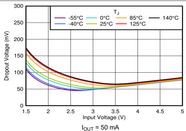
6-36. Dropout vs V_{IN} and Temperature
