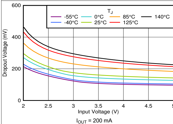
6-35. Dropout vs V_{IN} and Temperature
