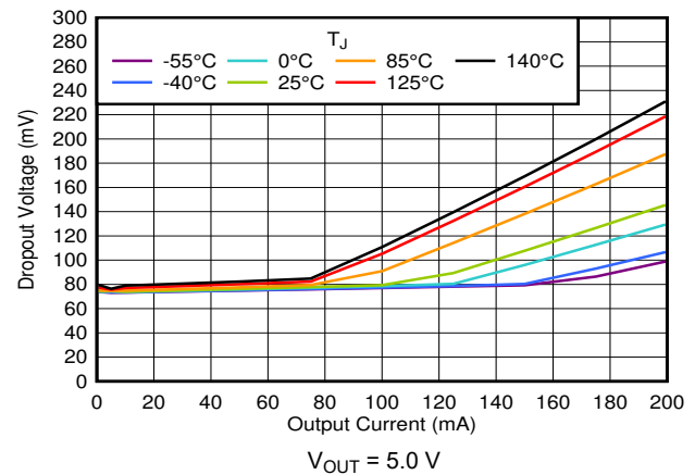
6-34. Dropout vs I_{OUT} and Temperature
