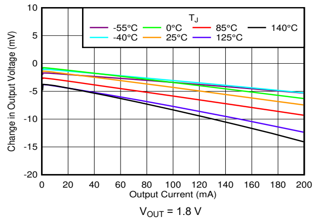
6-32. Load Regulation vs V_{IN} and Temperature
