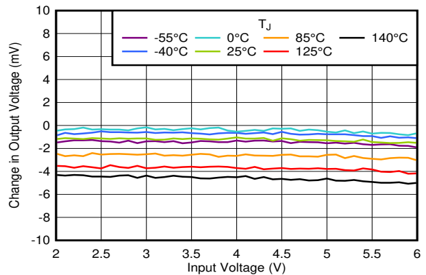
FIG 6-26. Line Regulation vs V_{IN} and Temperature
