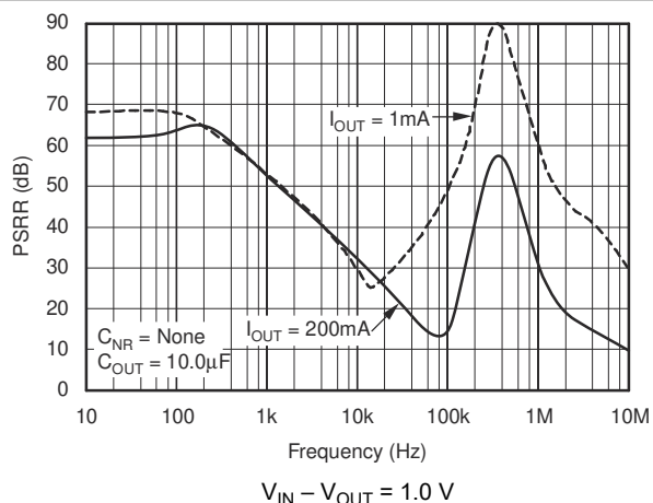
FIG 6-15. TPS799285 Power-Supply Ripple Rejection vs Frequency
