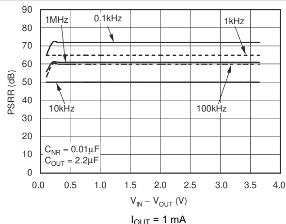
FIG 6-16. Power-Supply Ripple Rejection vs V_{IN} - V_{OUT}
