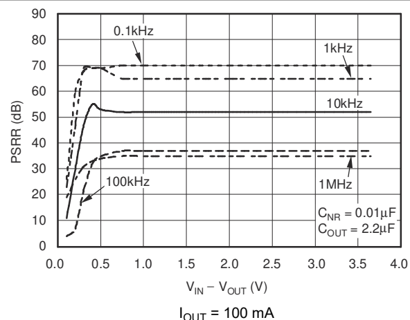
FIG 6-17. Power-Supply Ripple Rejection vs V_{IN} - V_{OUT}
