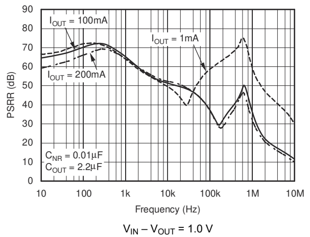
6-10. TPS799285 Power-Supply Ripple Rejection vs Frequency
