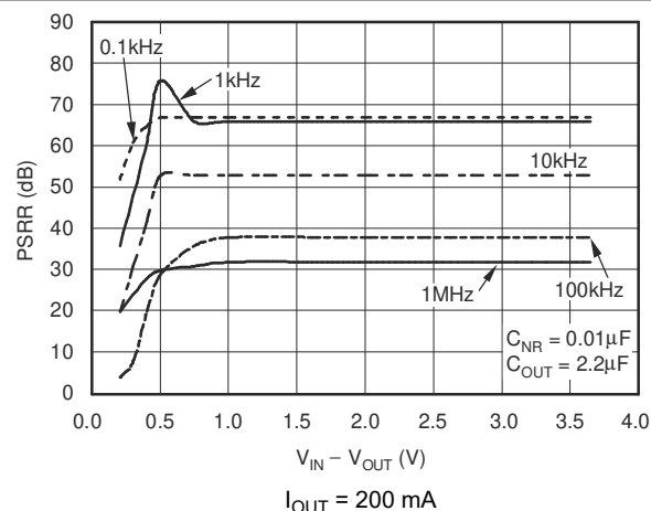
FIG 6-18. Power-Supply Ripple Rejection vs V_{IN} - V_{OUT}
