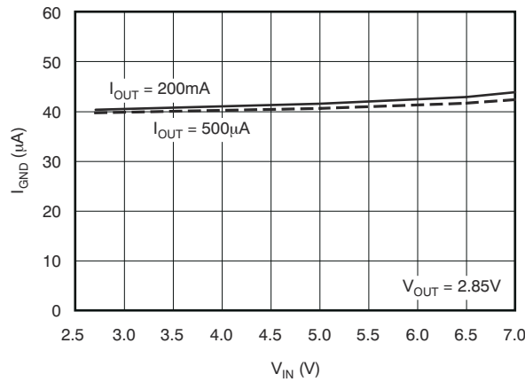
6-7. Ground Pin Current vs Input Voltage
