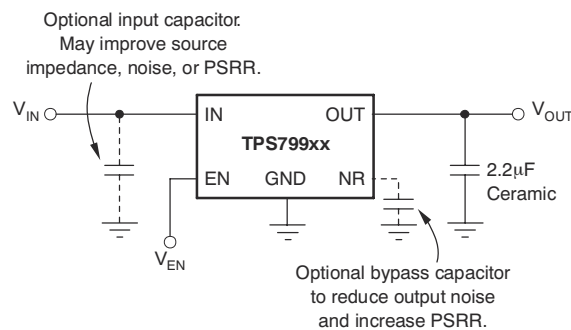
図 8-1. Typical Application Circuit for Fixed Voltage Versions
