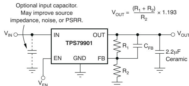
図 8-2. Typical Application Circuit for Adjustable Voltage Version
