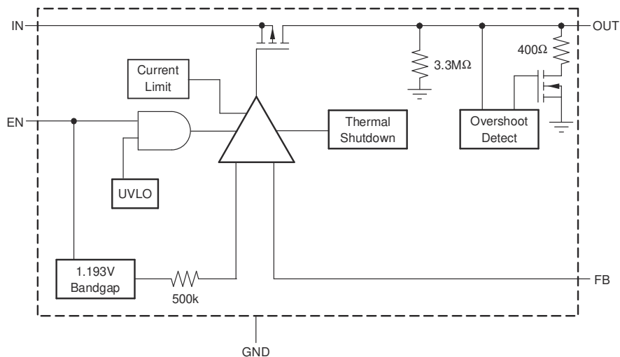
7-2. Adjustable-Voltage Versions
