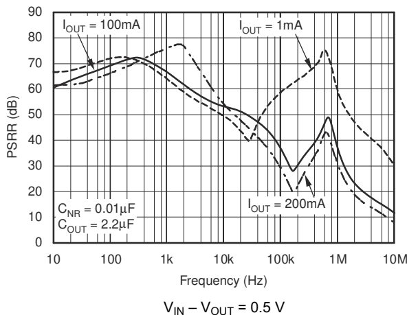
6-11. TPS799285 Power-Supply Ripple Rejection vs Frequency
