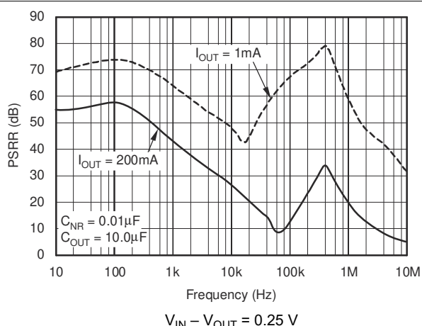
FIG 6-14. TPS799285 Power-Supply Ripple Rejection vs Frequency
