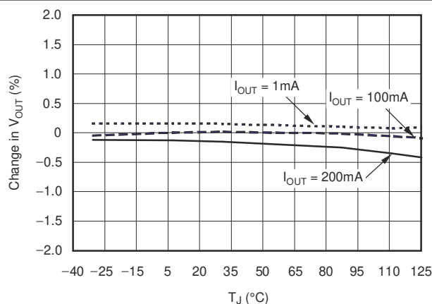
FIG 6-1. Load Regulation
