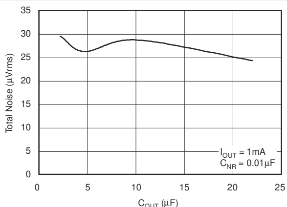
FIG 6-20. TPS799285 Total Noise vs C_{OUT}
