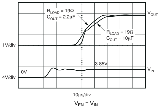
FIG 6-23. TPS799285 Turn-On Response
