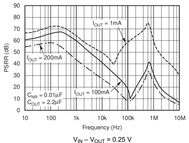
6-12. TPS799285 Power-Supply Ripple Rejection vs Frequency
