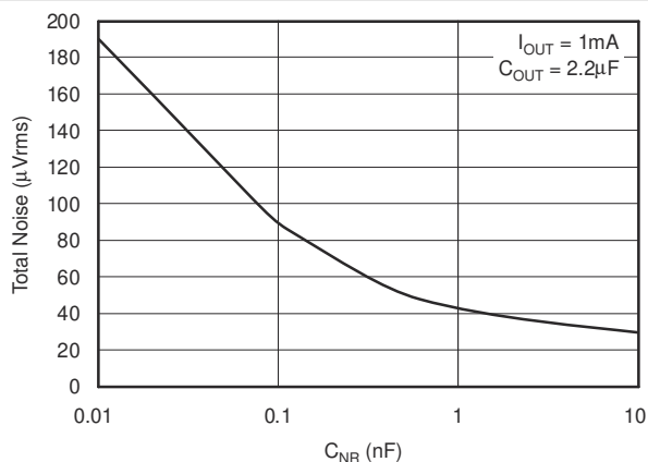
FIG 6-19. TPS799285 Total Noise vs C_{NR}
