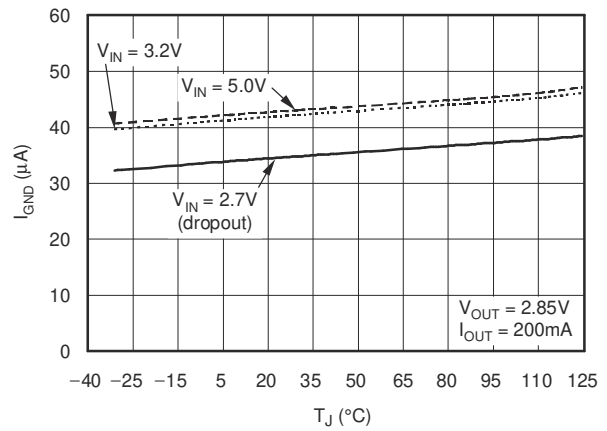
6-8. TPS799285 Ground Pin Current vs Junction Temperature
