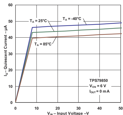
図 5-8. Quiescent Current vs Input Voltage
