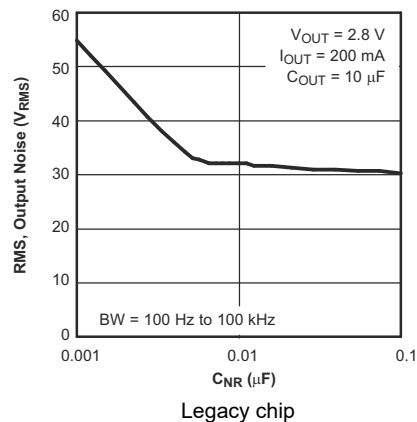
Figure 5-10. Root Mean Square Output Noise vs C_{\text{NR}}
