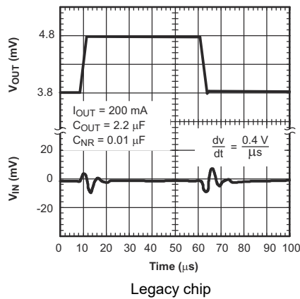
5-23. TPS793 Line Transient Response
