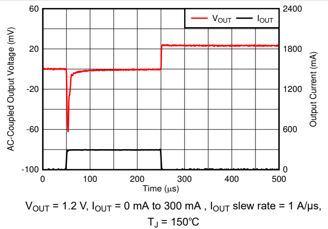
FIG 6-52. Load Transient
