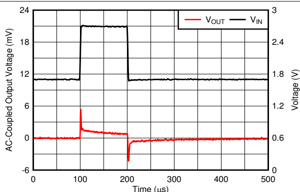
FIG 6-28. Line Transient
