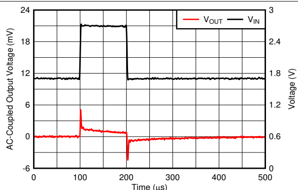
FIG 6-27. Line Transient
