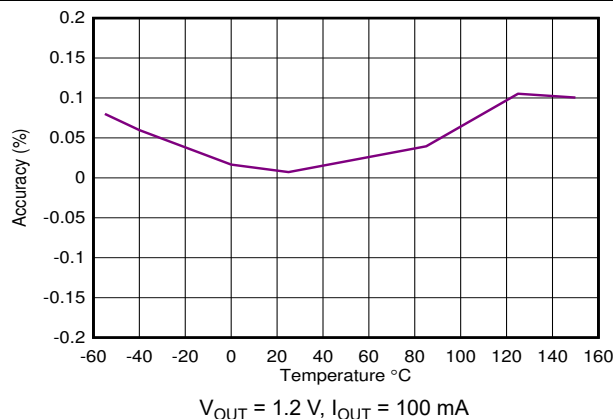
FIG 6-9. Accuracy vs Temperature
