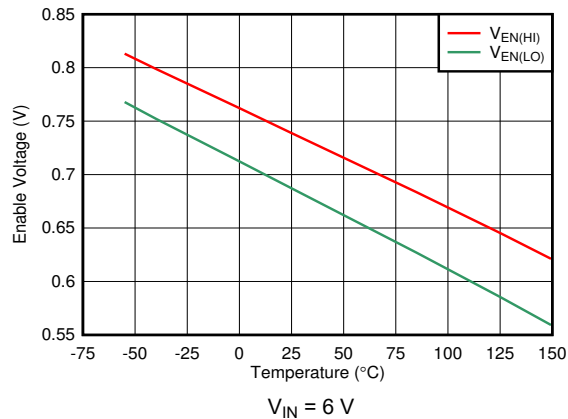
FIG 6-21. V_{\text{EN(HI)}} and V_{\text{EN(LO)}} Thresholds vs Temperature
