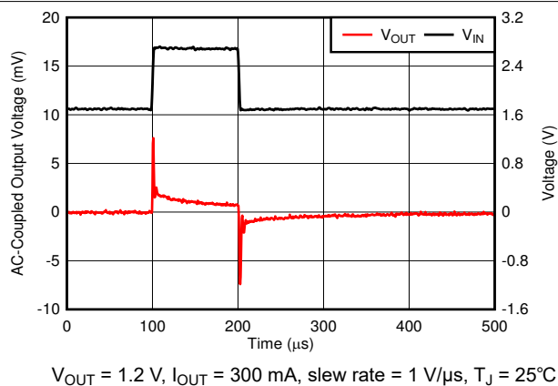
FIG 6-32. Line Transient
