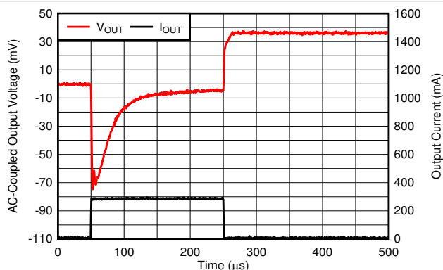
FIG 6-61. Load Transient
