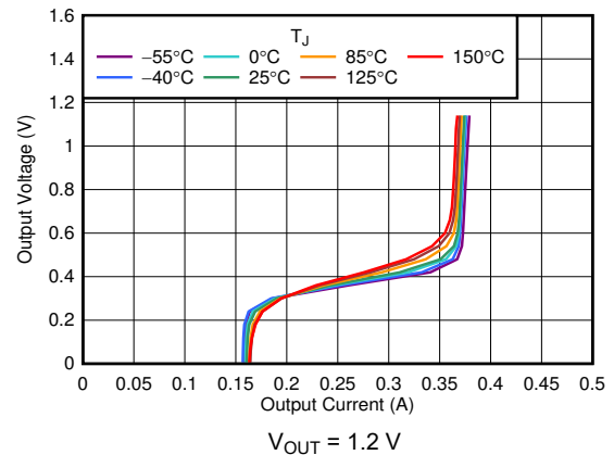
FIG 6-22. Foldback Current Limit vs I_{\text{OUT}} and Temperature
