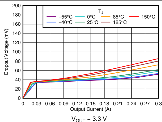
FIG 6-12. Dropout Voltage vs I_{\text{OUT}}
