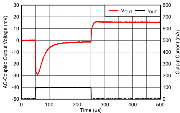
FIG 6-55. Load Transient
