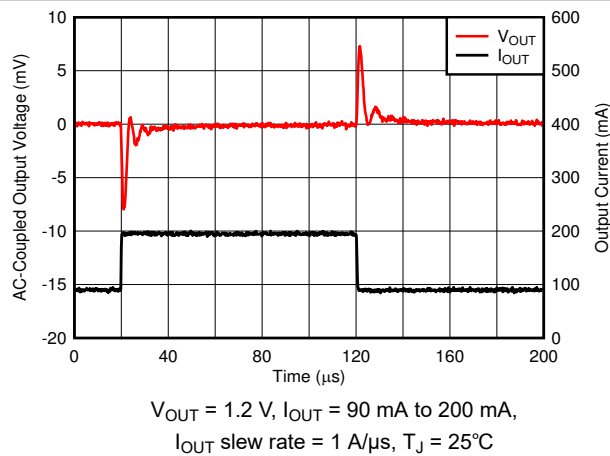
FIG 6-53. Load Transient
