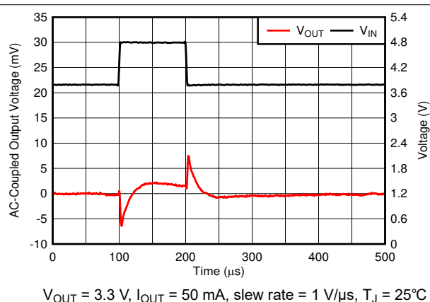
FIG 6-35. Line Transient
