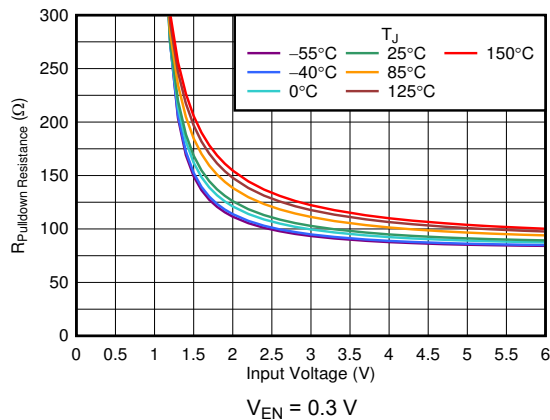
FIG 6-19. Pulldown Resistor ( R_{\text{Pulldown}} ) vs V_{\text{IN}}
