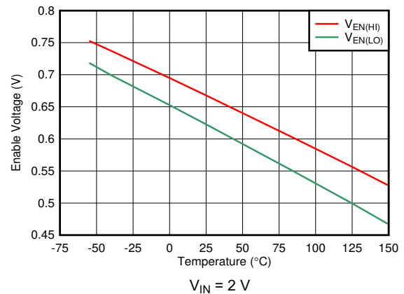
FIG 6-20. V_{\text{EN(HI)}} and V_{\text{EN(LO)}} Thresholds vs Temperature
