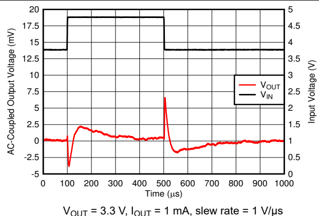
FIG 6-24. Line Transient
