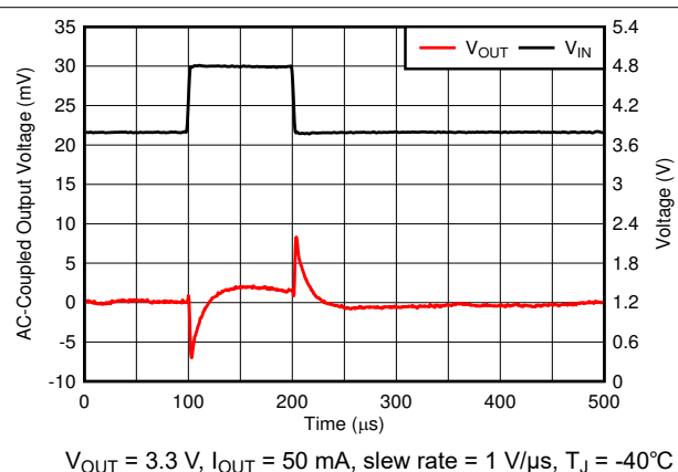
FIG 6-36. Line Transient
