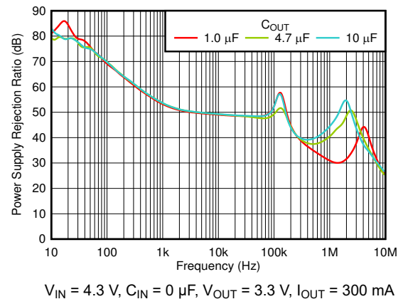
Figure 6-68. PSRR vs Frequency and C_{OUT}
