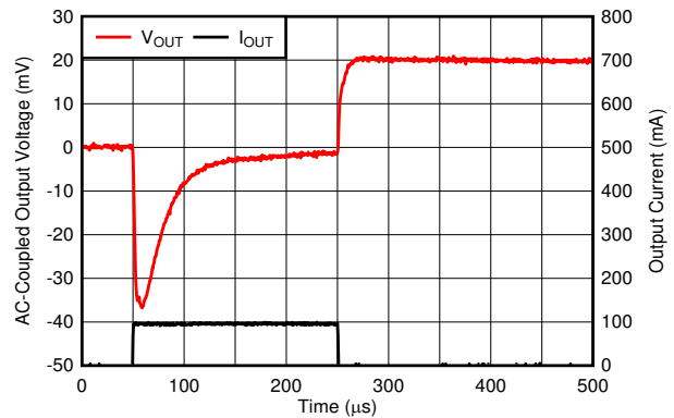
FIG 6-56. Load Transient
