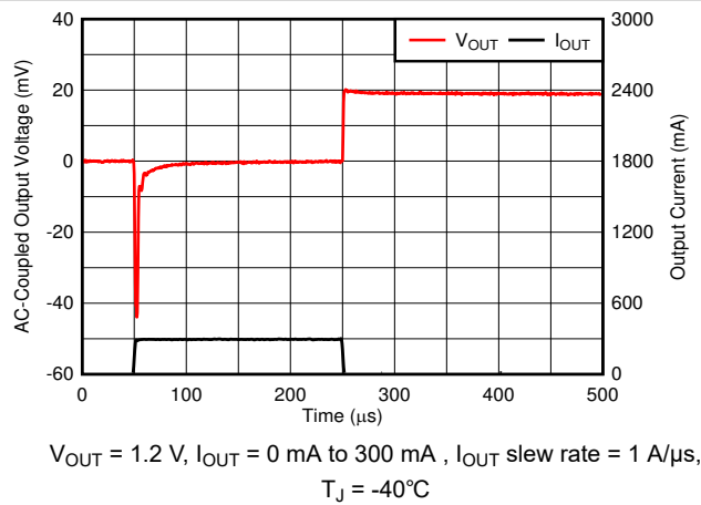
FIG 6-51. Load Transient
