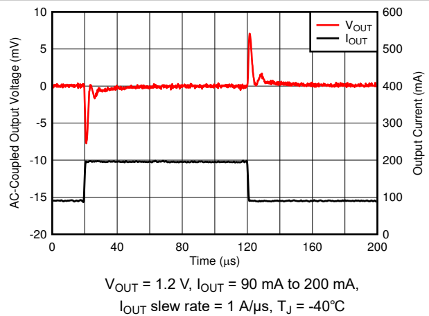
FIG 6-54. Load Transient
