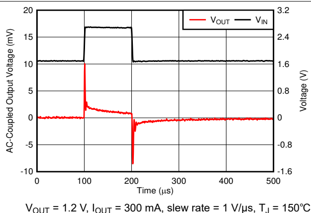
FIG 6-34. Line Transient
