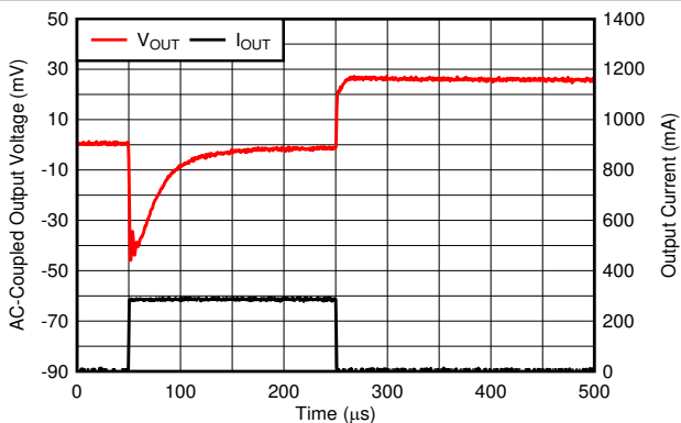
FIG 6-58. Load Transient
