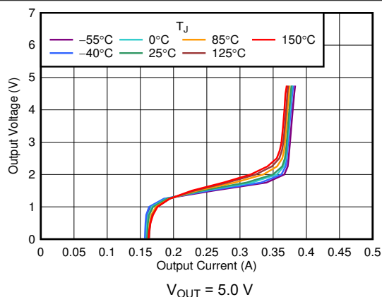
FIG 6-23. Foldback Current Limit vs I_{\text{OUT}} and Temperature
