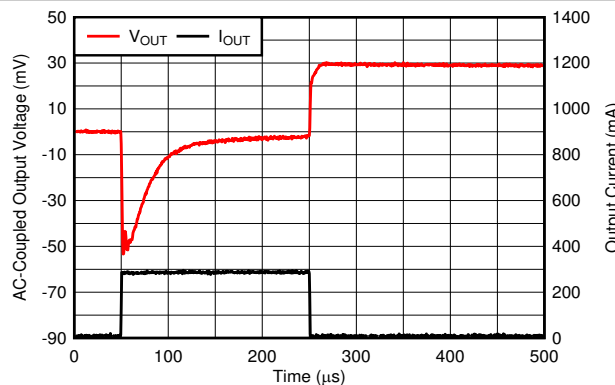
FIG 6-57. Load Transient
