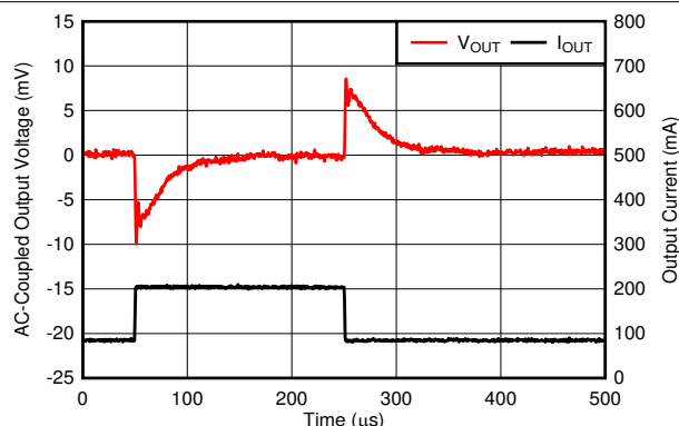
FIG 6-61. Load Transient
