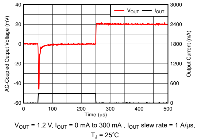
FIG 6-50. Load Transient
