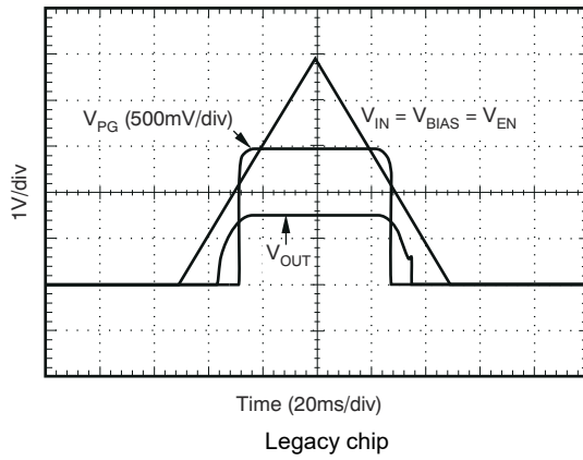
Figure 5-40. Power-Up, Power-Down
