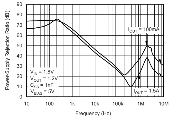
Figure 5-14. V_{BIAS} PSRR vs Frequency
