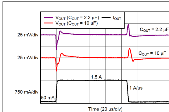
図 7-2. Load Transient Response
