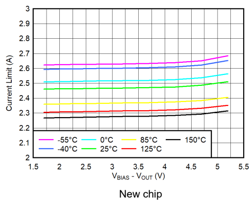
5-32. Current Limit vs ( V_{BIAS} - V_{OUT} )
