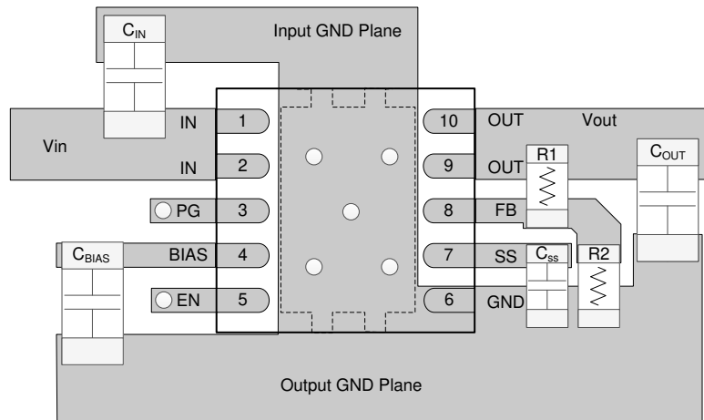
8-10. TPS547 Layout Recommendation
