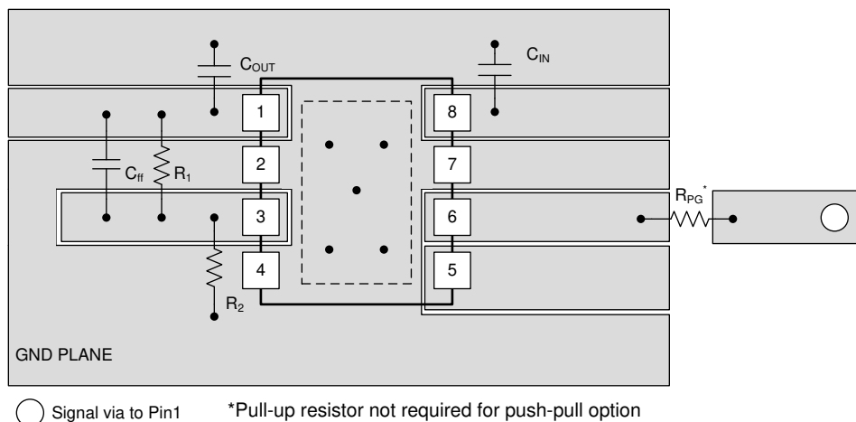
10-2. Layout Example for the DRB Package
