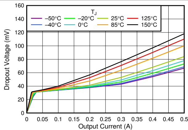
FIG 6-9. 3.3-V Dropout Voltage vs I_{OUT}
