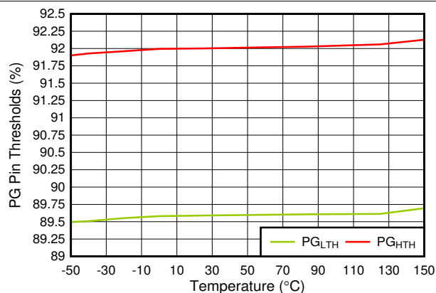
FIG 6-20. PG_{LTH} and PG_{HTH} vs Temperature
