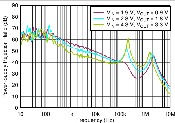
FIG 6-39. PSRR vs Frequency and V_{IN}
