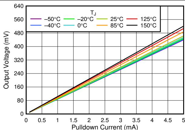
FIG 6-19. V_{OUT} vs I_{OUT} Pulldown Resistor
