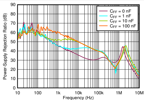
FIG 6-43. PSRR vs Frequency and C_{FF}
