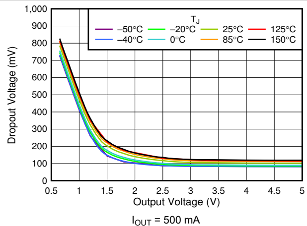
FIG 6-12. V_{DO} vs V_{OUT}
