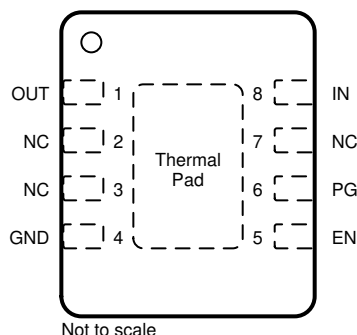
图 5-4. DRB Package, 8-Pin Fixed VSON (Top View)
