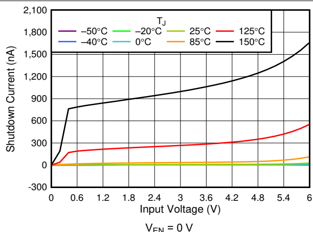
FIG 6-14. I_{SHDN} vs V_{IN}
