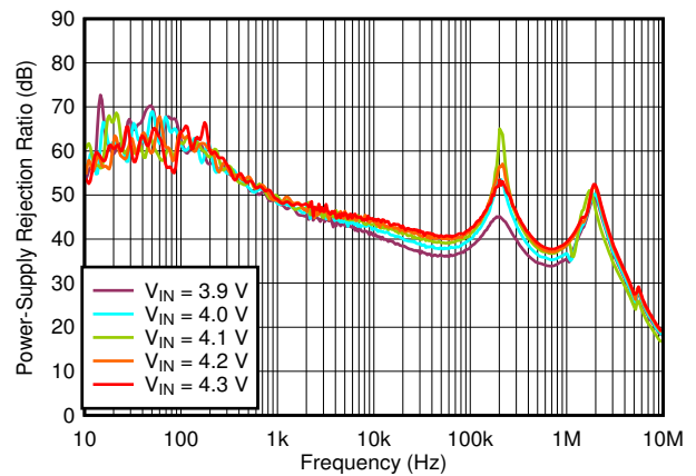
FIG 6-38. PSRR vs Frequency and V_{IN}
