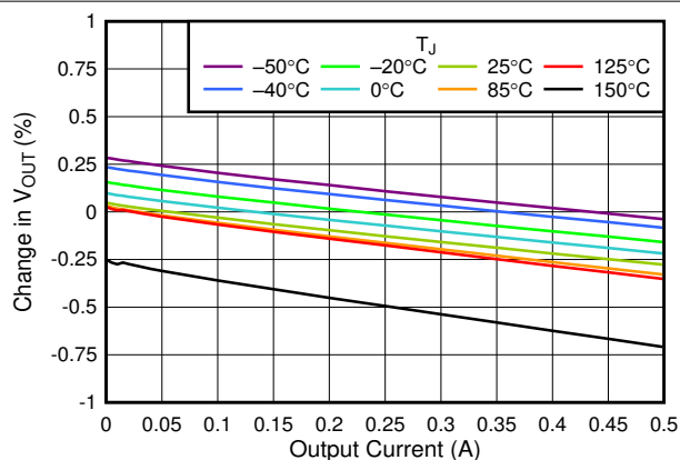
FIG 6-18. 5.5-V Load Regulation vs I_{OUT}
