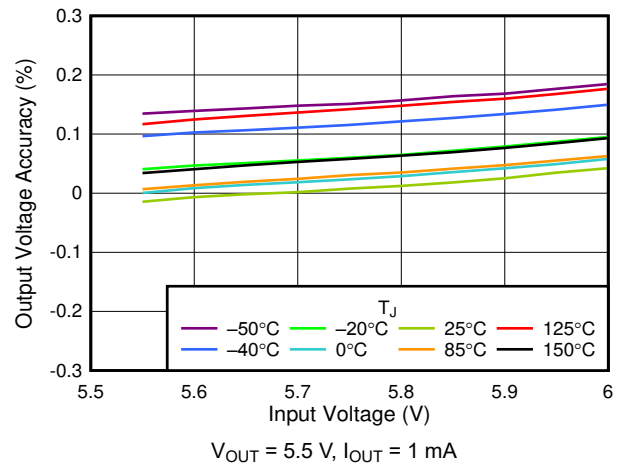
FIG 6-8. 5.5-V Line Regulation vs V_{IN}
