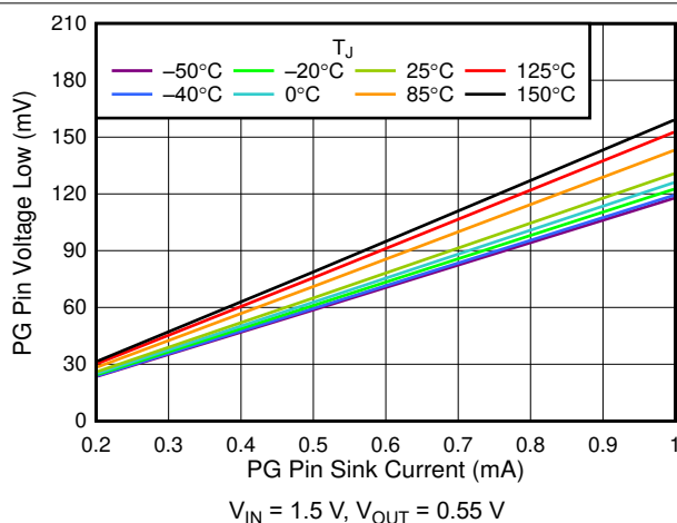
FIG 6-23. V_{OL}(PG) vs PG Pin Sink Current
