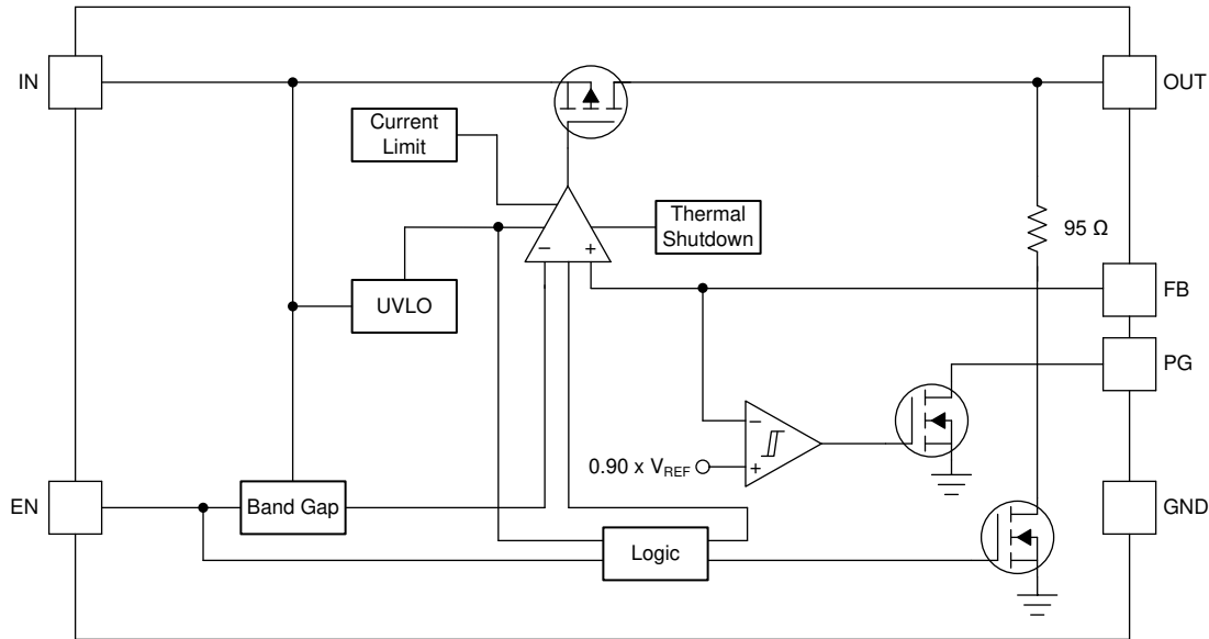
FIG 7-1. Adjustable Version With Open-Drain Power-Good
