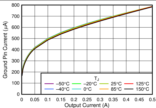
FIG 6-13. I_{GND} vs I_{OUT}
