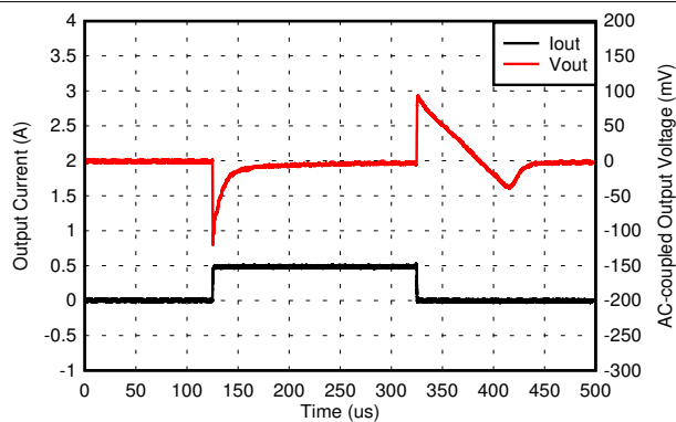
FIG 6-32. 3.3-V, 1-mA to 500-mA Load Transient
