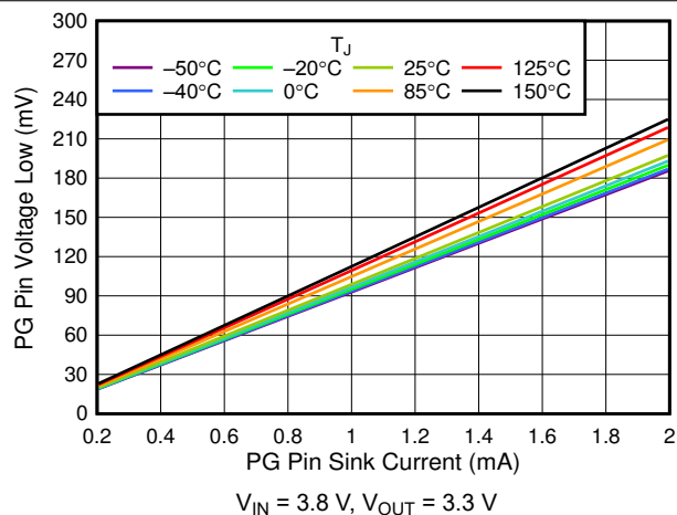
FIG 6-22. V_{OL}(PG) vs PG Pin Sink Current
