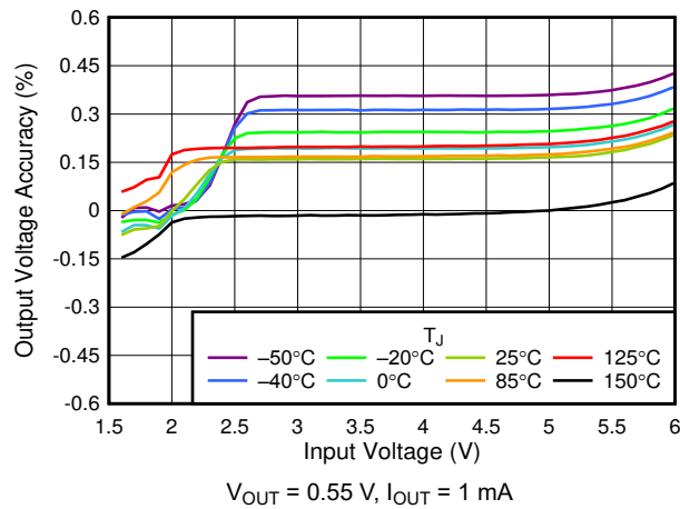
FIG 6-7. 0.55-V Line Regulation vs V_{IN}
