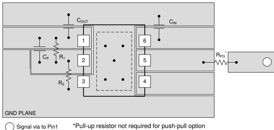
10-1. Layout Example for the DRV Package
