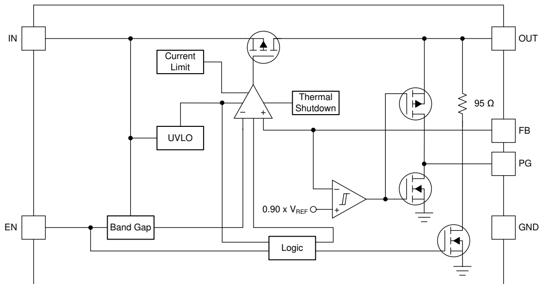
FIG 7-2. Adjustable Version With Push-Pull Power-Good
