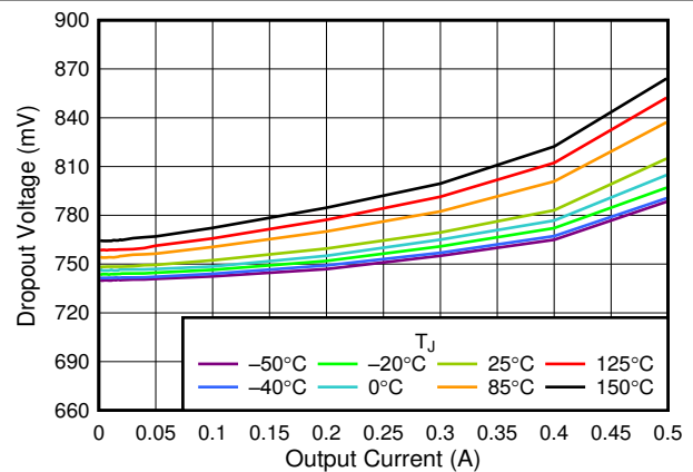
FIG 6-10. 0.55-V Dropout Voltage vs I_{OUT}
