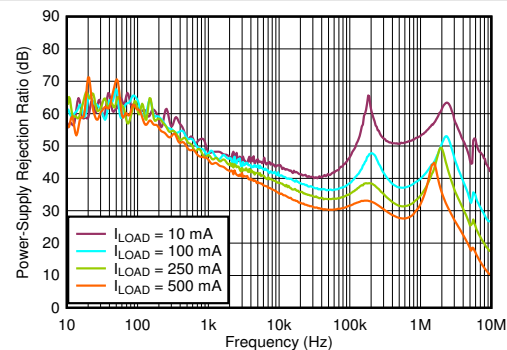
FIG 6-44. PSRR vs Frequency and I_{LOAD}
