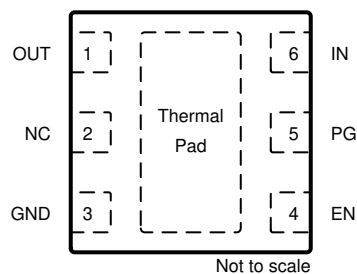
图 5-2. DRV Package, 6-Pin Fixed WSON (Top View)
