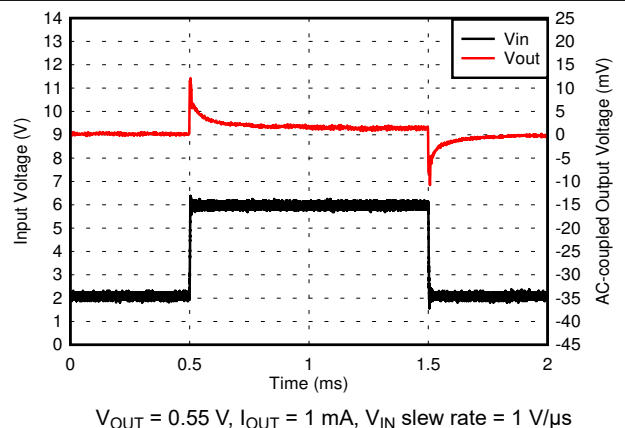
6-30. 0.55-V Line Transient
