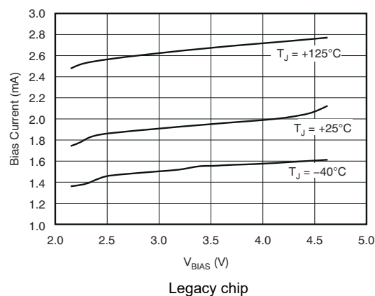
Figure 5-26. I_{\text{BIAS}} vs V_{\text{BIAS}} and V_{\text{OUT}}
