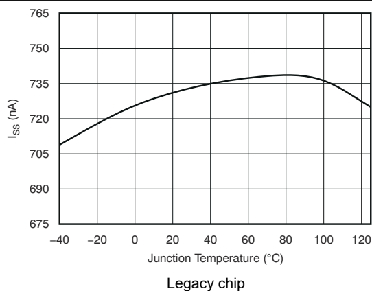
Figure 5-29. Soft-Start Charging Current ( I_{\text{SS}} ) vs Temperature
