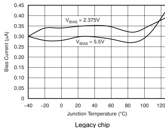
Figure 5-28. I_{\text{BIAS}} Shutdown vs Temperature
