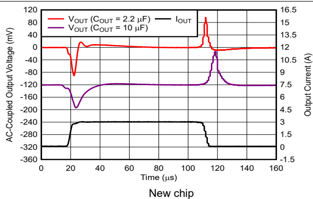
Figure 5-34. Load Transient Response
