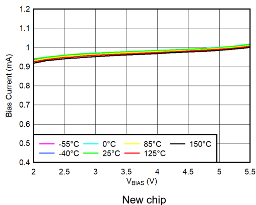
Figure 5-27. BIAS Pin Current vs V_{\text{BIAS}} and Temperature ( T_J )
