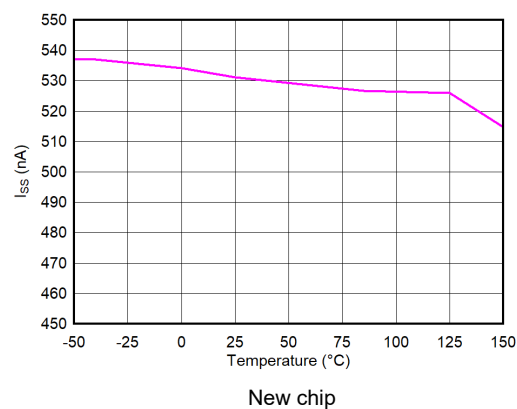
Figure 5-30. Soft-Start Charging Current ( I_{\text{SS}} ) vs Temperature ( T_J )
