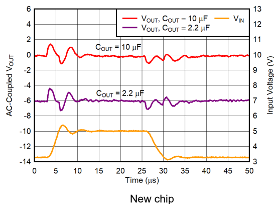
Figure 5-36. V_{BIAS} Line Transient
