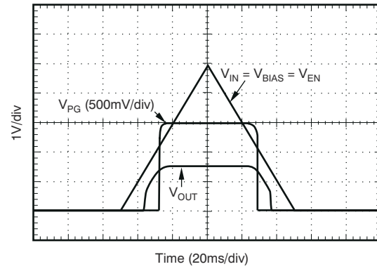
図 7-3. Power-Up, Power-Down
