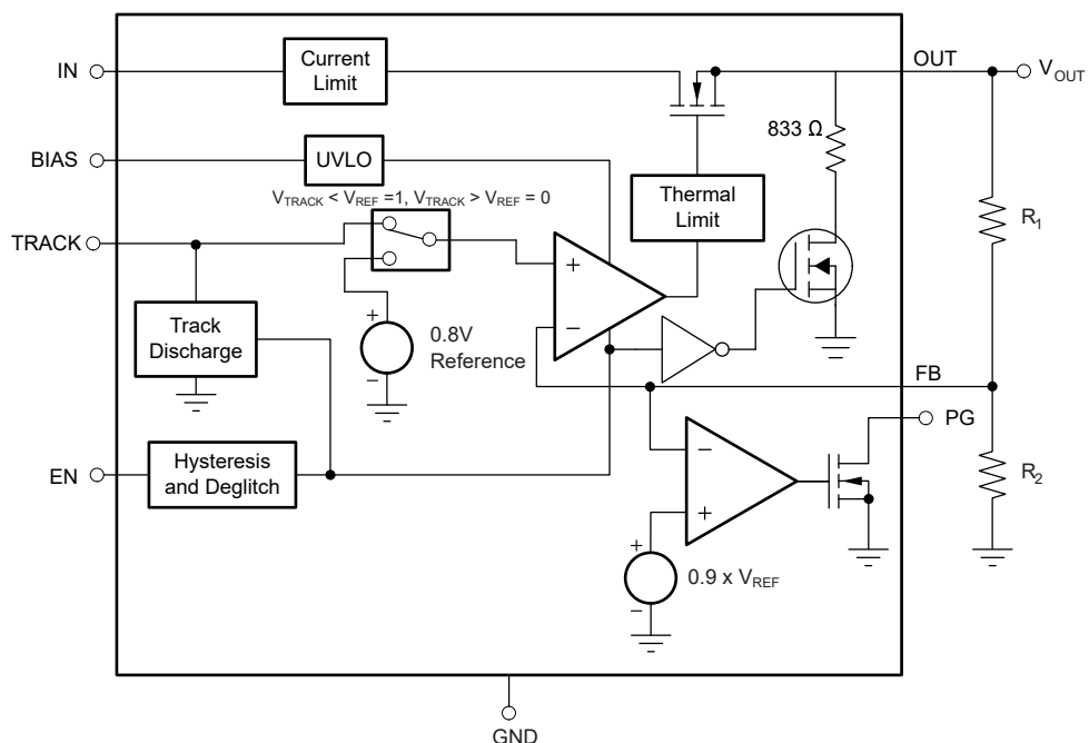
図 6-2. New chip Functional Block Diagram
