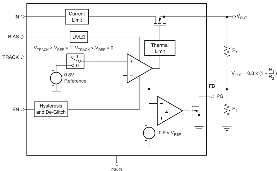
6-1. Legacy chip Functional Block Diagram
