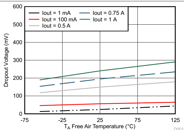
图 6-2. Dropout Voltage vs Temperature
