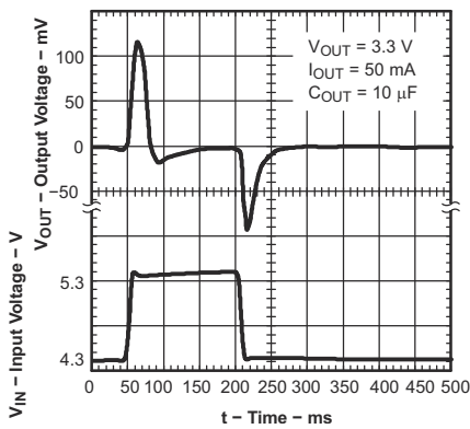
Figure 7-8. Line Transient Response (Legacy Chip)
