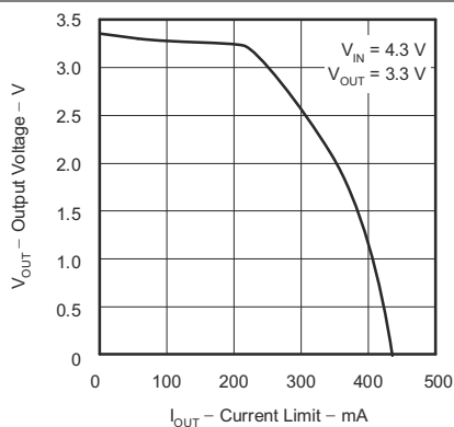
5-19. Output Voltage vs Current Limit (Legacy Chip)
