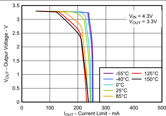
5-20. Output Voltage vs Current Limit (New Chip)
