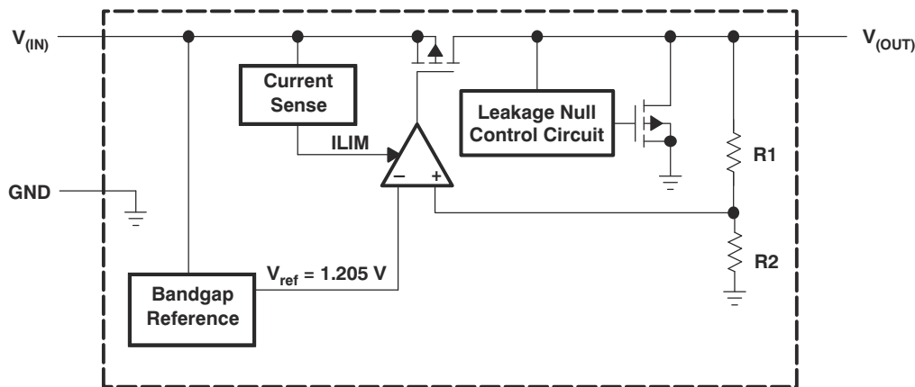
图 7-2. Functional Block Diagram—Fixed Version
