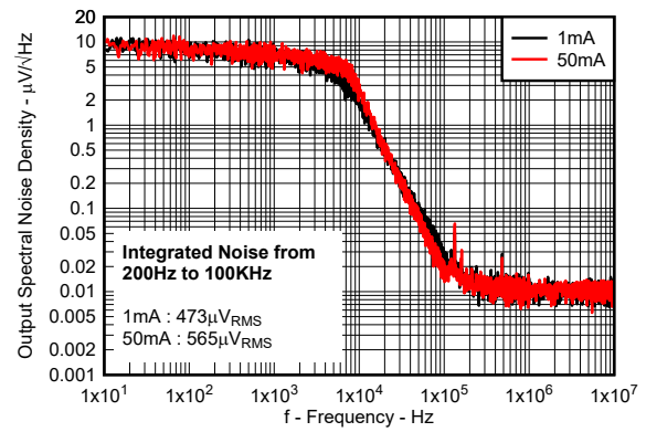
FIG 6-8. Output Spectral Noise Density vs Frequency for New Chip
