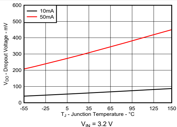
6-14. Dropout Voltage vs Free-Air Temperature for New Chip
