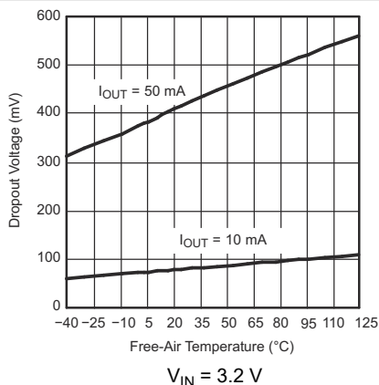
6-13. Dropout Voltage vs Free-Air Temperature for Legacy Chip
