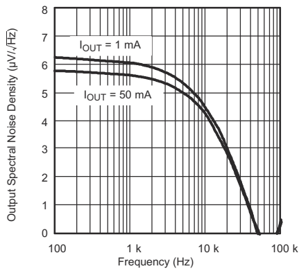
FIG 6-7. Output Spectral Noise Density vs Frequency for Legacy Chip
