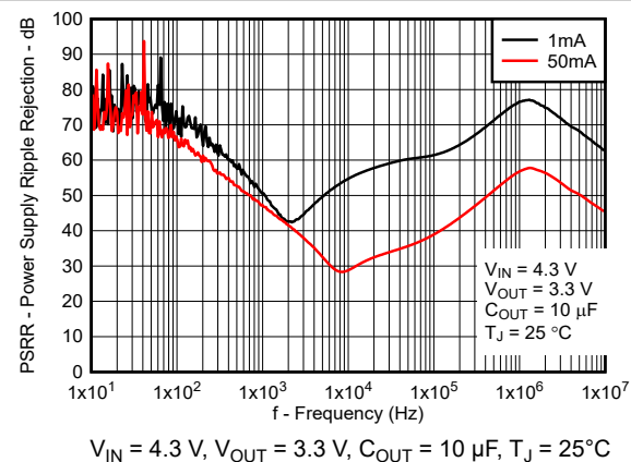
6-16. Power-Supply Ripple Rejection vs Frequency for New Chip
