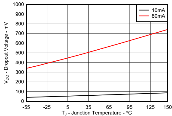
FIG 5-13. TPS71433 Dropout Voltage vs Junction Temperature (New Chip)
