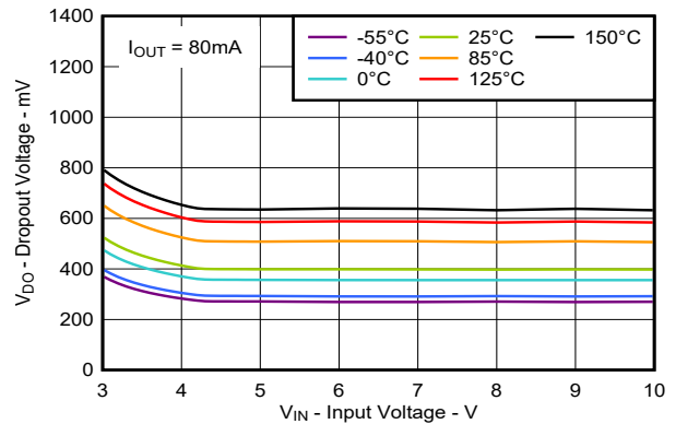
FIG 5-14. TPS71401 Dropout Voltage vs Input Voltage (New Chip)
