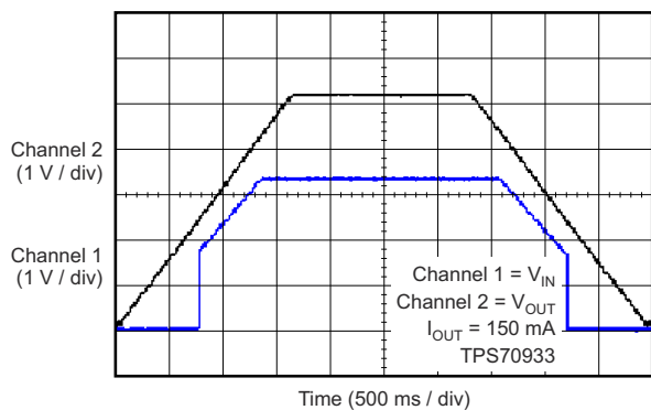
Figure 6-34. Power-Up and Power-Down Response
