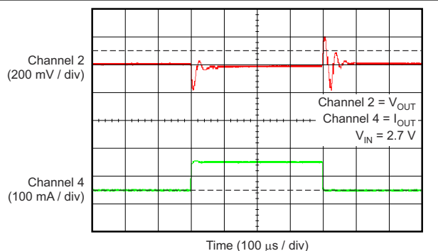
FIG 6-22. TPS70912 Load Transient (1 mA to 150 mA)
