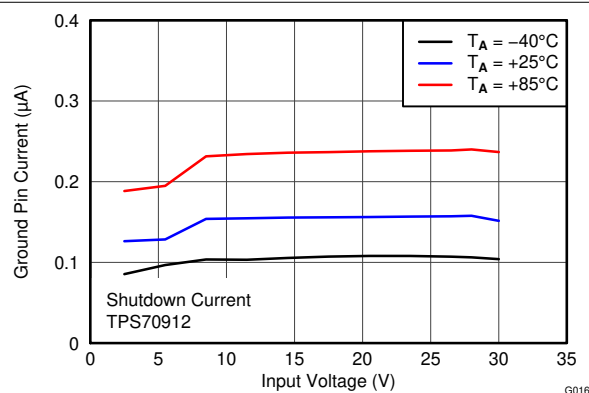
FIG 6-15. GND Current vs V_{\text{IN}} and Temperature
