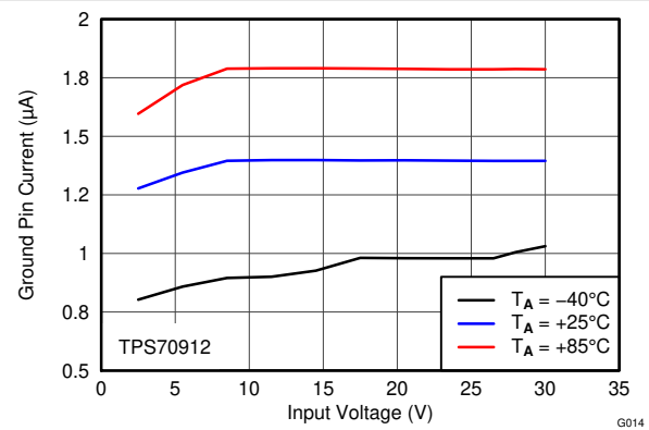
FIG 6-14. GND Current vs V_{\text{IN}} and Temperature
