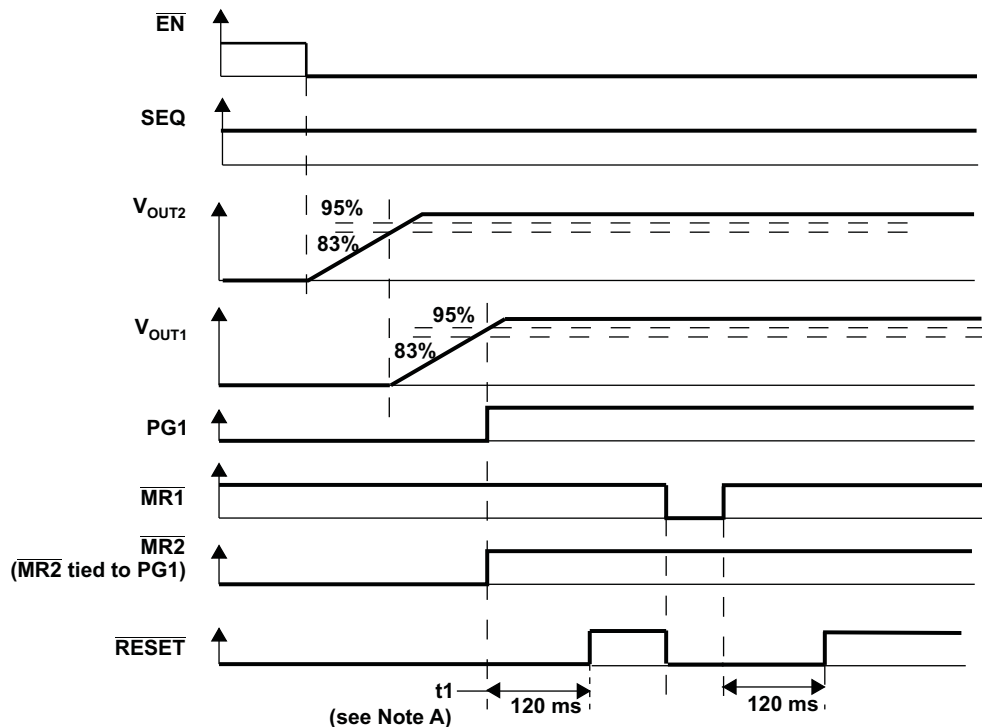
Figure 35. Timing When \overline{\text{MR1}} Is Toggled
