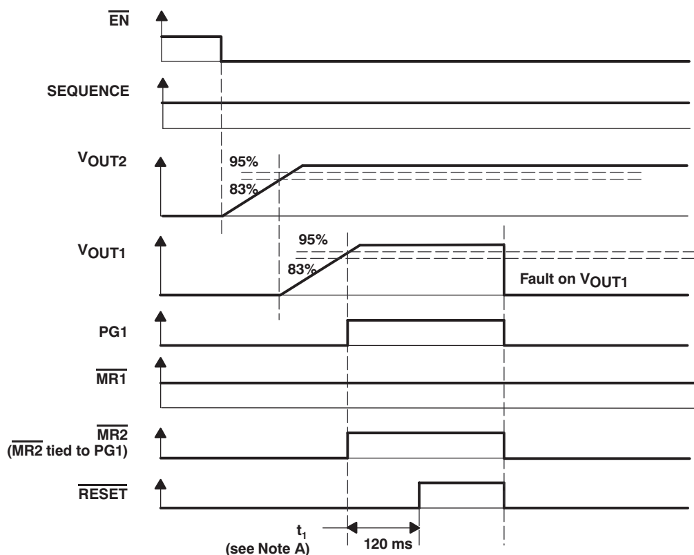
Figure 41. Timing When a Fault Occurs on V OUT1
