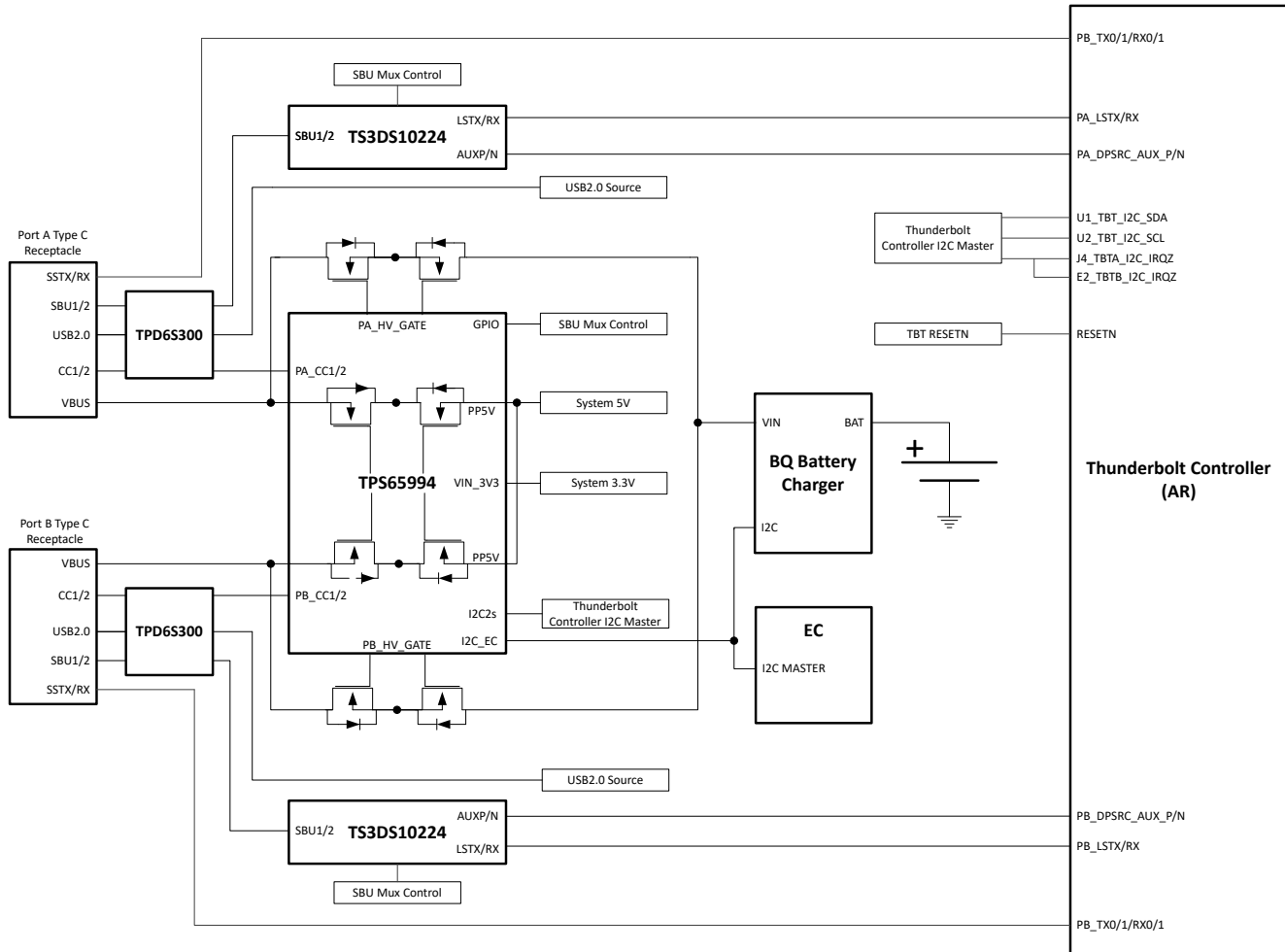
图 9-6. Thunderbolt Architecture
