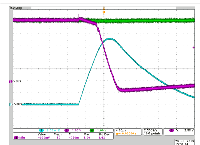
9-4. Px_VBUS Short with TVS2200 and Schottky Diode
