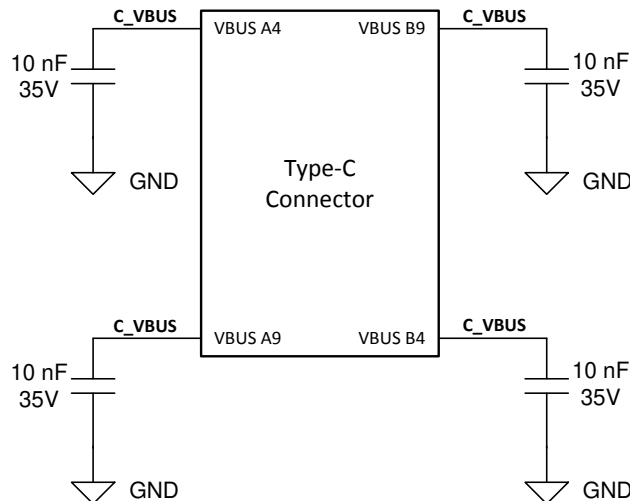
✎ 9-1. Type-C Connector VBUS Capacitors
