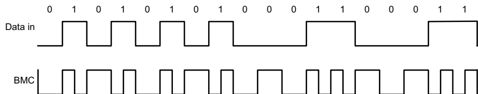
FIG 8-4. Biphasic Mark Coding Example
