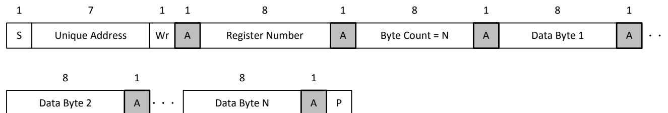
図 8-25. I 2 C Unique Address Write Register Protocol
