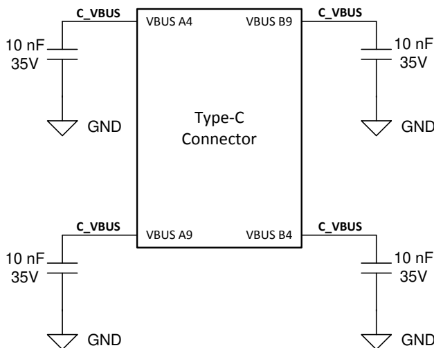
9-2. Type-C Connector VBUS Capacitors
