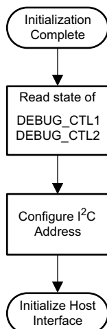
FIG 9-53. I 2 C Address Configuration
