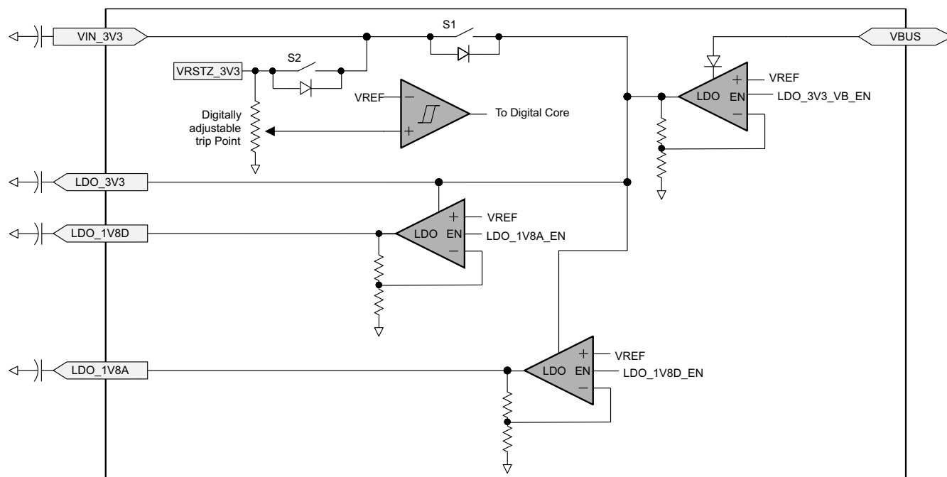
FIG 9-40. Power Supply Path
