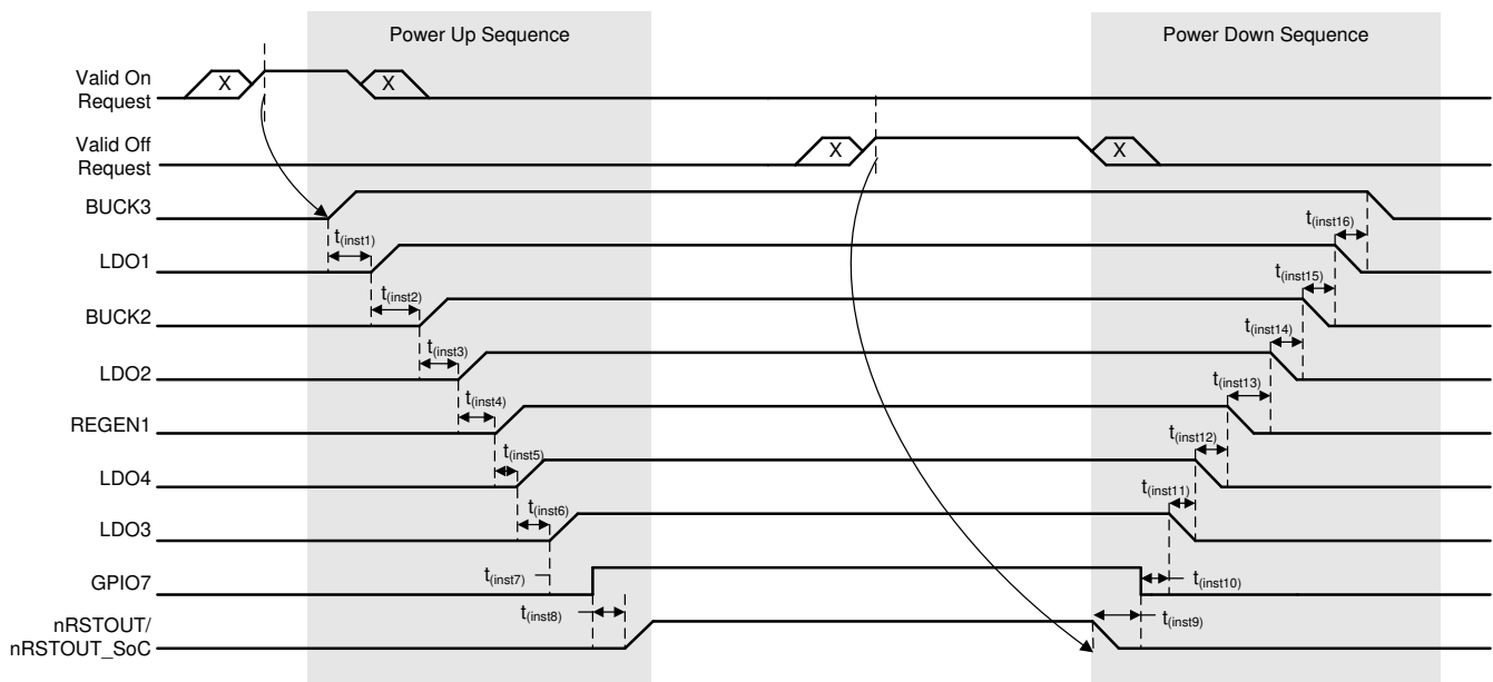
図 8-42. Power Sequence Example
