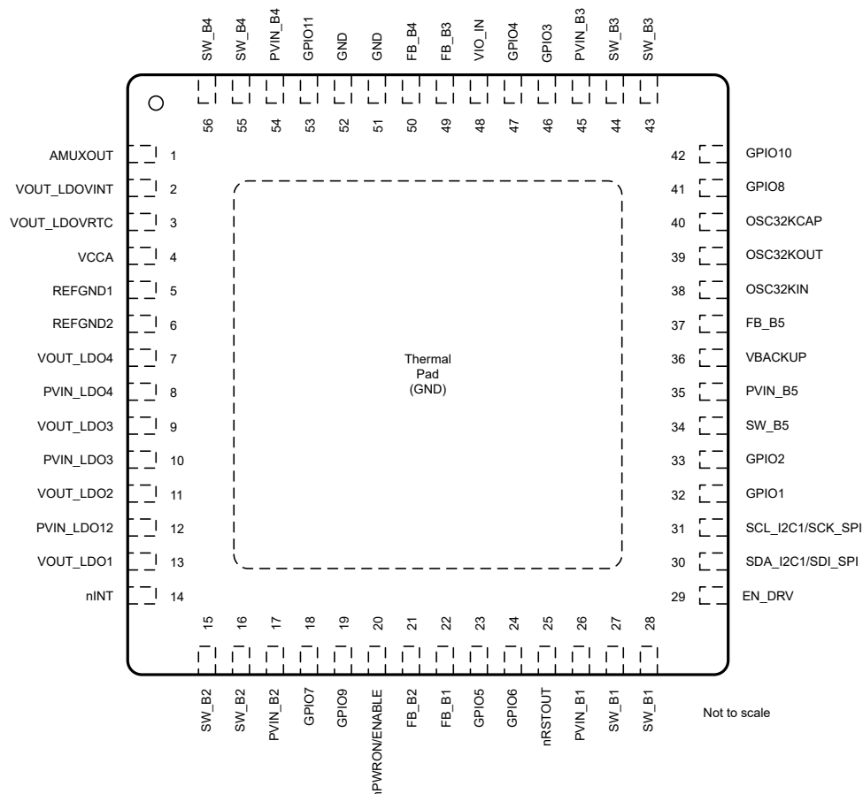
図 6-1. 56-Pin RWE (VQFNP) Package, 0.5-mm Pitch, With Thermal Pad (Top View)
