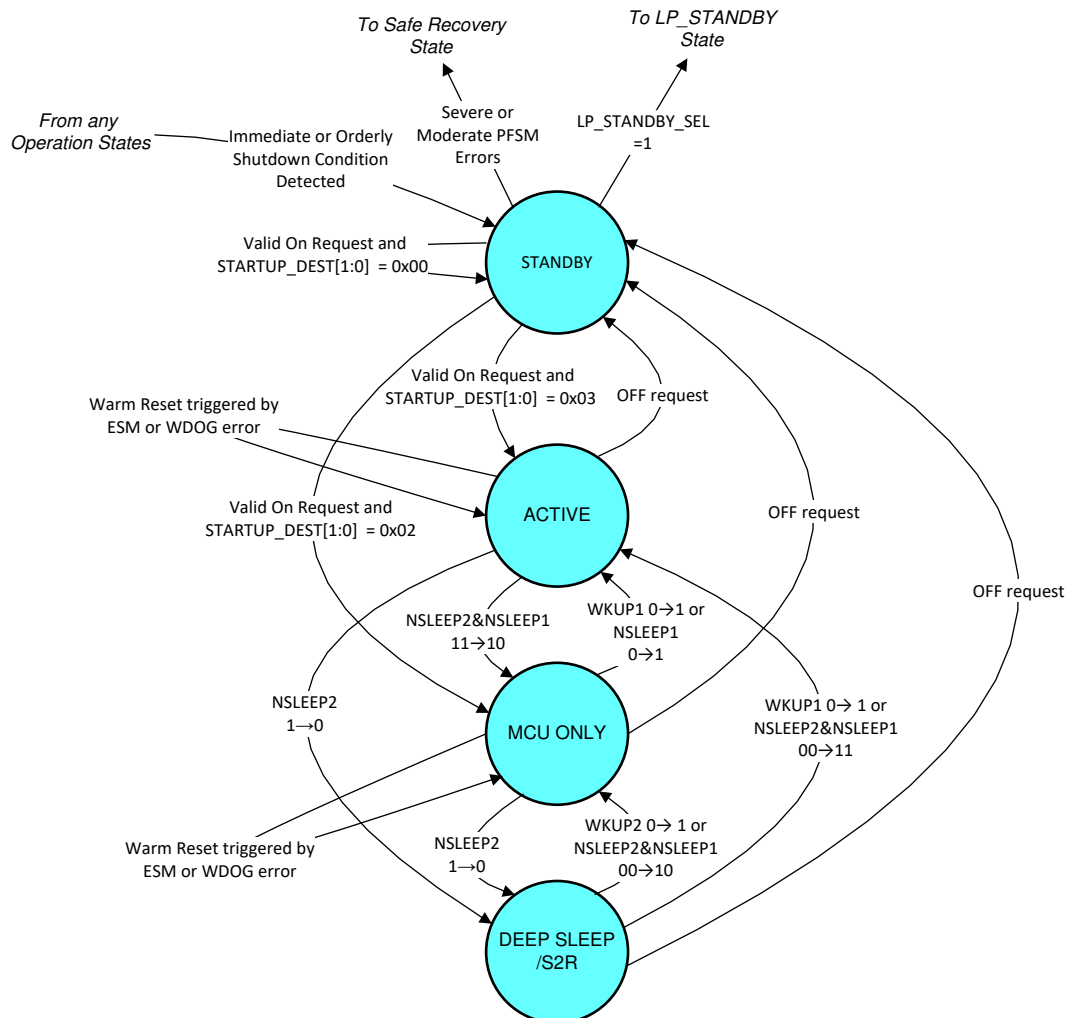
8-39. Example of a Mission State-Machine
