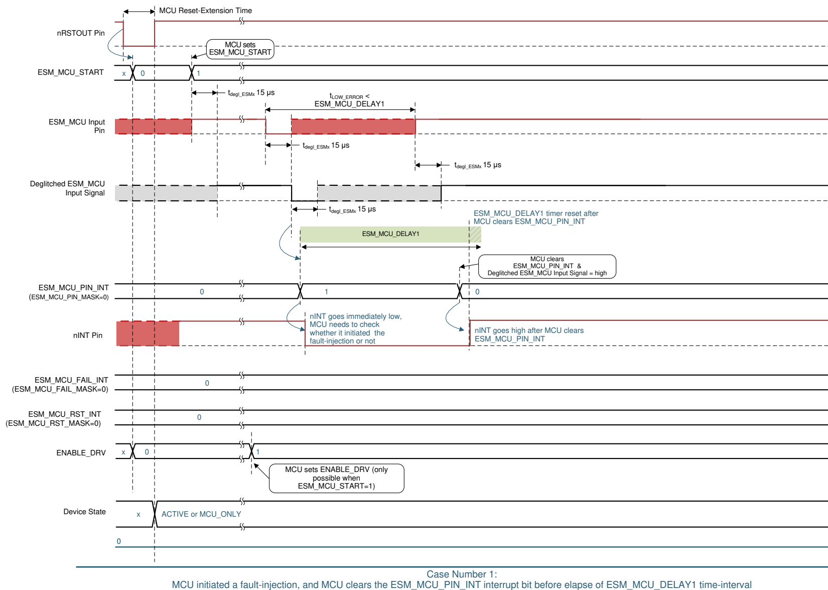
図 8-26. Example Waveform for ESM in Level Mode - Case Number 1: ESM_MCU Signal Recovers Before Elapse of Delay-1 time-interval
