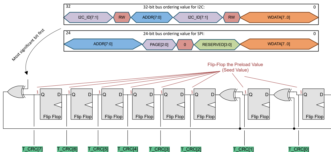
8-49. Calculation of 8-Bit CRC on Transmitted Data (T_CRC)
