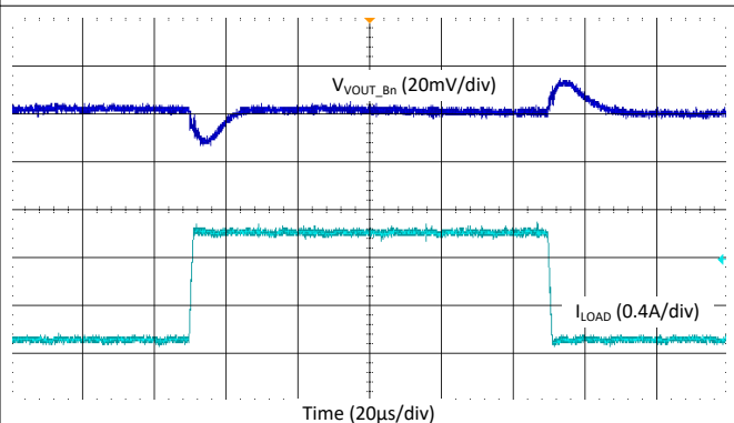
図 9-55. Buck Load Step Transient - Buck5, 4.4 MHz, Auto Mode
