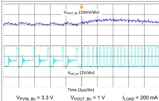
図 9-36. Buck Transient from PFM mode to PWM mode, 2.2 MHz, Single Phase
