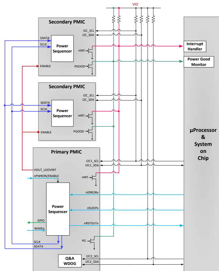
図 8-44. Multi-PMIC Pin Connections
