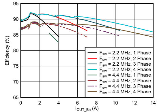
図 9-5. BUCK Efficiency with F_{sw} = 2.2\text{ MHz} or 4.4\text{ MHz}
