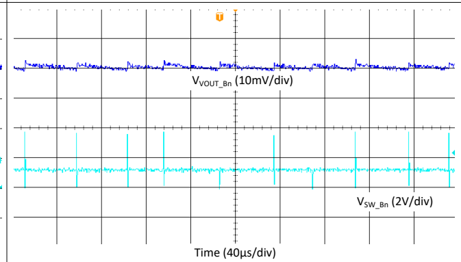
図 9-23. Buck Output Ripple - Single Phase, Fsw = 2.2 MHz, Forced-PWM Mode
