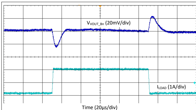
図 9-52. Buck Load Step Transient - Buck4, 2.2 MHz, Forced-PWM Mode
