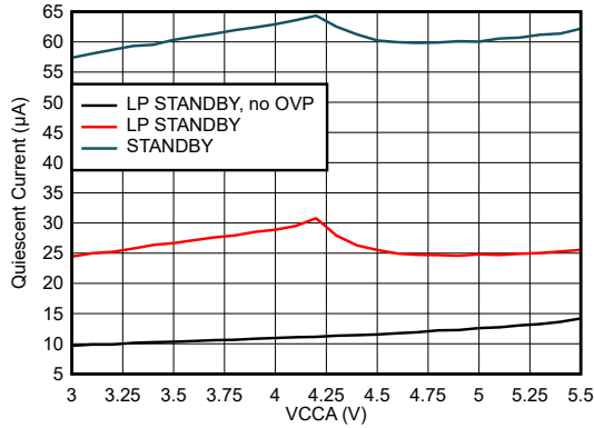
図 7-1. Quiescent Current vs Input Voltage
