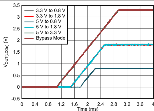
図 7-13. GPLDO Start-up with LDOn_SLOW_RAMP = 1
