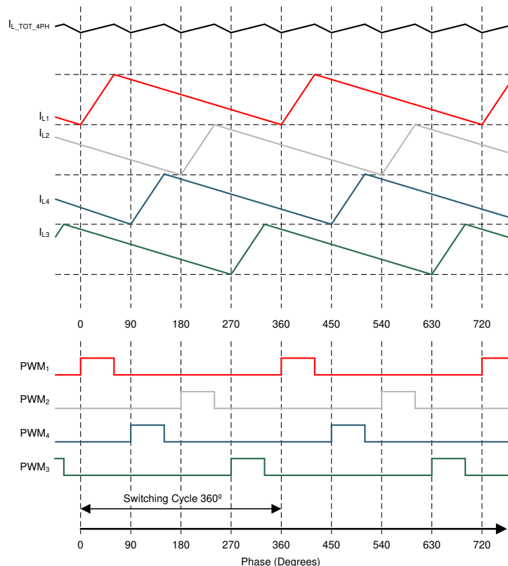
図 8-3. Example of PWM Timings, Inductor Current Waveforms, and Total Output Current in 4-Phase Configuration. 1
