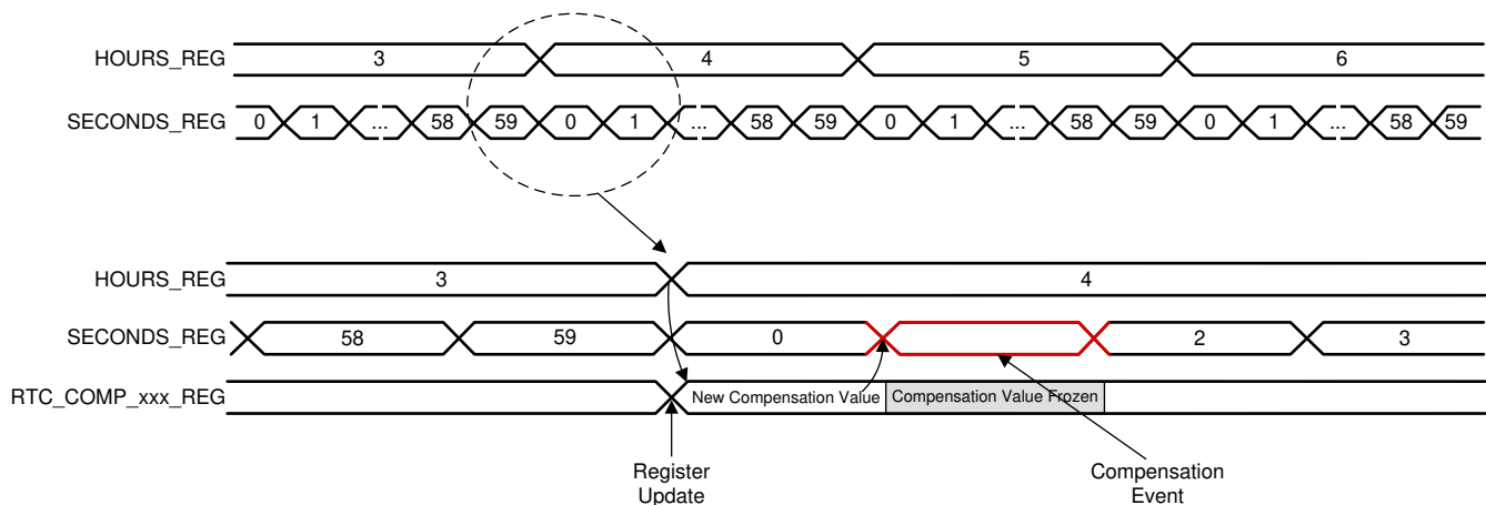
図 8-14. RTC Compensation Scheduling
