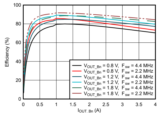
図 9-7. BUCK Efficiency in Varied Phase Configuration, 5 V Input
