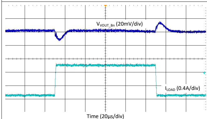
図 9-54. Buck Load Step Transient - Buck5, 2.2 MHz, Auto Mode
