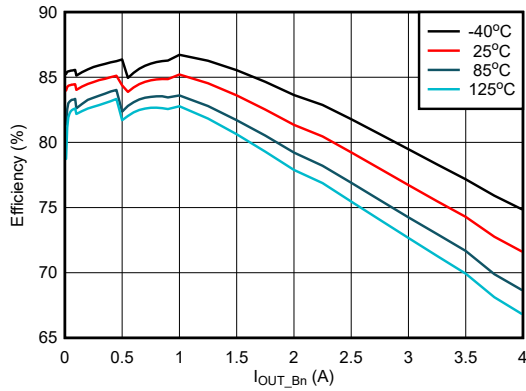
図 9-10. BUCK Efficiency at different T_A , Auto Mode
