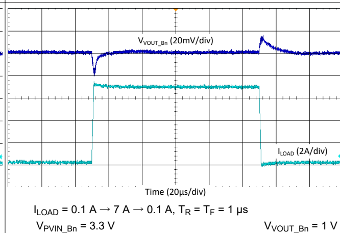
図 9-39. Buck Load Step Transient - 4-Phase, 4.4 MHz, Auto Mode
