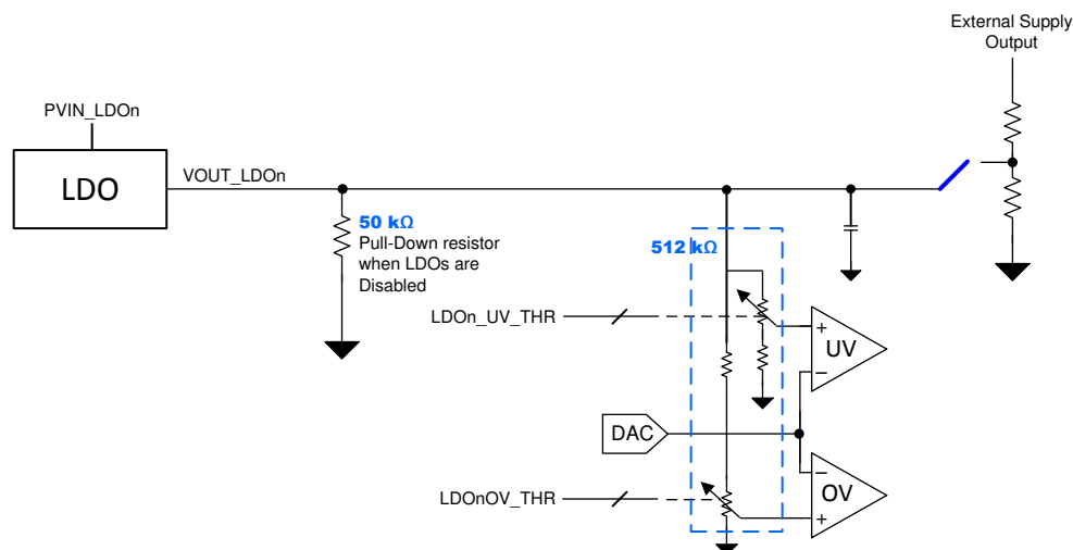
8-9. Impedance at the VOUT_LDOn Pins
