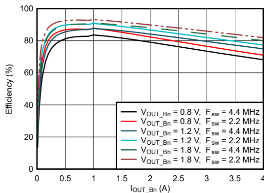
図 9-6. BUCK Efficiency in Varied Phase Configuration, 3.3 V Input
