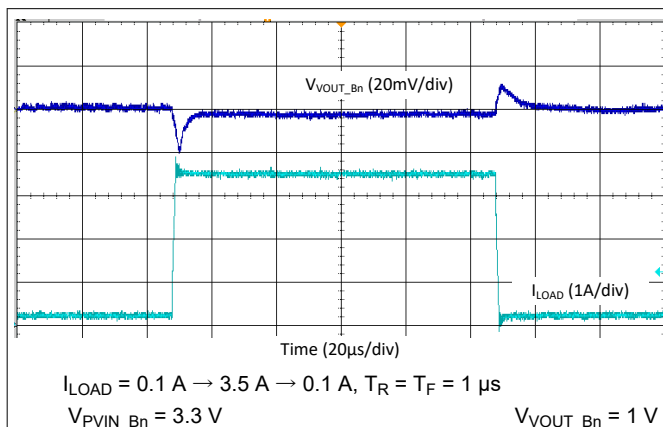
図 9-46. Buck Load Step Transient - 2-Phase, 2.2 MHz, Auto Mode
