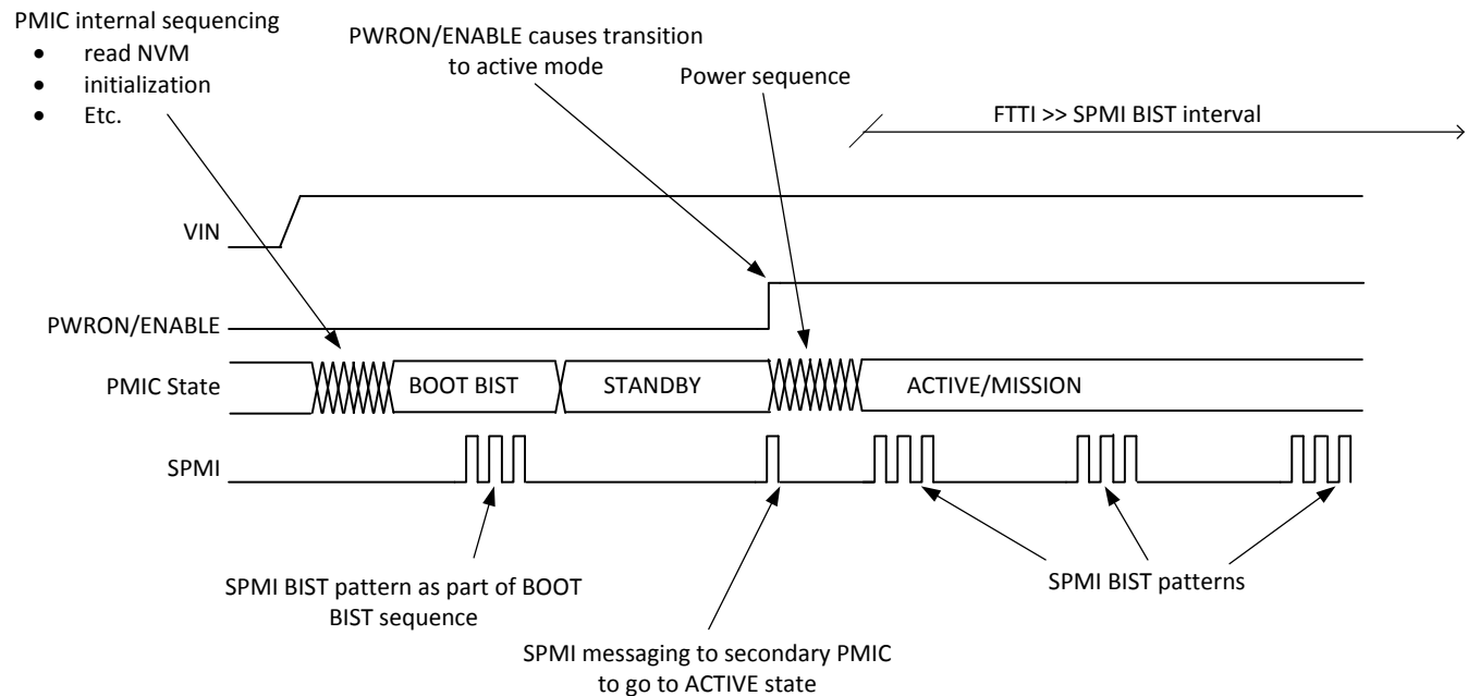
8-47. SPMI-BIST Operation
