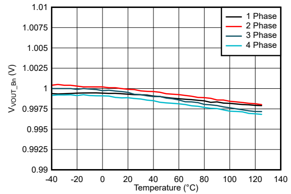
図 9-13. Buck Temperature Drift, Auto Mode, F_{sw} = 4.4\text{ MHz}
