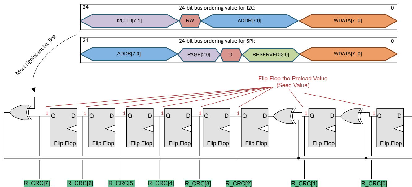
8-48. Calculation of 8-Bit CRC on Received Data (R_CRC)
