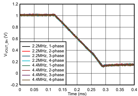
図 7-8. Buck Shutdown with no Load, Auto Mode
