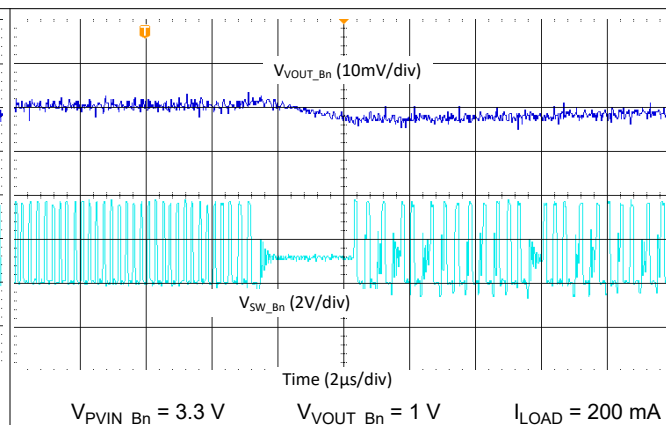
図 9-35. Buck Transient from PWM mode to PFM mode, 4.4 MHz, Single Phase
