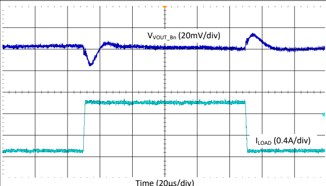
図 9-53. Buck Load Step Transient - Buck4, 4.4 MHz, Forced-PWM Mode
