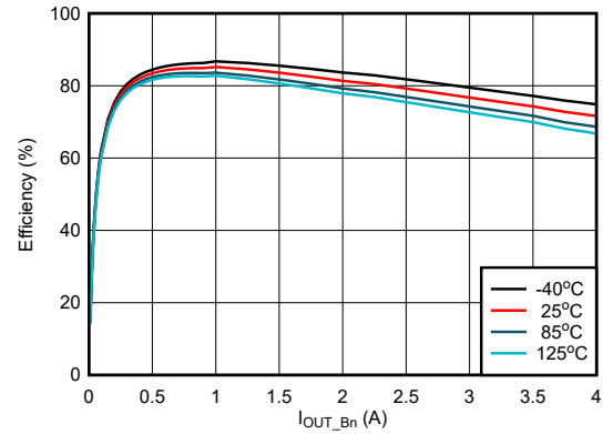
図 9-11. BUCK Efficiency at different T_A , Forced-PWM Mode
