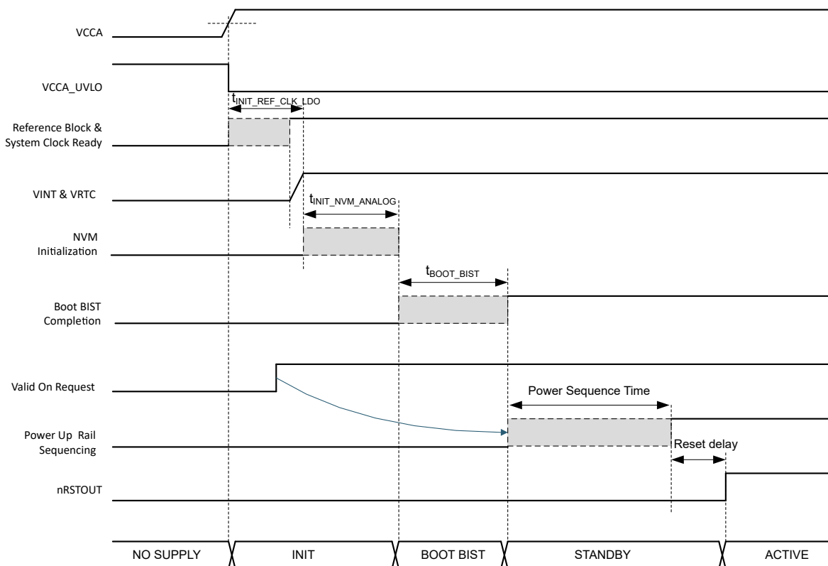
図 8-41. Device Start-up Timing Diagram
