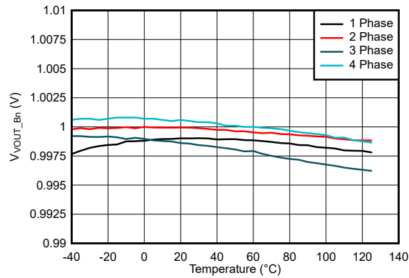
図 9-12. Buck Temperature Drift, Auto Mode, F_{sw} = 2.2\text{ MHz}
