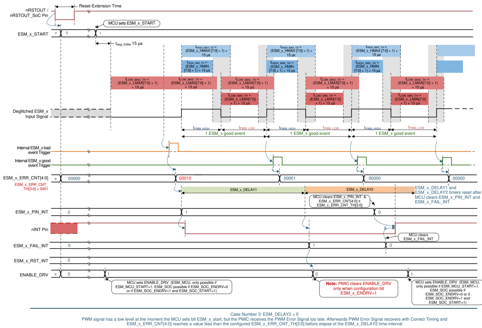
図 8-34. Example Waveform for ESM in PWM Mode – Case Number 3: ESM Starts with Low-Level at Deglitched Input Signal, but Receives Too Late a Correct PWM Signal Afterwards (The _x stand for _MCU or _SoC)
