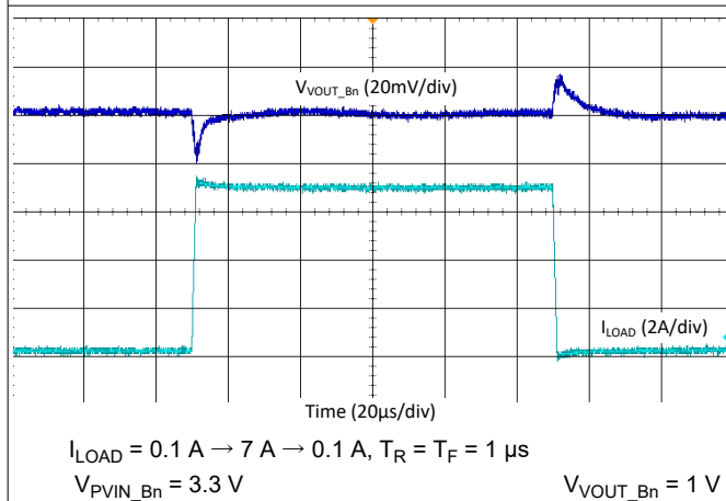
図 9-38. Buck Load Step Transient - 4-Phase, 2.2 MHz, Auto Mode
