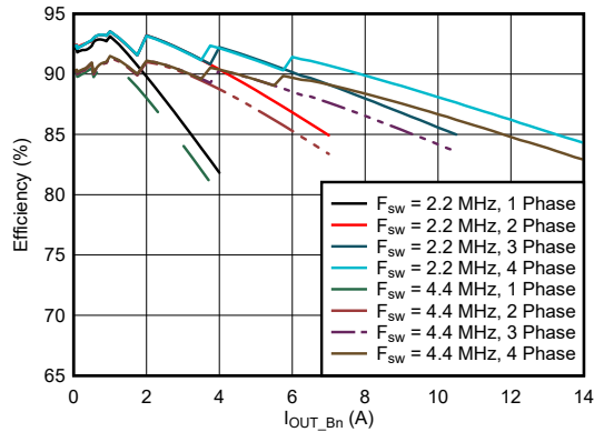
図 9-4. BUCK Efficiency at 3.3 V or 5 V Input Voltage
