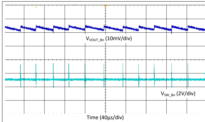
図 9-22. Buck Output Ripple - Single Phase, Auto Mode
