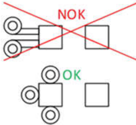
9-69. Ground connection of capacitor at VOUT_LDOVINT pin
