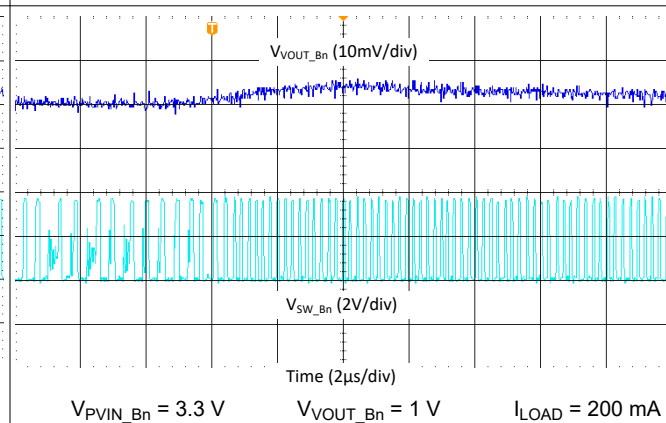
図 9-37. Buck Transient from PFM mode to PWM mode, 4.4 MHz, Single Phase
