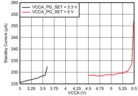
図 7-2. Standby Current with VCCA Monitor
