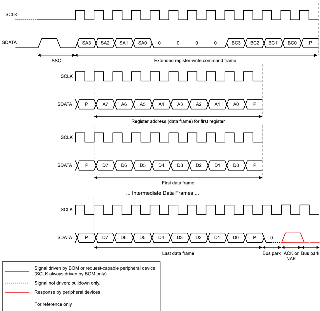
8-46. SPMI Extended Register Write Command
