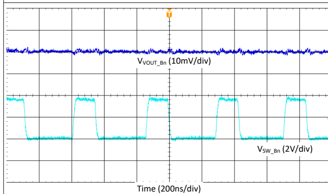
図 9-24. Buck Output Ripple - Single Phase, Fsw = 4.4 MHz, Forced-PWM Mode
