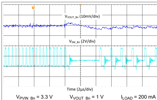
図 9-34. Buck Transient from PWM mode to PFM mode, 2.2 MHz, Single Phase
