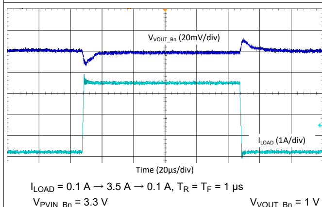
図 9-48. Buck Load Step Transient - 2-Phase, 2.2 MHz, Forced-PWM Mode
