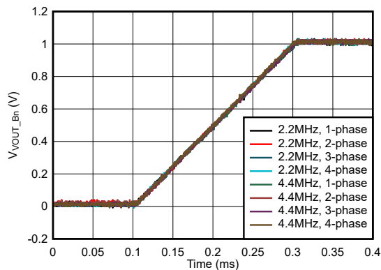
図 7-7. Buck Start-up with 1A Load, Auto Mode
