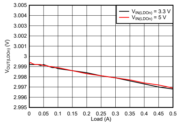
図 9-59. LDO1/2/3 Load Regulation, V_{out} = 3\text{ V}
