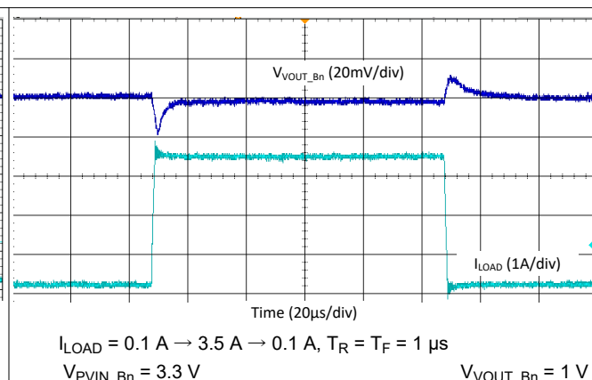
図 9-47. Buck Load Step Transient - 2-Phase, 4.4 MHz, Auto Mode
