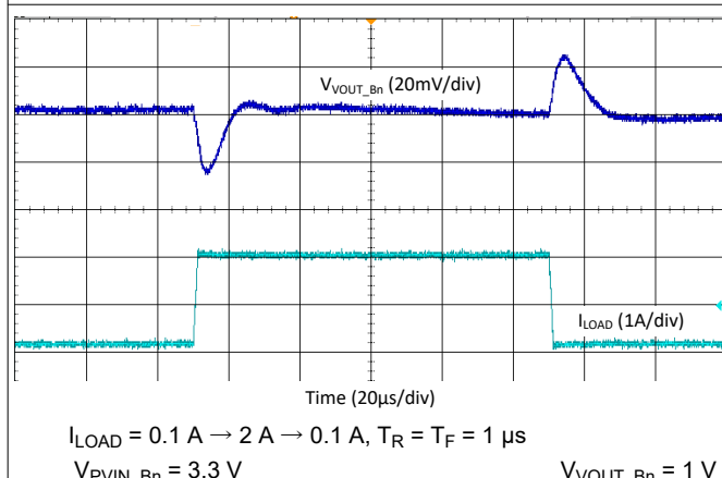
図 9-50. Buck Load Step Transient - Buck4, 2.2 MHz, Auto Mode
