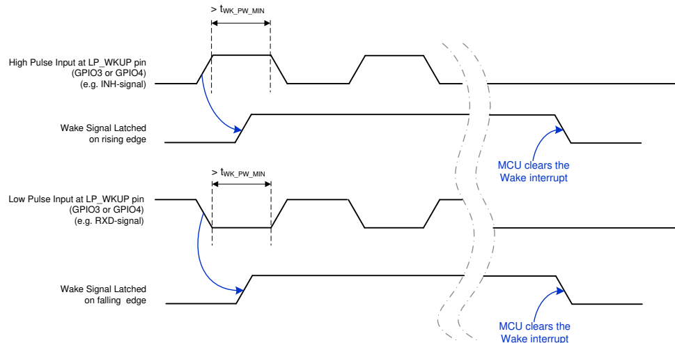
図 8-40. CAN Wake-Up Timing Diagram
