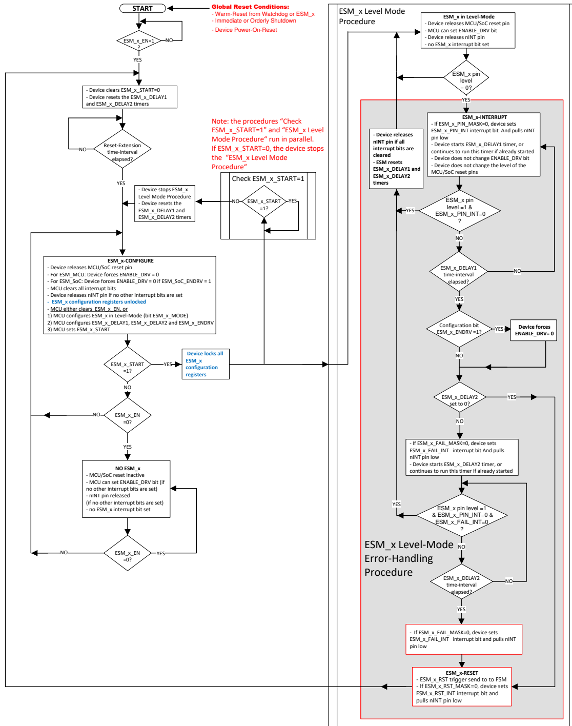
図 8-25. Flow Chart for Error Detection in Level Mode
