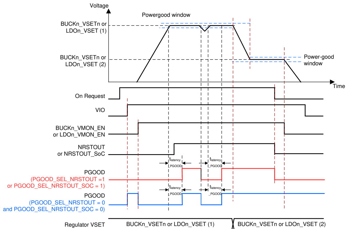
8-11. PGOOD Waveforms
