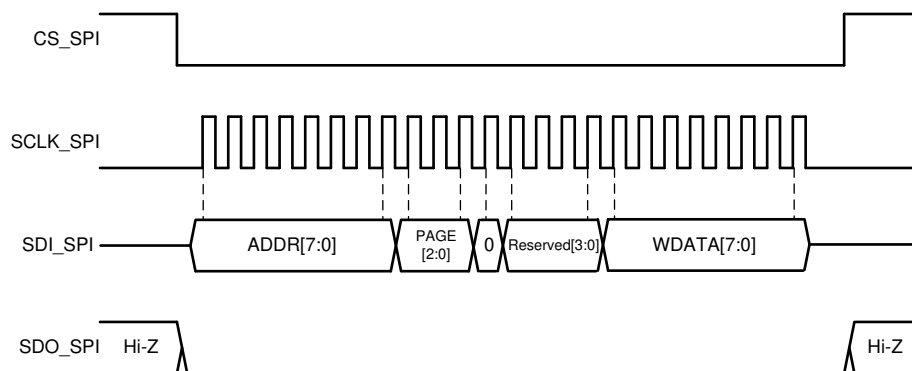
図 8-58. SPI Write Cycle
