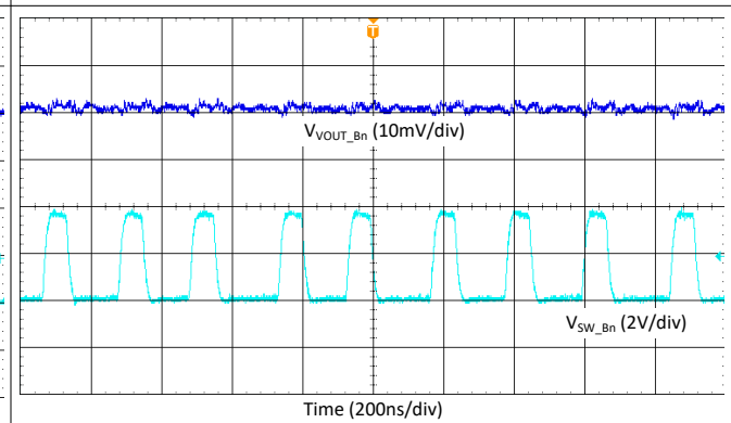
図 9-27. Buck Output Ripple - 2-Phase, Fsw = 4.4 MHz, Forced-PWM Mode
