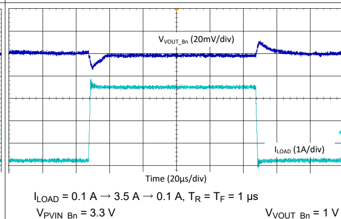
図 9-49. Buck Load Step Transient - 2-Phase, 4.4 MHz, Forced-PWM Mode
