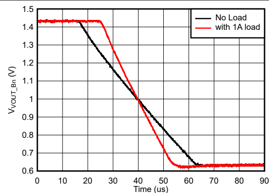
図 7-9. Buck Shutdown with 1A Load, Auto Mode
