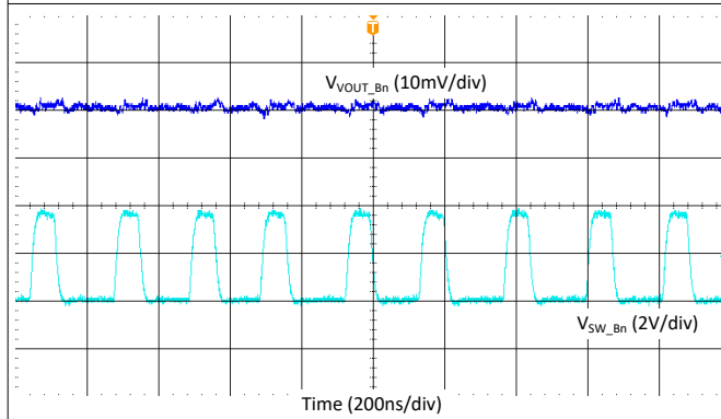
図 9-24. Buck Output Ripple - Single Phase, Fsw = 4.4 MHz, Forced-PWM Mode
