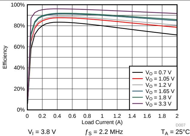
FIG 4-10. SMPS Efficiency for SMPS5 in PWM Mode
