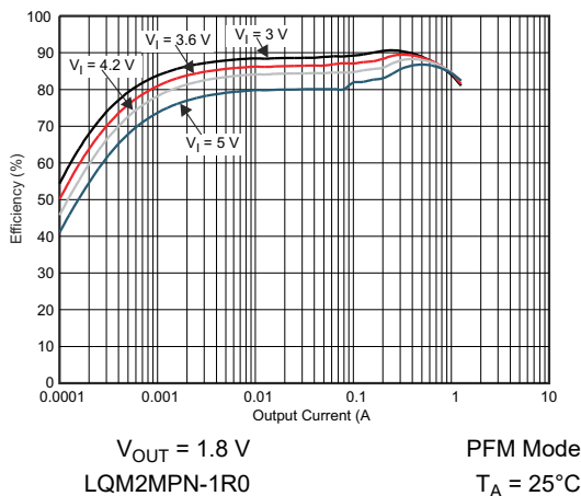
FIG 6-7. DCDC2 Efficiency vs Output Current
