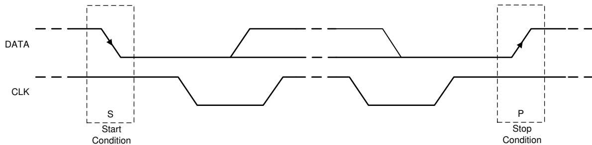
8-19. START and STOP Conditions
