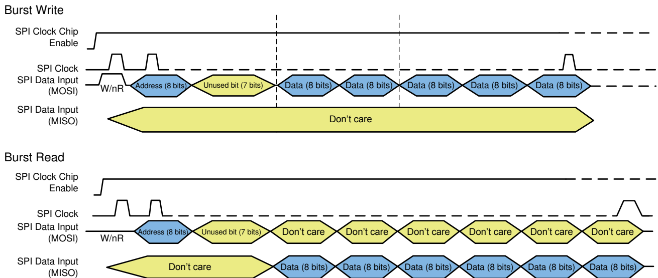
8-18. SPI BURST READ and BURST WRITE Protocol
