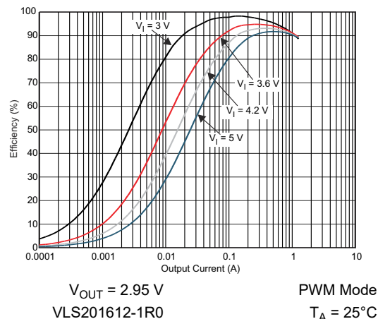
FIG 6-12. DCDC2 Efficiency vs Output Current
