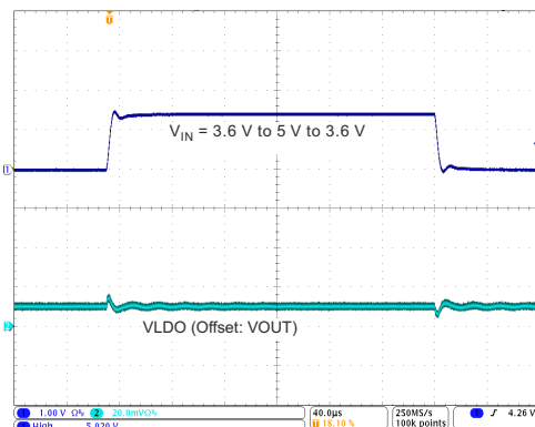
9-15. LDO4, LDO5 Line Transient Response
