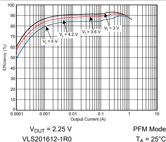
FIG 6-9. DCDC2 Efficiency vs Output Current
