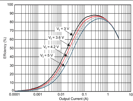
V_{OUT} = 1.2\text{ V} LQM2MPN-1R0 PWM Mode T_A = 25^\circ\text{C}
