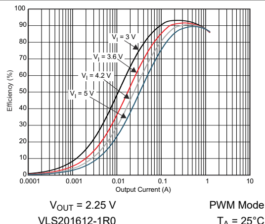
FIG 6-10. DCDC2 Efficiency vs Output Current
