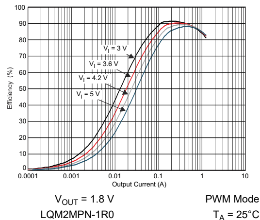
FIG 6-8. DCDC2 Efficiency vs Output Current
