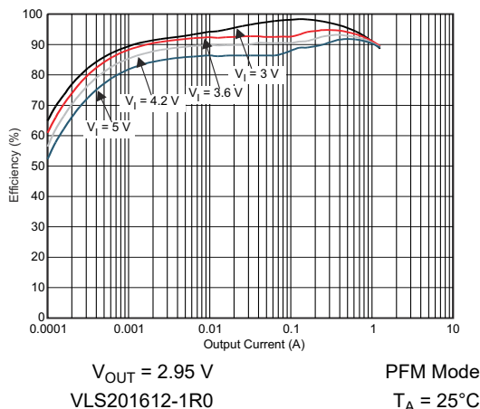
FIG 6-11. DCDC2 Efficiency vs Output Current
