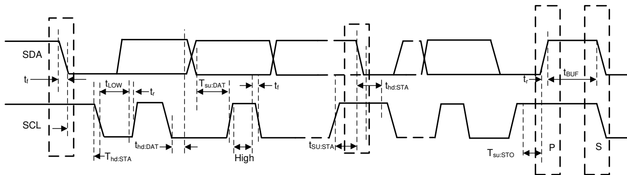
FIG 7-1. Serial Interface Timing Diagram for FS-Mode
