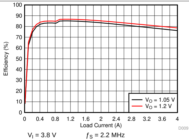
图 5-5. SMPS Efficiency for 4-A Multi-Phase PWM Mode
