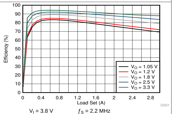
FIG 5-13. SMPS Efficiency for 3-A Single-Phase PWM Mode
