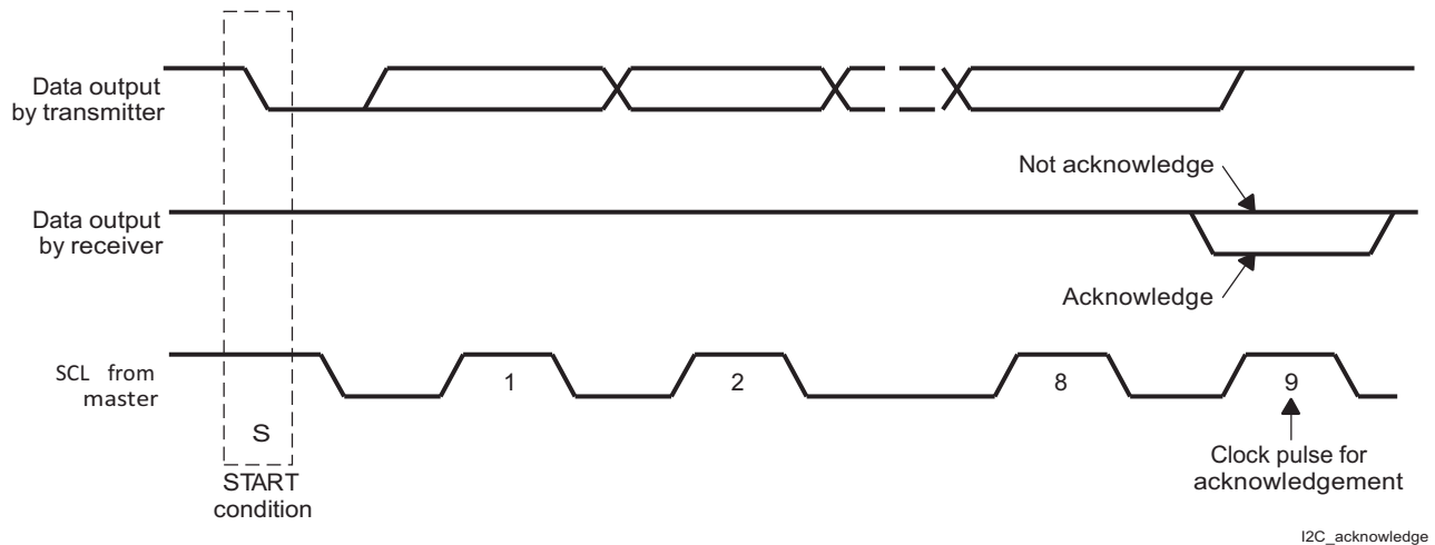
❏ 6-13. Acknowledge on the I 2 C Bus
