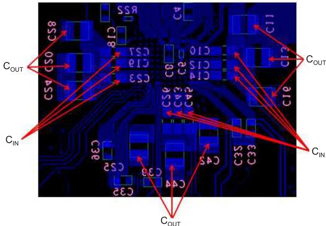
FIG 9-5. Bottom Layer Overview of Input and Output Capacitor Placement
