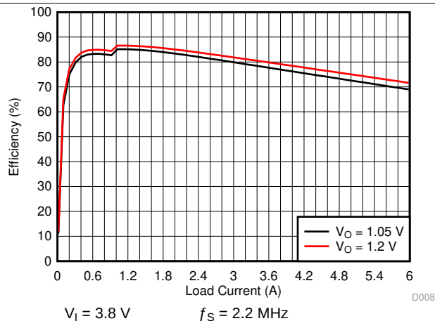
图 5-6. SMPS Efficiency for 6-A Multi-Phase PWM Mode
