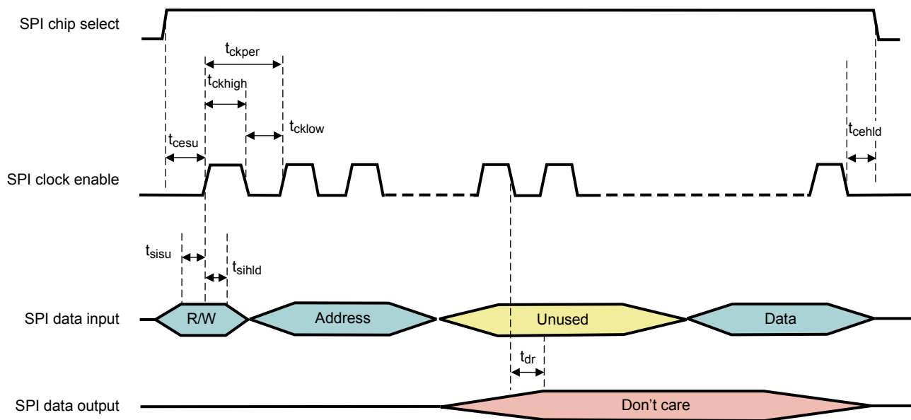
❏ 5-3. SPI Interface Timing Diagram
