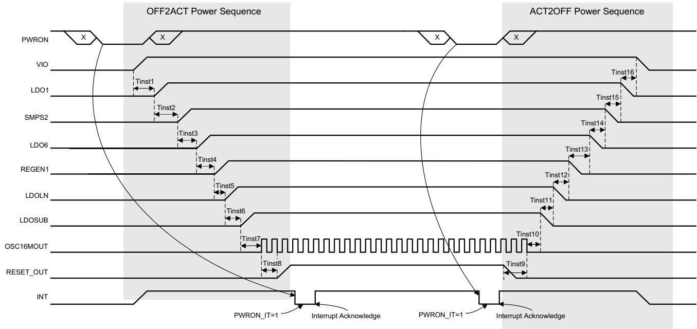
FIG 6-19. Power Sequence Example
