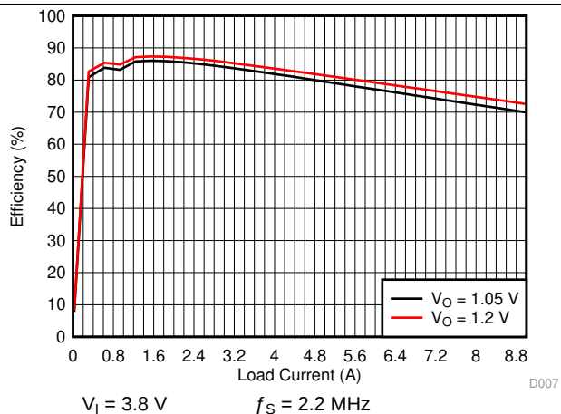
图 5-7. SMPS Efficiency for 9-A Multi-Phase PWM Mode
