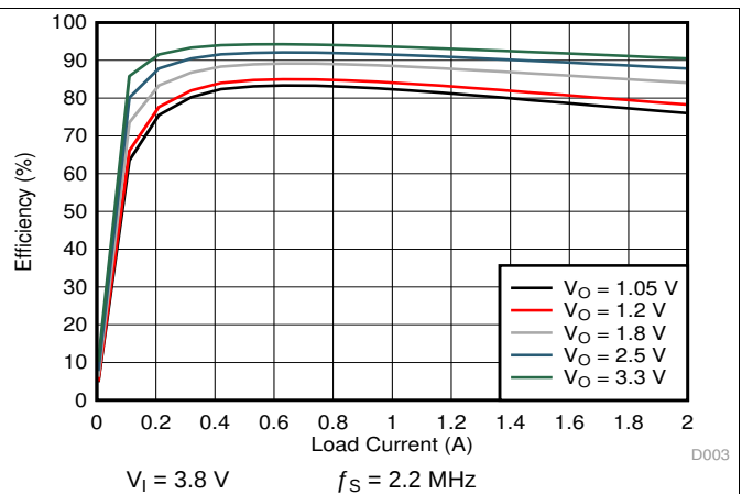
FIG 5-11. SMPS Efficiency for 2-A Single-Phase PWM Mode
