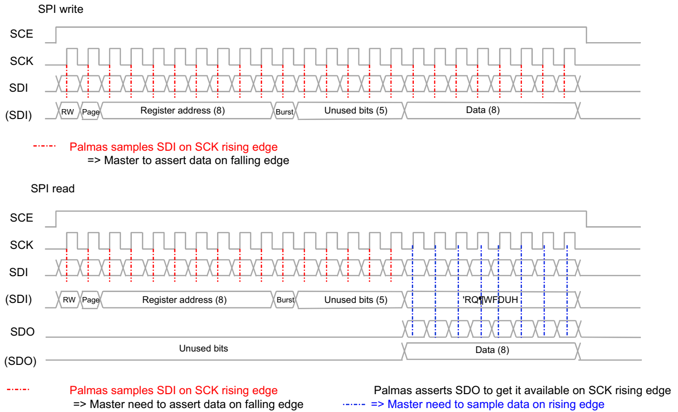
✎ 6-15. SPI Single Read and Write Access
