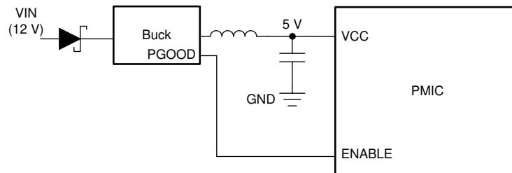
7-4. Supporting Uncontrolled Power Down when the PMIC is Supplied by a Preregulator
