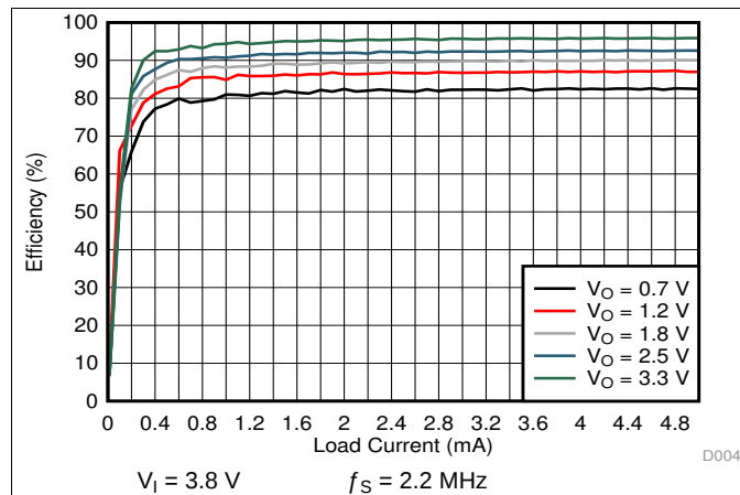
FIG 5-10. SMPS Efficiency for 2-A Single-Phase ECO-mode
