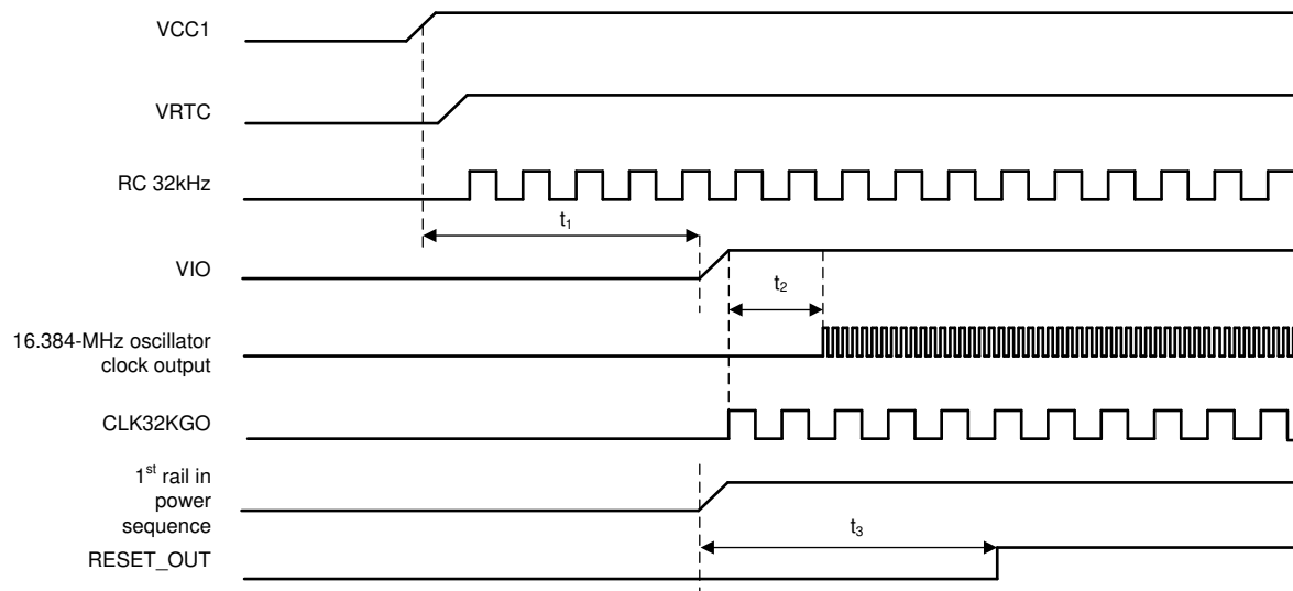
FIG 6-20. Start Up Timing Diagram
