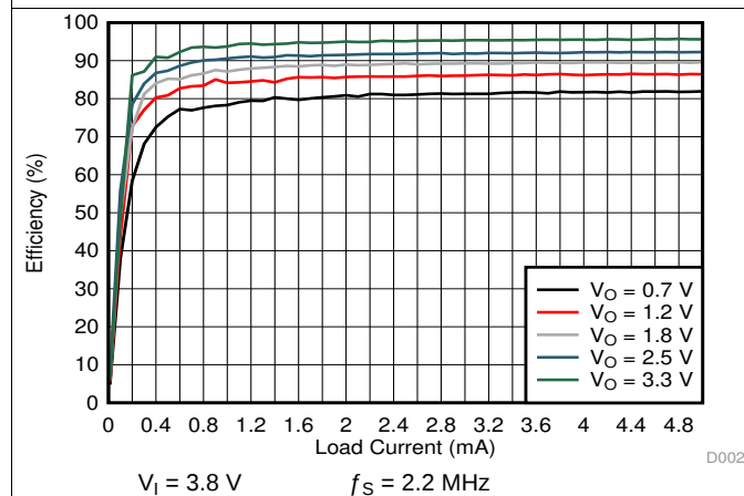
FIG 5-12. SMPS Efficiency for 3-A Single-Phase ECO-mode
