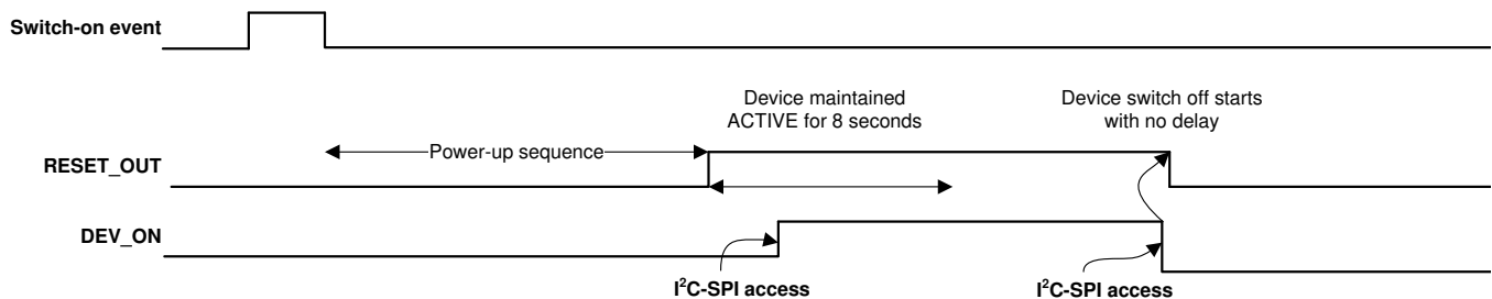
FIG 6-23. DEV_ON Mode Timing Diagrams
