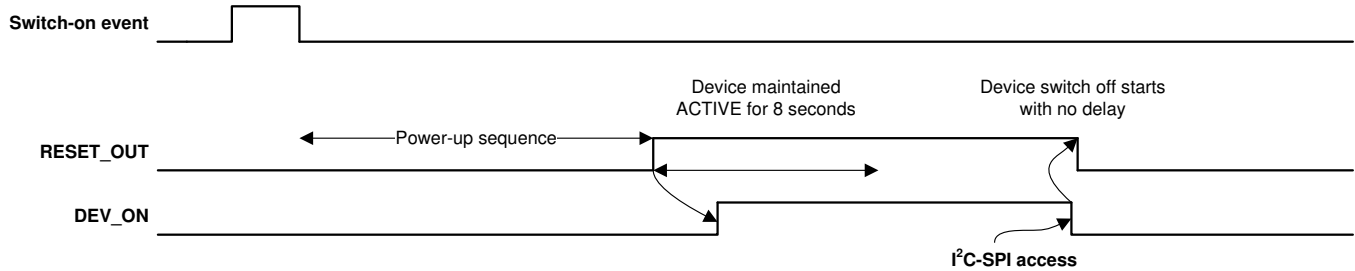
FIG 6-22. AUTODEVON Mode Timing Diagrams
