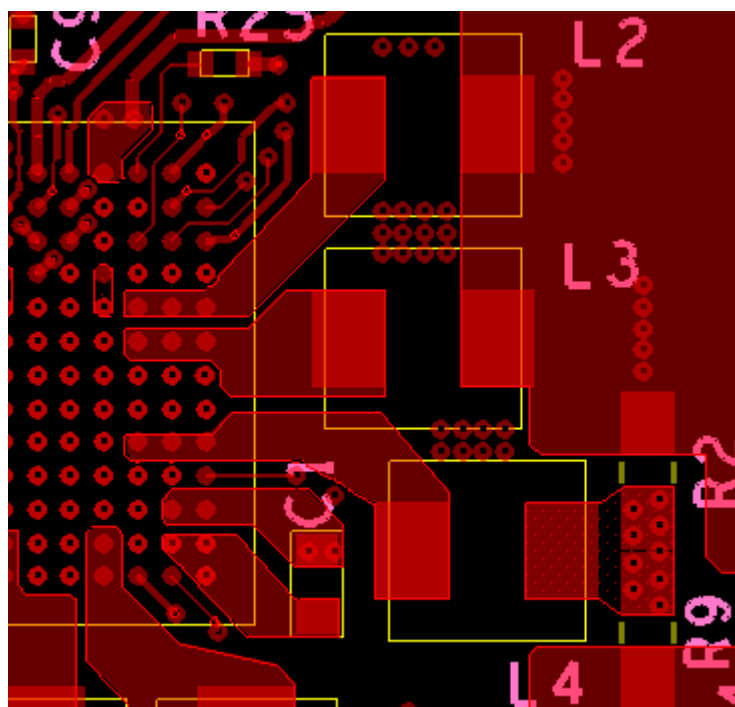
FIG 9-6. Top Layer Zoomed View of SMPS123 SW Connections to Inductors
