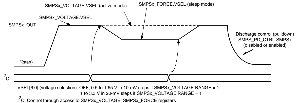
Figure 5-4. DVS - SMPS Controls Voltage Control Through I²C (SMPSx_CTRL.ROOF_FLOOR_EN = 0)
