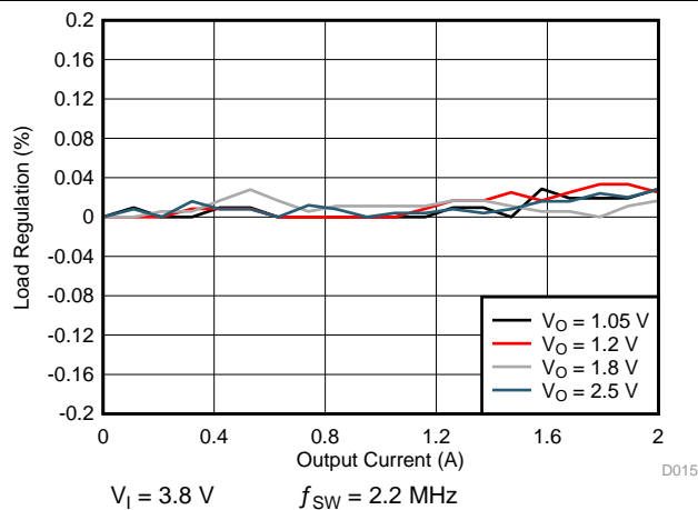
图 6-11. SMPS Regulation for 2-A Single Phase
