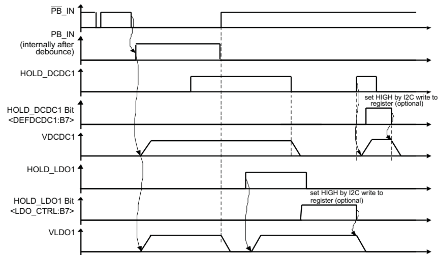
Figure 17. \overline{\text{PB\_IN}} Timing
