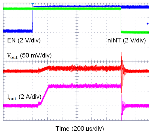
Figure 41. Buck Start-up With Short on Output
