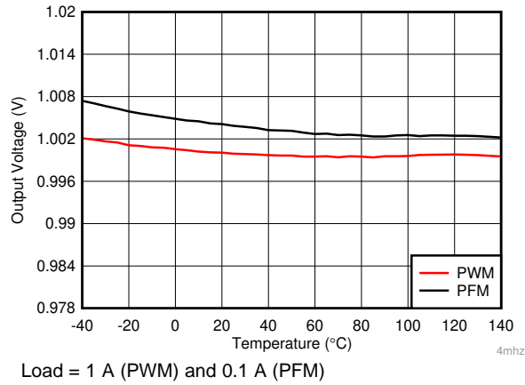
Figure 29. Buck Output Voltage vs Temperature
