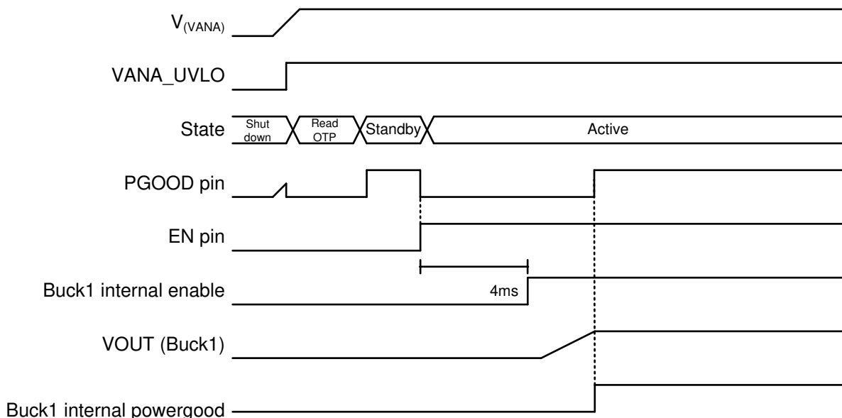
Figure 13. PGOOD Pin Operation in Continuous Mode
