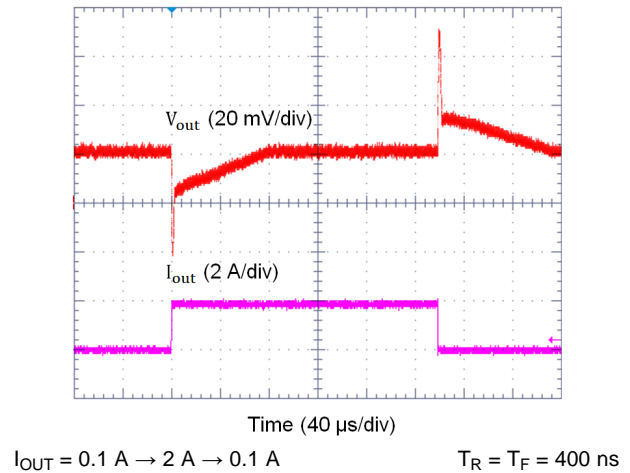
Figure 38. Buck Transient Load Step Response, Forced PWM Mode
