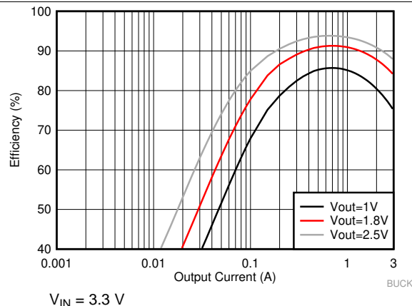
Figure 24. Buck Efficiency in Forced PWM Mode
