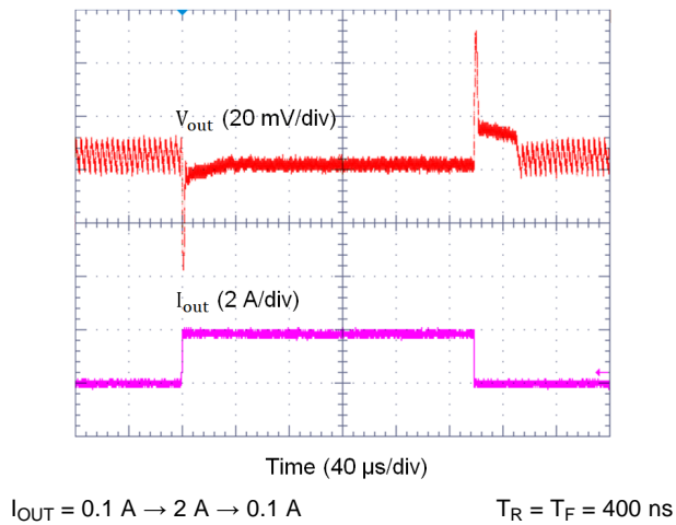
Figure 37. Buck Transient Load Step Response, AUTO Mode
