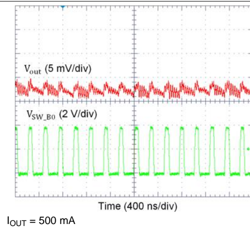
Figure 34. Buck Output Voltage Ripple, Forced PWM Mode
