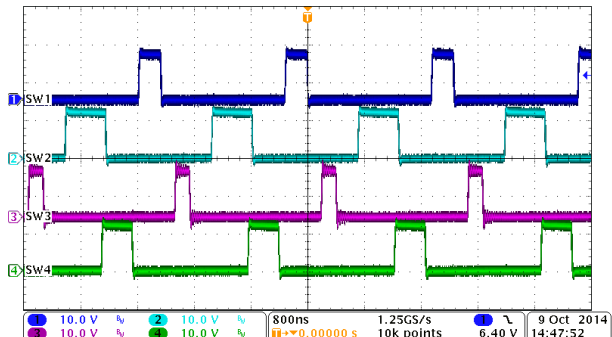
9-4. Phase Shift Between Channels
