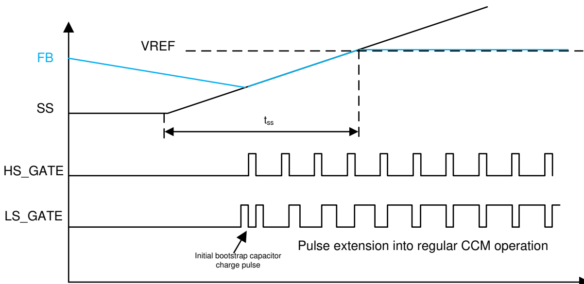
FIG 8-5. Soft-Start Under Prebiased Condition and CCM Mode Programmed
