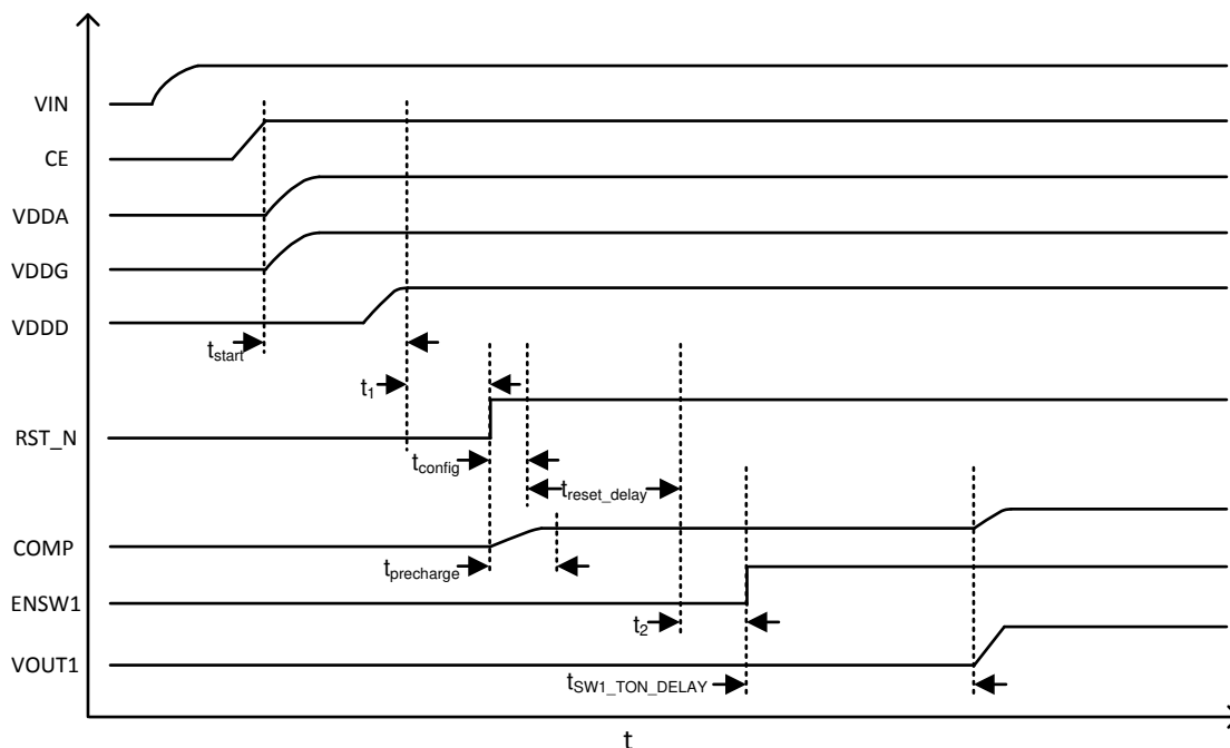
Figure 8-3. Timing Showing Startup from CE
