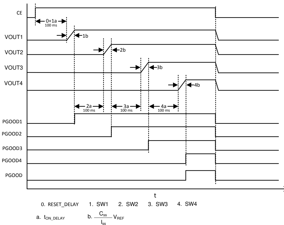
9-14. Example Timing Diagram for External Sequencing Through VOUT
