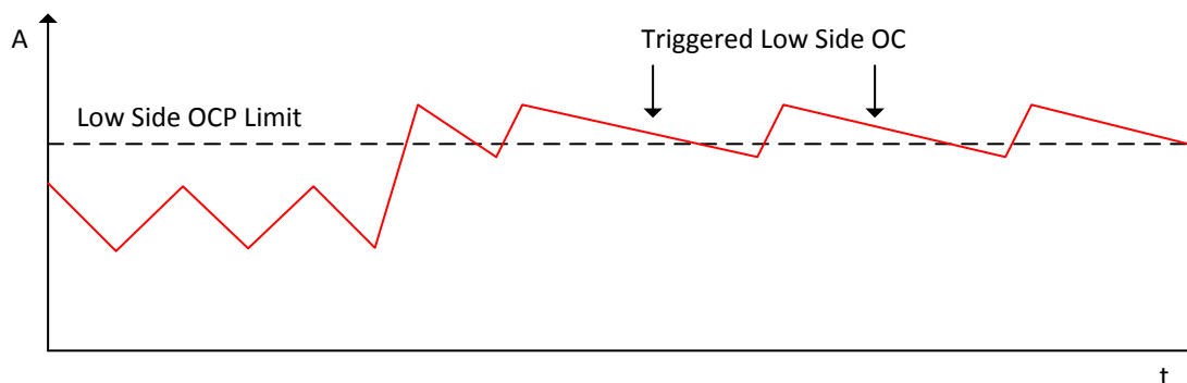
FIG 8-12. Inductor Current During Overcurrent Event With Low-Side Detection
