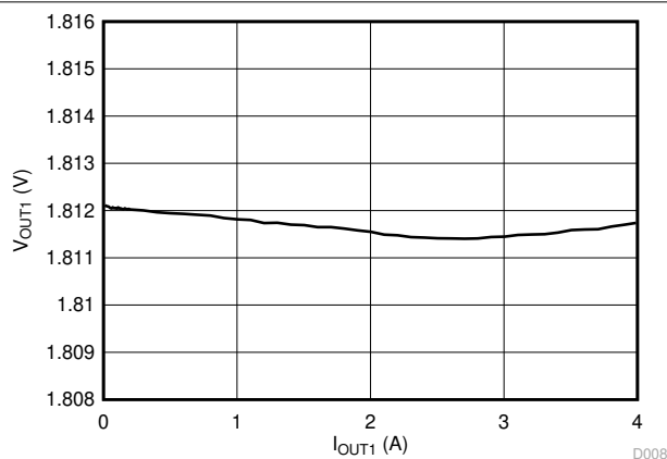
9-7. V_{OUT1} Load Regulation
