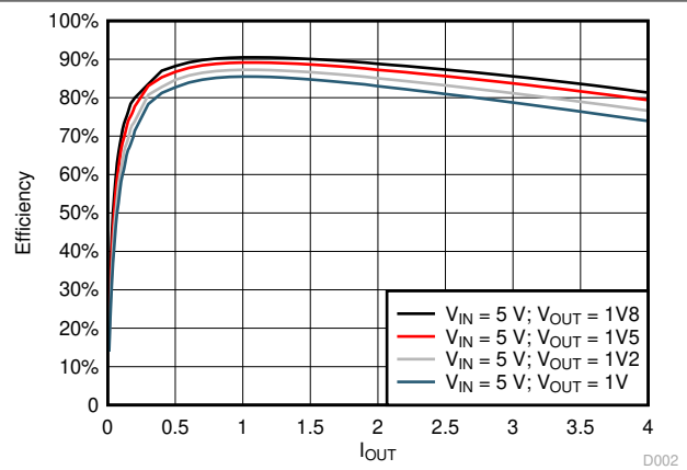
7-2. Buck1 and Buck2 Power Efficiency, V_{IN} = 5\text{ V}
