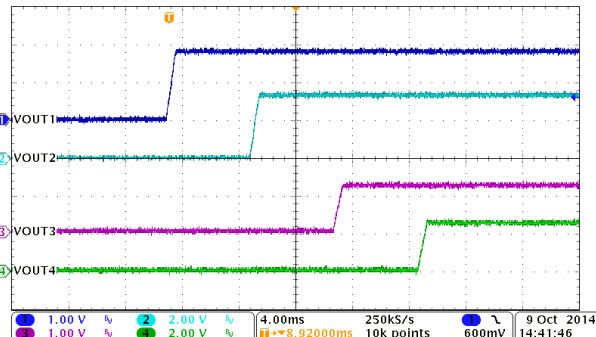
9-3. Configurable Power-Up Sequence
