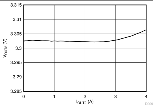
9-8. V_{OUT2} Load Regulation
