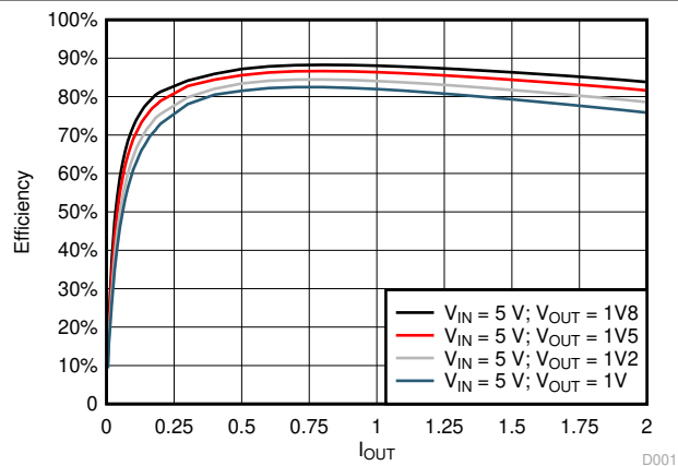
7-4. Buck3 and Buck4 Power Efficiency, V_{IN} = 5 V
