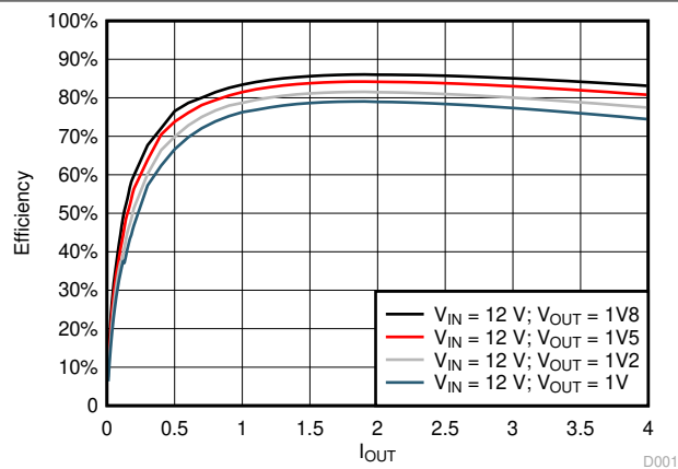
7-1. Buck1 and Buck2 Power Efficiency, V_{IN} = 12\text{ V}
