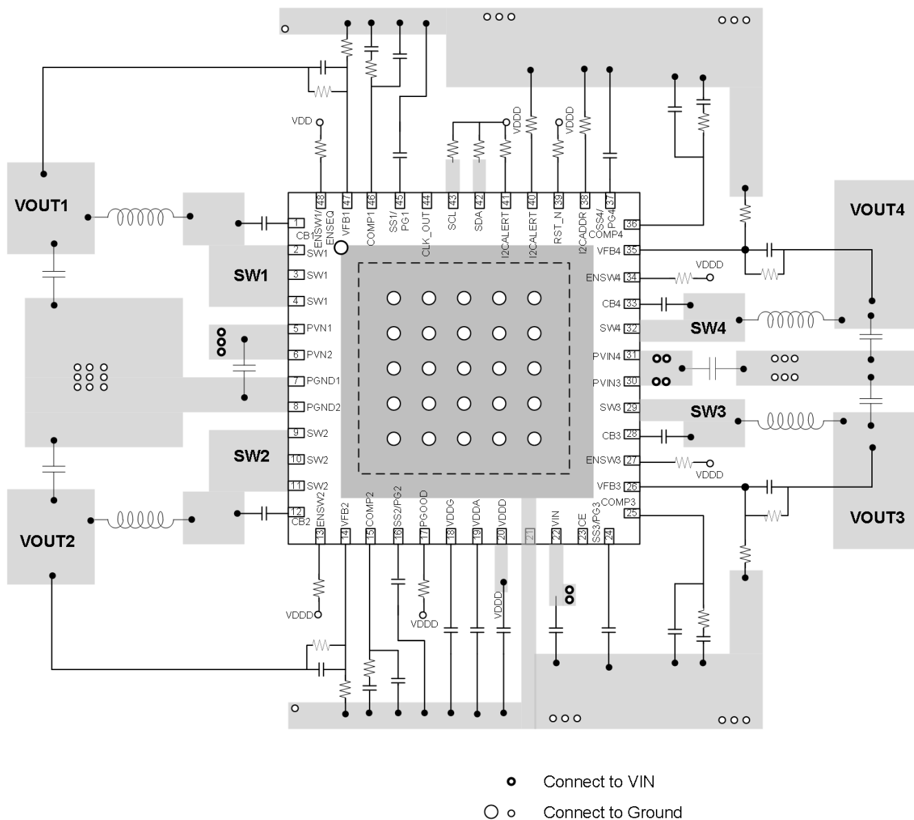
11-1. Layout Schematic
