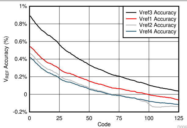
9-5. V_{REF} Accuracy vs Code
