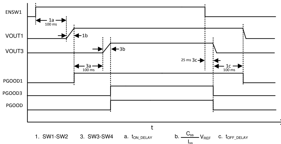
FIG 9-12. Example Timing Diagram for Current Sharing With Single-Pin Enable
