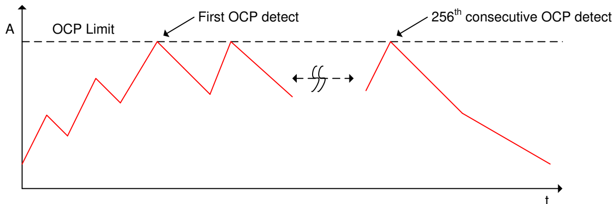
FIG 8-11. Inductor Current During Overcurrent Event
