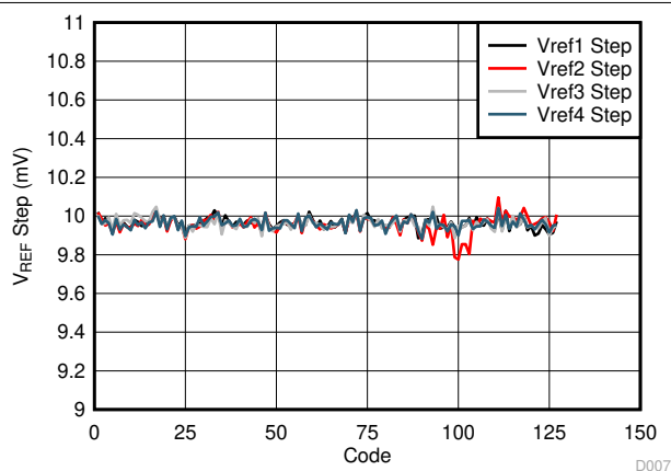
9-6. V_{REF} Step Accuracy vs Code
