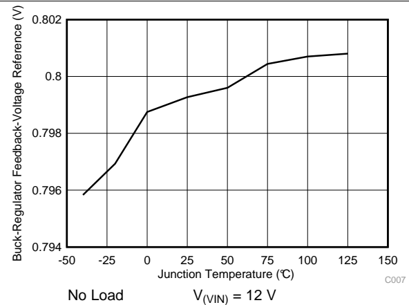
FIG 4. Buck-Regulator Feedback-Voltage Reference ( V_{(FB1)} ) vs Junction Temperature
