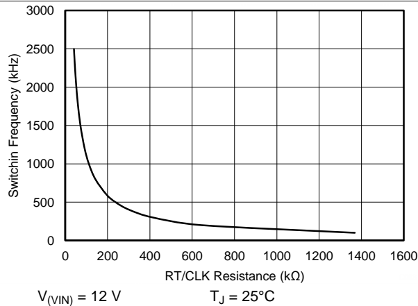
FIG 3. Buck-Regulator Switching Frequency vs R_{T\_CLK} Resistance
