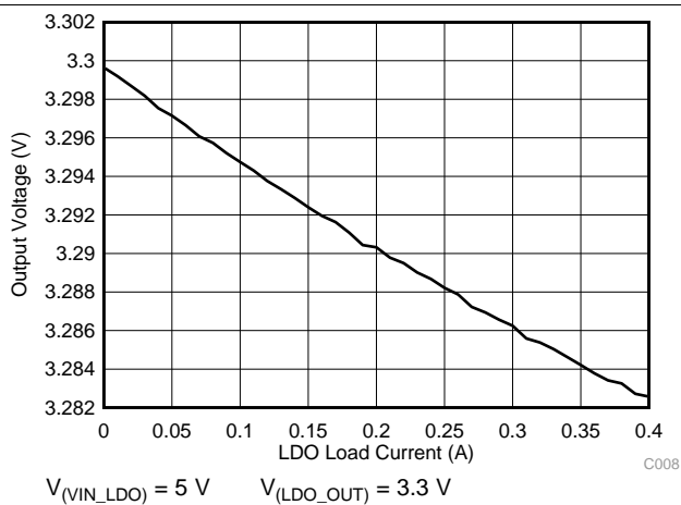
FIG 5. LDO-Regulator Load Regulation
