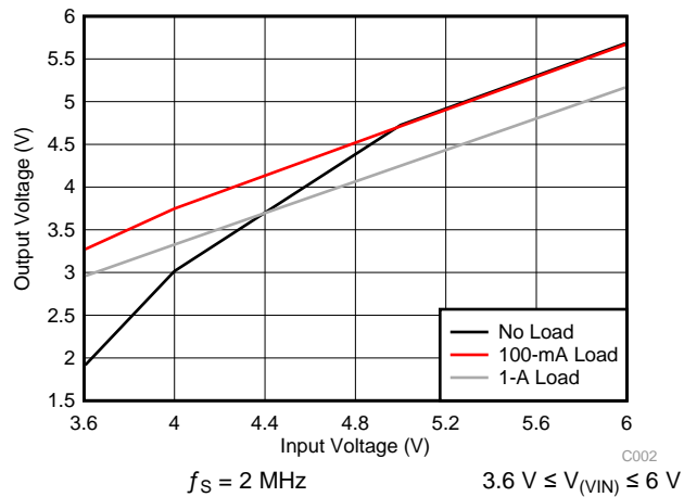
FIG 1. Maximum-Possible Buck-Regulator Output Voltage
