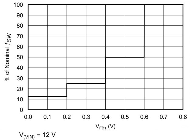
FIG 2. Buck-Regulator Switching Frequency vs V_{(FB1)} Feedback Voltage
