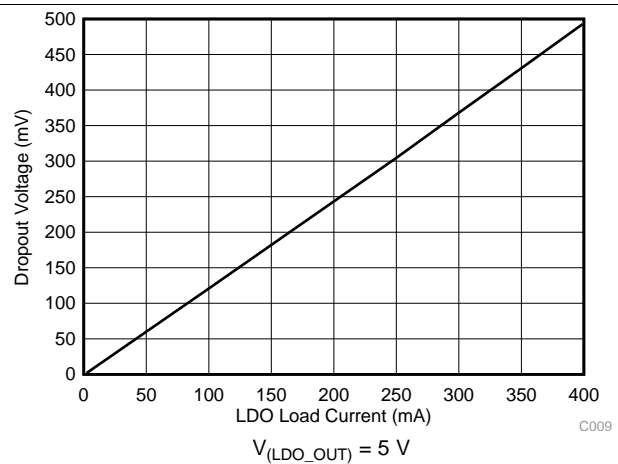
FIG 6. LDO-Regulator Dropout Voltage vs Load Current
