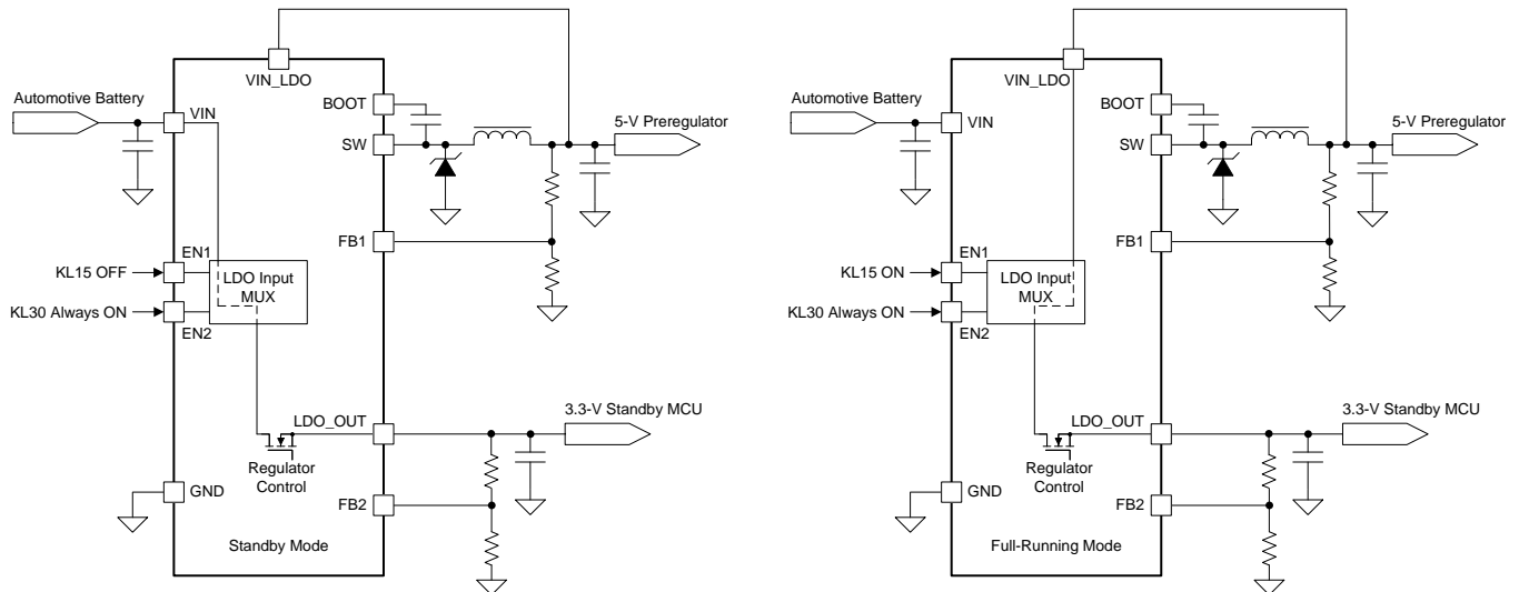
FIG 15. Example of LDO Auto Source in Standby Condition
