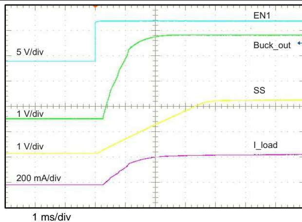
图 24. Buck-Regulator Startup Operation
