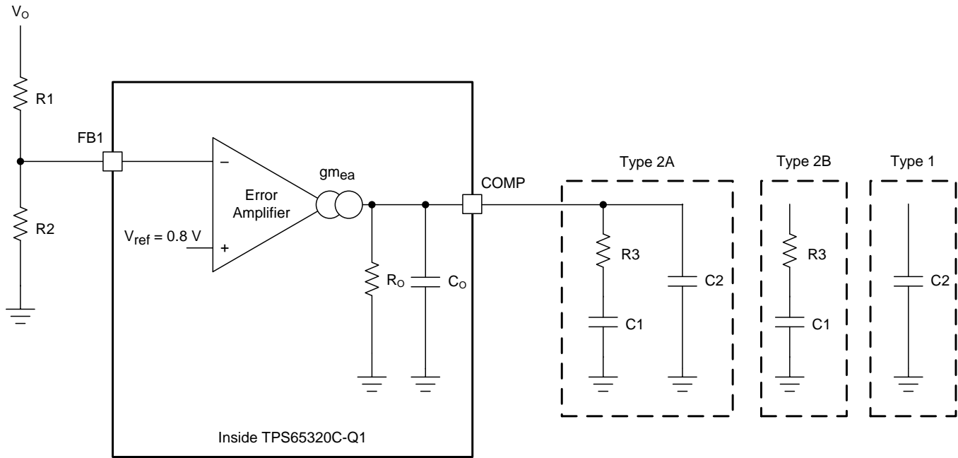
FIG 12. Types of Frequency Compensation
