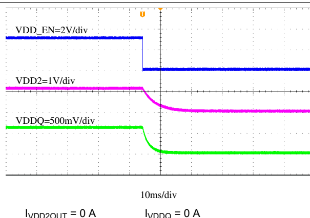
8-24. VDDQ Shutdown Through VDD_EN
