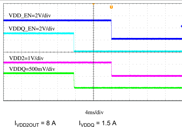
8-21. VDDQ Shutdown Through VDDQ_EN
