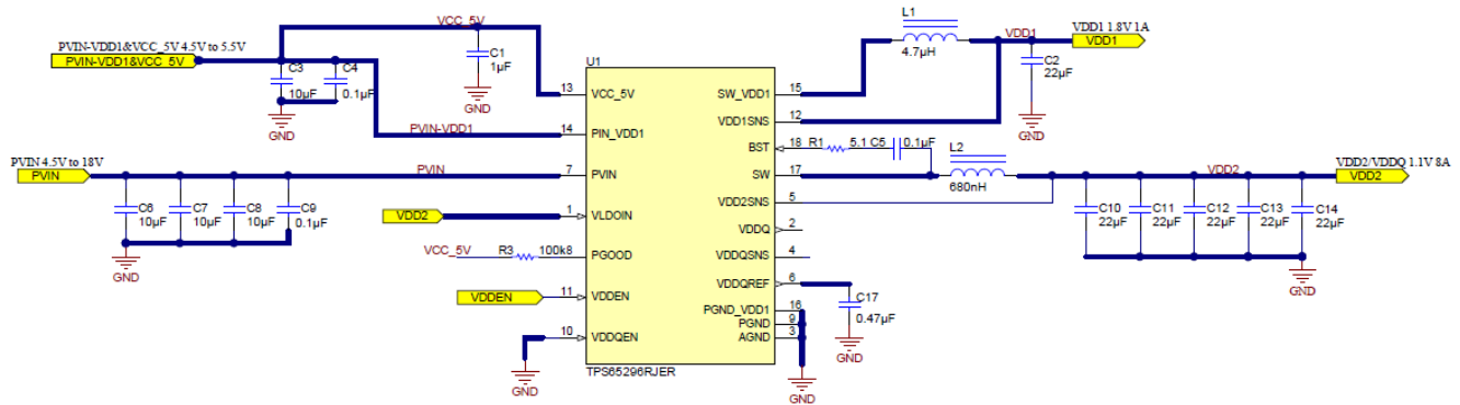
❏ 8-2. LPDDR4 Application Schematic
