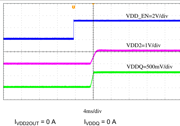
8-22. VDDQ Start-Up Through VDD_EN
