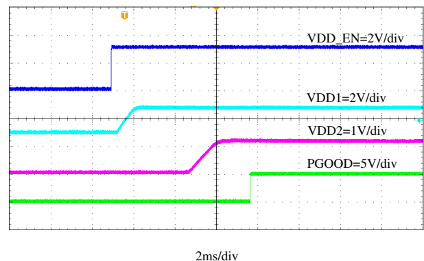
8-14. Start-Up Through VDD_EN, I_{VDD1OUT} = 0 A , I_{VDD2OUT} = 0 A
