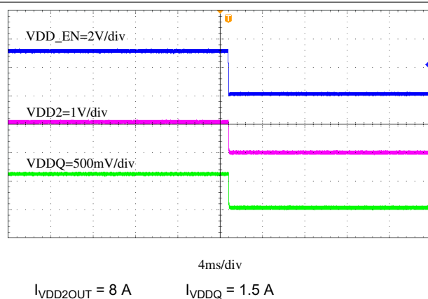
8-25. VDDQ Shutdown Through VDD_EN
