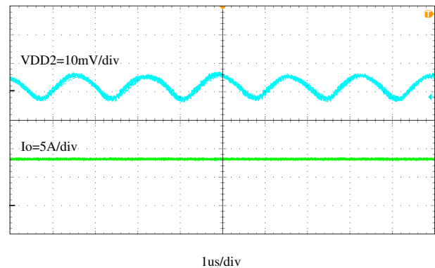
8-12. VDD2 Output Voltage Ripple, I_{OUT} = 8 A
