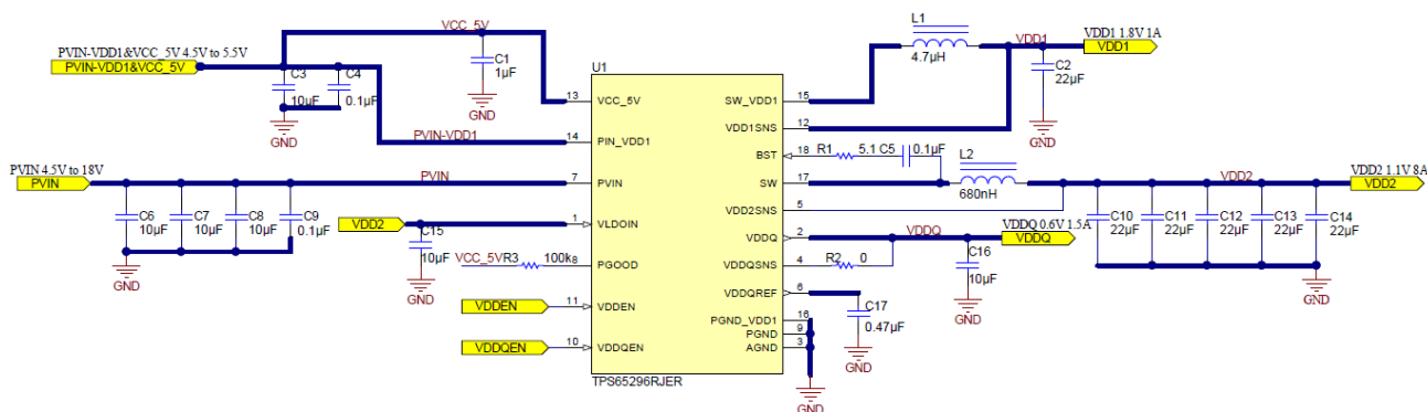
8-1. LPDDR4X Application Schematic
