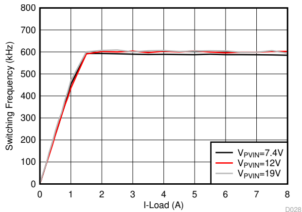
6-26. VDD2 Switching Frequency vs Load Current
