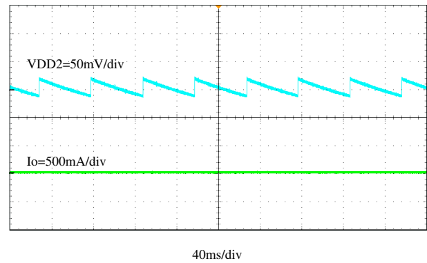
8-10. VDD2 Output Voltage Ripple, I_{OUT} = 0 A
