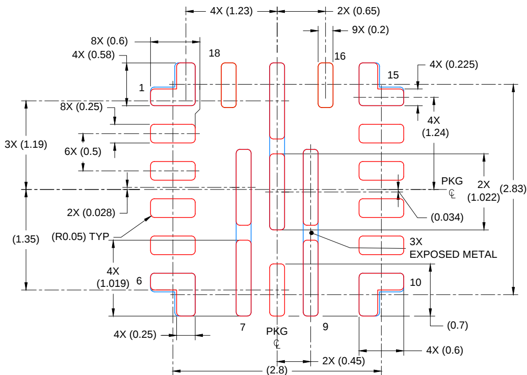
SOLDER PASTE EXAMPLE BASED ON 0.1 mm THICK STENCIL PRINTED SOLDER COVERAGE BY AREA UNDER PACKAGE PADS 1, 6, 10 & 15: 93% & PADS 7-9, 17: 89% SCALE: 20X
