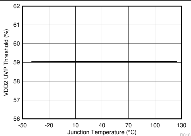
6-16. VDD1 UVP Threshold vs Junction Temperature
