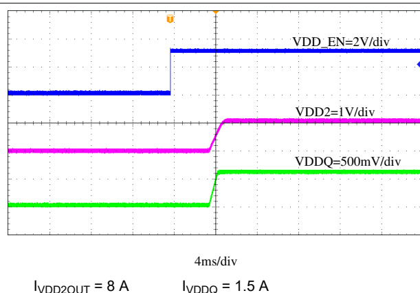
8-23. VDDQ Start-Up Through VDD_EN
