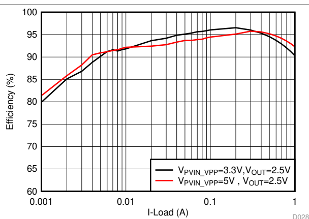
Figure 33. VPP Efficiency Curve, V_{OUT} = 2.5\text{ V}
