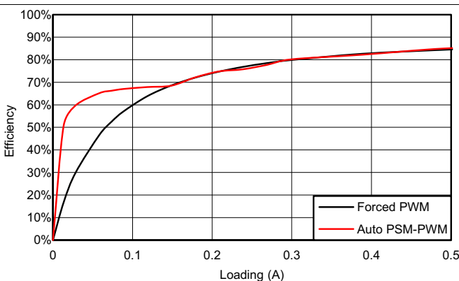
Figure 2. 0.8-V Efficiency, Light Load V_{IN} = 12\text{ V} , V_{OUT} = 0.8\text{ V}
