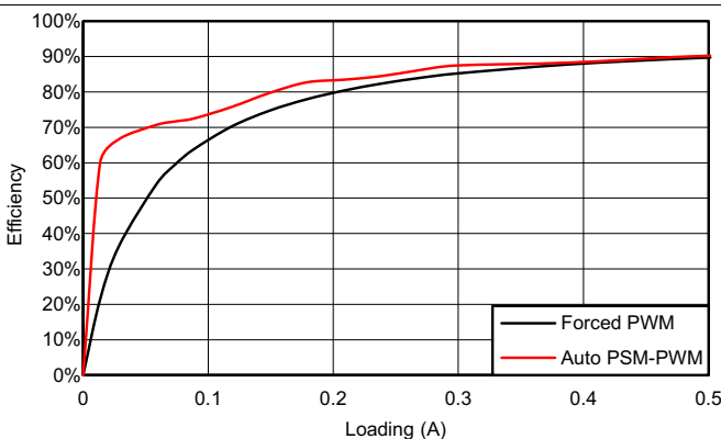
Figure 4. 1.8-V Efficiency, Light Load V_{IN} = 12\text{ V} , V_{OUT} = 1.8\text{ V}
