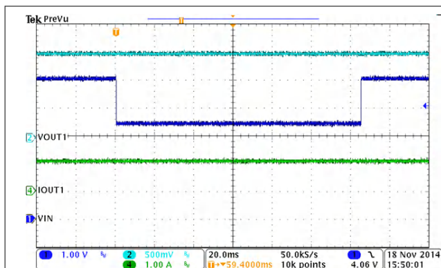
8-23. Operation at VIN Drop to 2.5 V
