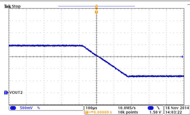
图 8-20. VID2 from 7F to 00, SR = 10 mV/Cycle
