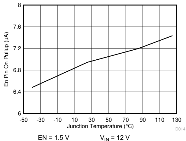
6-14. EN Pin Pullup Current vs Temperature, EN = 1.5 V
