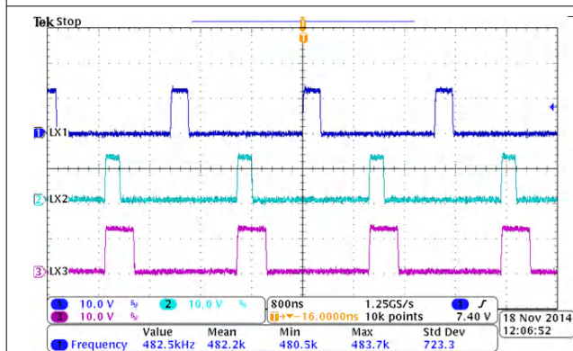
图 8-21. 180° Out-of-Phase
