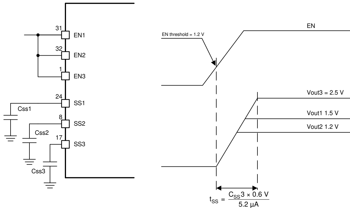
FIG 7-7. Simultaneous Start-up Sequence Using SSx Pins
