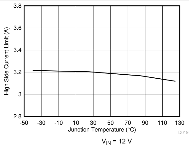
6-19. Buck2 High-Side Current Limit vs Temperature
