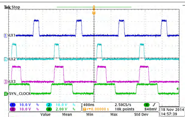
图 8-22. Synchronization With External Clock
