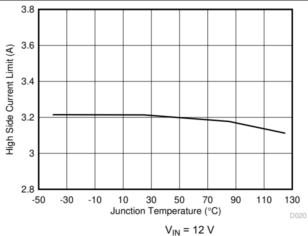
6-20. Buck3 High-Side Current Limit vs Temperature
