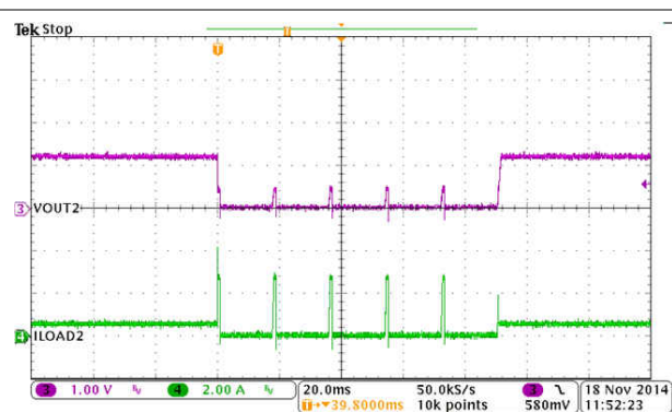
图 8-16. BUCK2, Hiccup and Recovery
