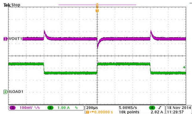
8-10. BUCK1, Load Transient
