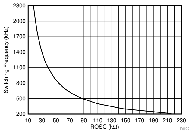
図 7-12. ROSC vs Switching Frequency
