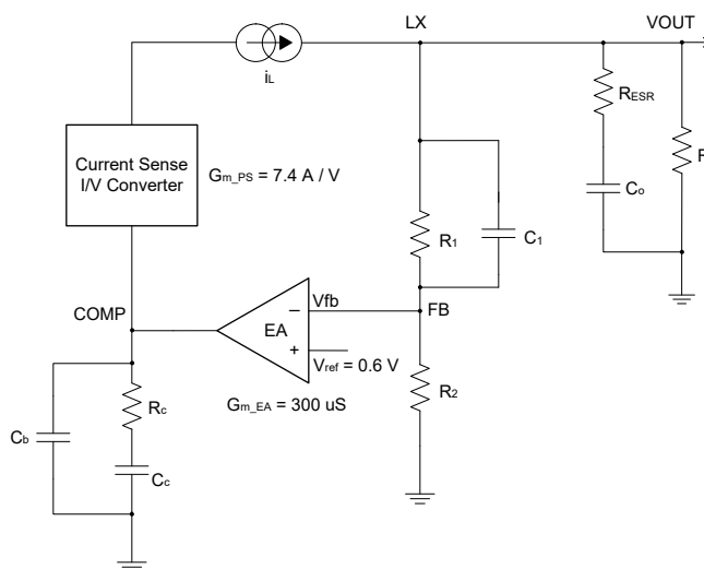
FIG 9-1. DC/DC Loop Compensation
