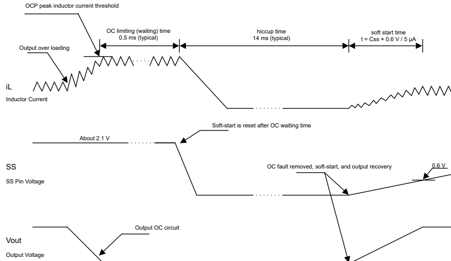
FIG 8-11. Overcurrent Protection
