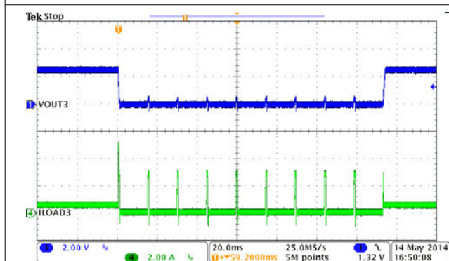
図 9-16. BUCK3, Hiccup and Recovery
