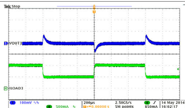
图 9-12. BUCK3, Load Transient, 0.5 to 1 A SR = 0.25 A/µs
