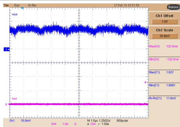
8-30. Buck 2 Ripple, No Load
