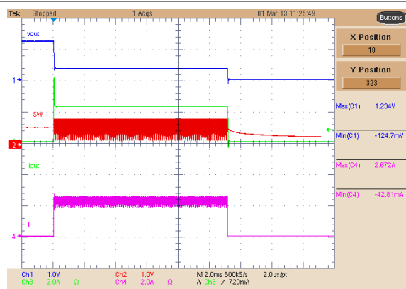
8-18. Buck 1 Current Limit Operation, Hiccup
