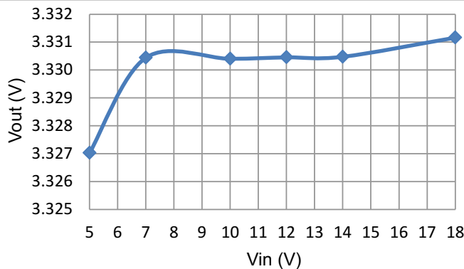
FIG 6-17. Line Regulation, Load = 1 A
