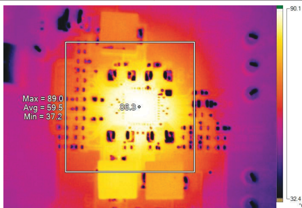
8-51. Temperature Profile, V_O = 1.2\text{ V} , I_O = 3\text{ A} , V_O = 1.8\text{ V} , I_O = 2\text{ A} , V_O = 3.3\text{ V} , I_O = 2\text{ A} , T_A = 28^\circ\text{C}
