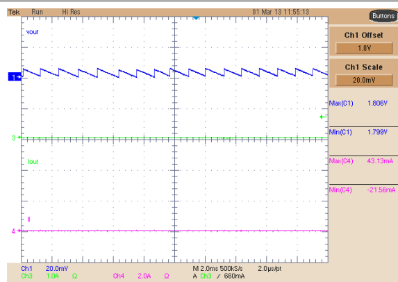
8-33. Buck 2 Low-Power Output, No Load
