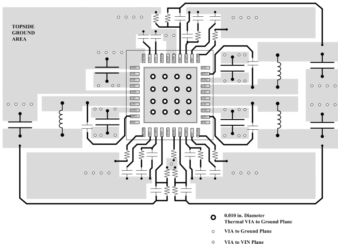
Figure 35. Layout Schematic
