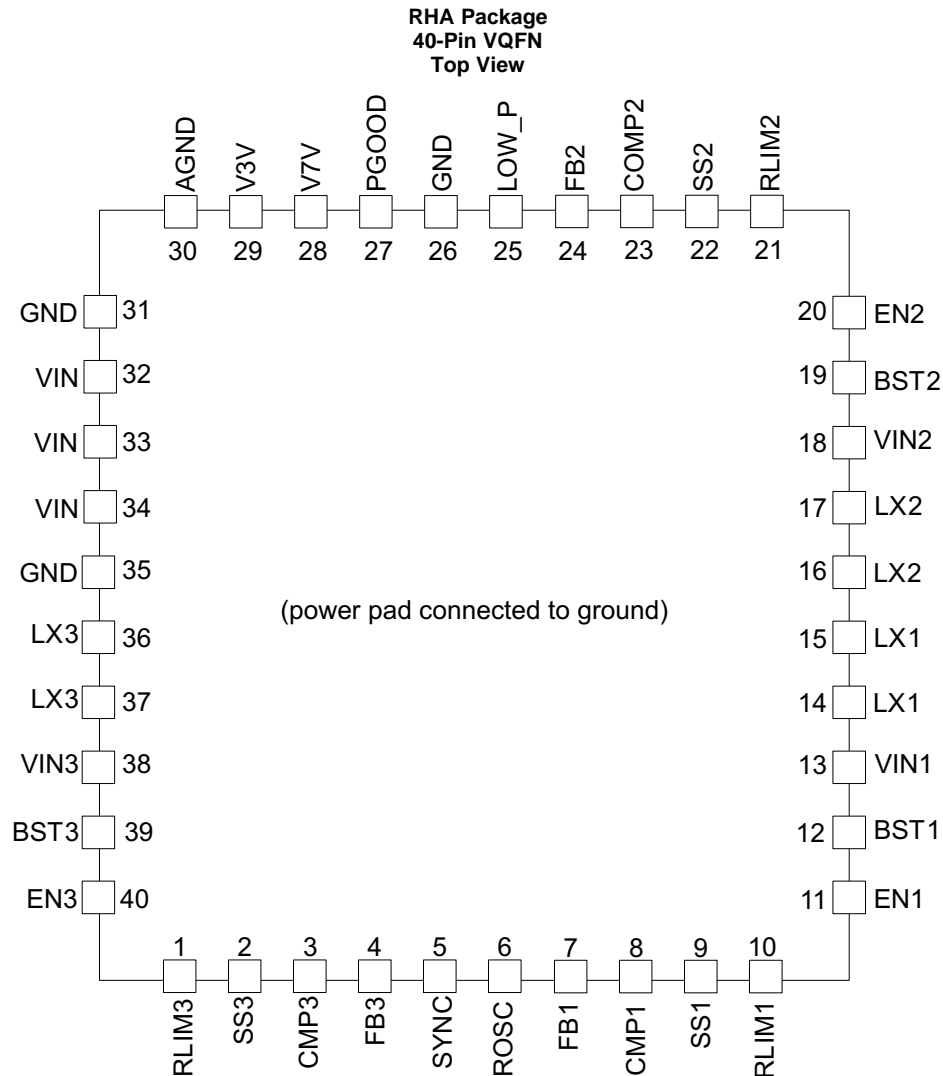
Pin Functions
